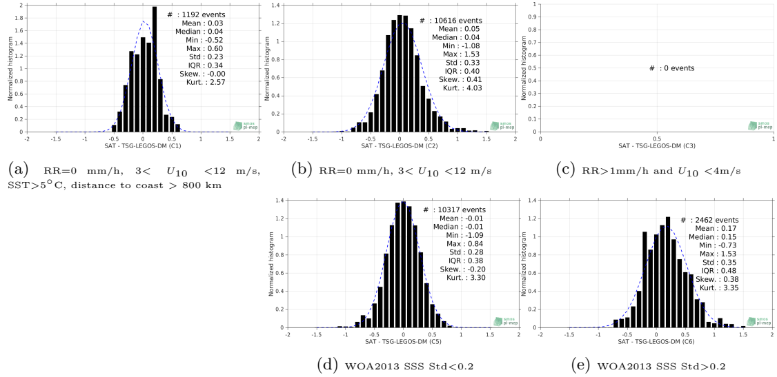
Figure 13: Normalized histogram of \Delta SSS (SMOS-L3-CATDS-CECOS-LOCEAN-V4-9DAYS-25KM - TSG-LEGOS-DM) for 5 different subdatasets corresponding to: RR=0 mm/h, 3 < U_{10} < 12 m/s, SST > 5°C, distance to coast > 800 km (a), RR=0 mm/h, 3 < U_{10} < 12 m/s (b), RR > 1mm/h and U_{10} < 4 m/s (c), WOA2013 SSS Std < 0.2 (d), WOA2013 SSS Std > 0.2 (e).
