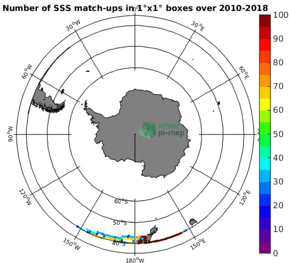
Figure 4: Number of SSS match-ups between TSG-LEGOS-DM SSS and the SMOS-L3-CATDS-CECOS-LOCEAN-V4-9DAYS-25KM SSS product for the Roaring Forties and Furious Fifties Pi-MEP region over 1^\circ \times 1^\circ boxes and for the full satellite product period.
