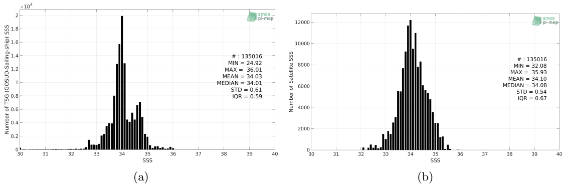
Figure 2: Histograms of SSS from TSG (GOSUD-Sailing-ship) (a) and SMOS SSS L3 v4 - 9 Days (CATDS-CECOS-LOCEAN) (b) considering all match-up pairs per bins of 0.1 over the Roaring Forties and Furious Fifties Pi-MEP region and for the full satellite product period.
