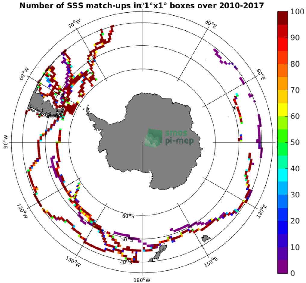
Figure 4: Number of SSS match-ups between TSG (GOSUD-Sailing-ship) SSS and the SMOS SSS L3 v4 - 9 Days (CATDS-CECOS-LOCEAN) SSS product for the Roaring Forties and Furious Fifties Pi-MEP region over 1°x1° boxes and for the full satellite product period.
