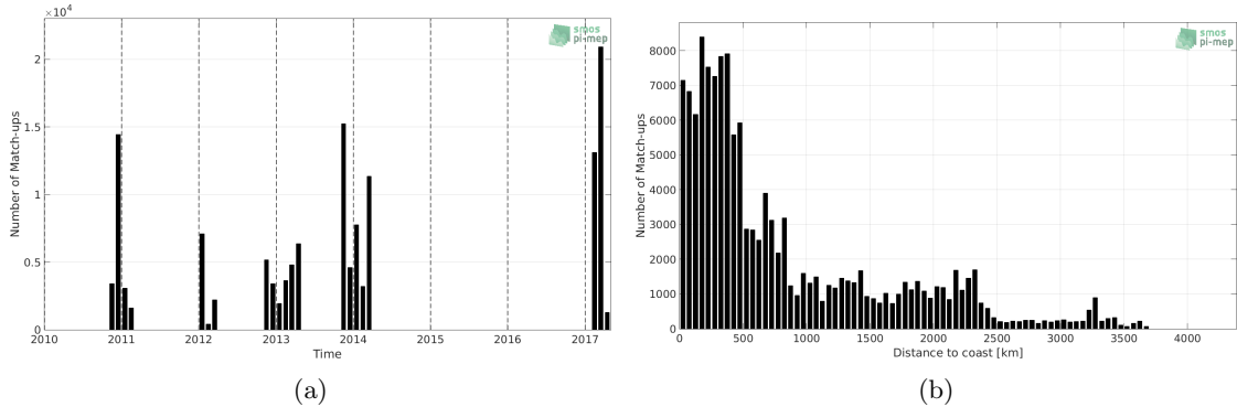
Figure 1: Number of match-ups between TSG (GOSUD-Sailing-ship) and SMOS SSS L3 v4 - 9 Days (CATDS-CECOS-LOCEAN) SSS as a function of time (a) and as function of the distance to coast (b) over the Roaring Forties and Furious Fifties Pi-MEP region and for the full satellite product period.
