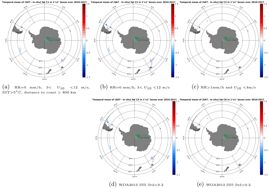
Figure 12: Temporal mean gridded over spatial boxes of size 1°x1° of \Delta SSS (SMOS SSS L3 v4 - 9 Days (CATDS-CECOS-LOCEAN) - TSG (GOSUD-Research-vessel)) for 5 different subdatasets corresponding to: RR=0 mm/h, 3 < U_{10} < 12 m/s, SST>5°C, distance to coast > 800 km (a), RR=0 mm/h, 3 < U_{10} < 12 m/s (b), RR>1mm/h and U_{10} < 4 m/s (c), WOA2013 SSS Std<0.2 (d), WOA2013 SSS Std>0.2 (e).
