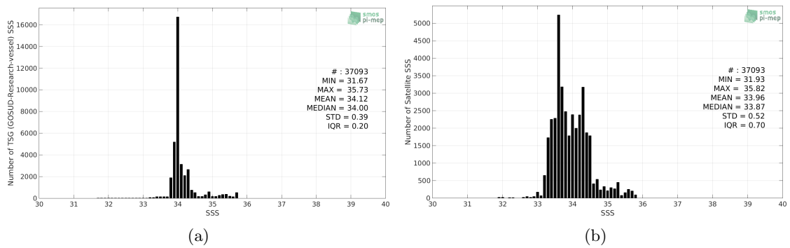
Figure 2: Histograms of SSS from TSG (GOSUD-Research-vessel) (a) and SMOS SSS L3 v4 - 9 Days (CATDS-CECOS-LOCEAN) (b) considering all match-up pairs per bins of 0.1 over the Roaring Forties and Furious Fifties Pi-MEP region and for the full satellite product period.
