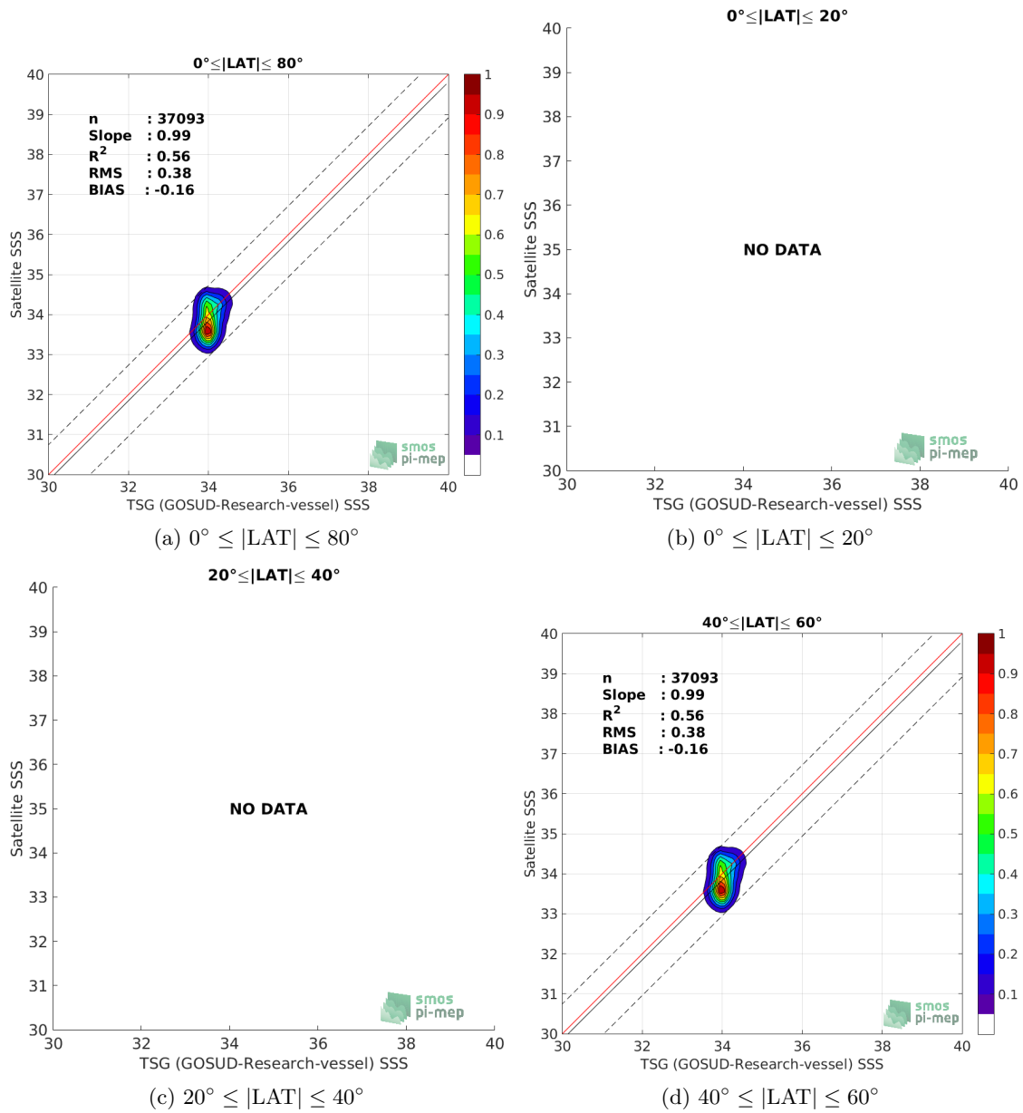
Figure 9: Contour maps of the concentration of SMOS SSS L3 v4 - 9 Days (CATDS-CECOS-LOCEAN) SSS ( y -axis) versus TSG (GOSUD-Research-vessel) SSS ( x -axis) at match-up pairs for different latitude bands. For each plot, the red line shows x=y . The black thin and dashed lines indicate a linear fit through the data cloud and the \pm 95\% confidence levels, respectively. The number match-up pairs n , the slope and R^2 coefficient of the linear fit, the root mean square (RMS) and the mean bias between satellite and in situ data are indicated for each latitude band in each plots.
