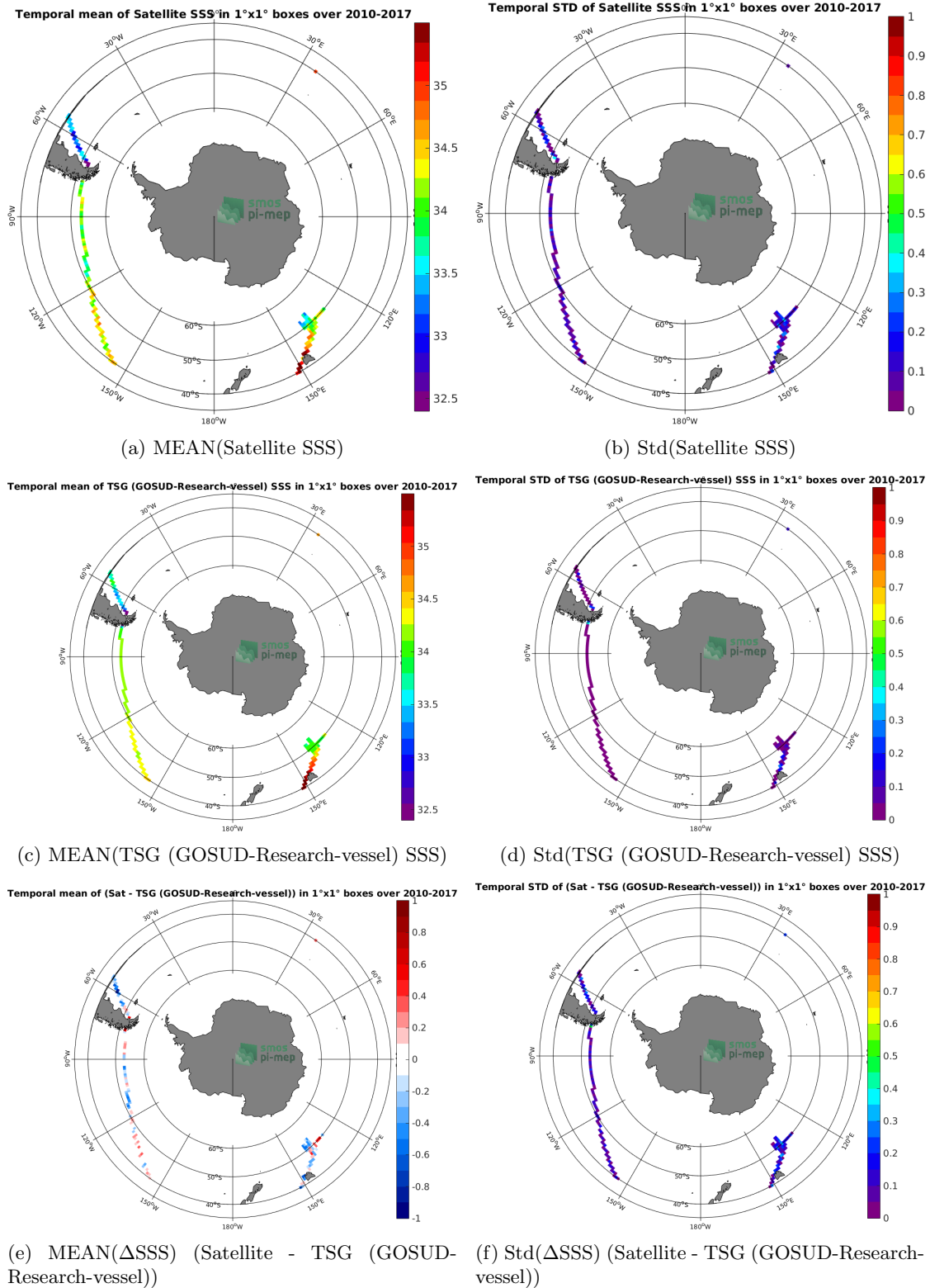
Figure 6: Temporal mean (left) and Std (right) of SSS from SMOS SSS L3 v4 - 9 Days (CATDS-CECOS-LOCEAN) (top), TSG (GOSUD-Research-vessel) (middle), and of \Delta SSS (Satellite - TSG (GOSUD-Research-vessel)). Only match-up pairs are used to generate these maps.
