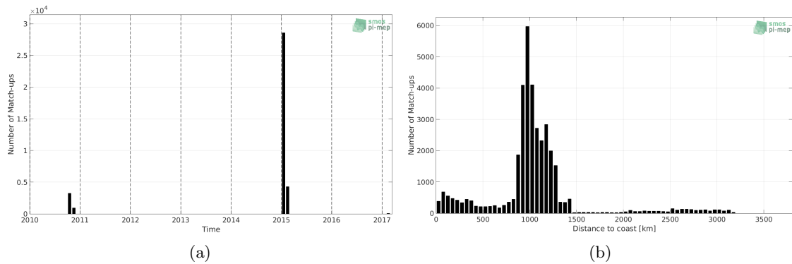
Figure 1: Number of match-ups between TSG (GOSUD-Research-vessel) and SMOS SSS L3 v4 - 9 Days (CATDS-CECOS-LOCEAN) SSS as a function of time (a) and as function of the distance to coast (b) over the Roaring Forties and Furious Fifties Pi-MEP region and for the full satellite product period.
