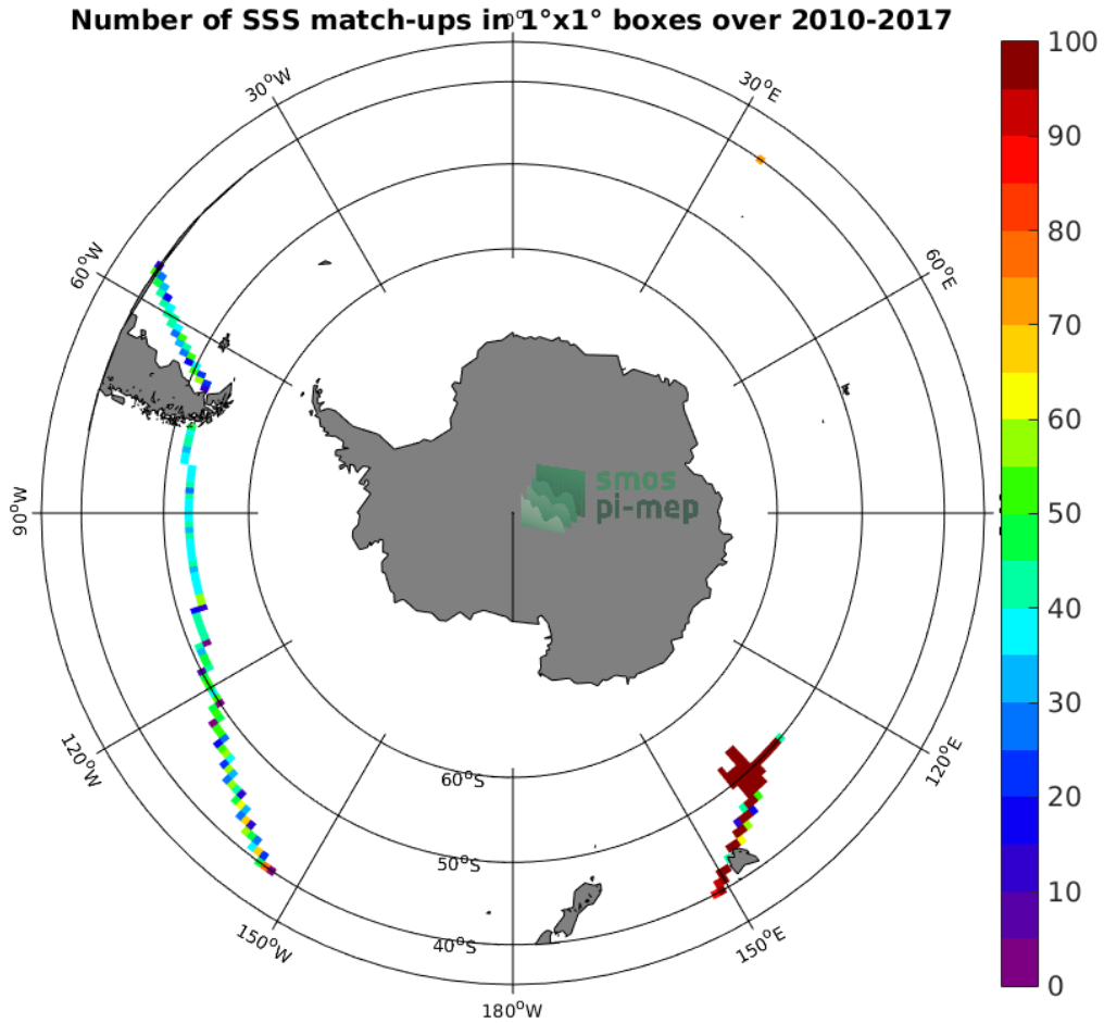
Figure 4: Number of SSS match-ups between TSG (GOSUD-Research-vessel) SSS and the SMOS SSS L3 v4 - 9 Days (CATDS-CECOS-LOCEAN) SSS product for the Roaring Forties and Furious Fifties Pi-MEP region over 1^\circ \times 1^\circ boxes and for the full satellite product period.
