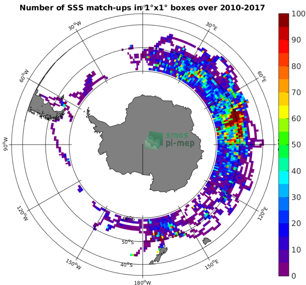
Figure 4: Number of SSS match-ups between Sea mammals SSS and the SMOS SSS L3 v4 - 9 Days (CATDS-CECOS-LOCEAN) SSS product for the Roaring Forties and Furious Fifties Pi-MEP region over 1°x1° boxes and for the full satellite product period.
