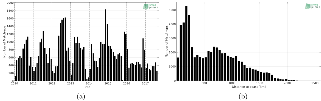
Figure 1: Number of match-ups between Sea mammals and SMOS SSS L3 v4 - 9 Days (CATDS-CECOS-LOCEAN) SSS as a function of time (a) and as function of the distance to coast (b) over the Roaring Forties and Furious Fifties Pi-MEP region and for the full satellite product period.
