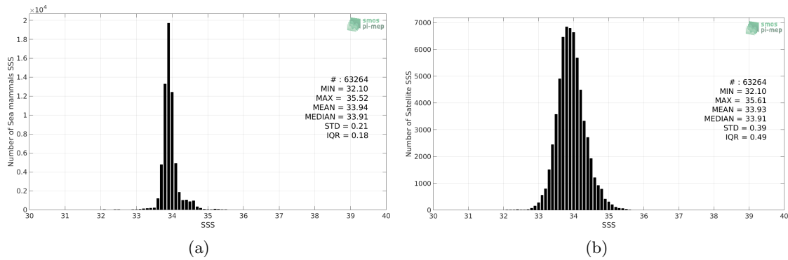
Figure 2: Histograms of SSS from Sea mammals (a) and SMOS SSS L3 v4 - 9 Days (CATDS-CECOS-LOCEAN) (b) considering all match-up pairs per bins of 0.1 over the Roaring Forties and Furious Fifties Pi-MEP region and for the full satellite product period.
