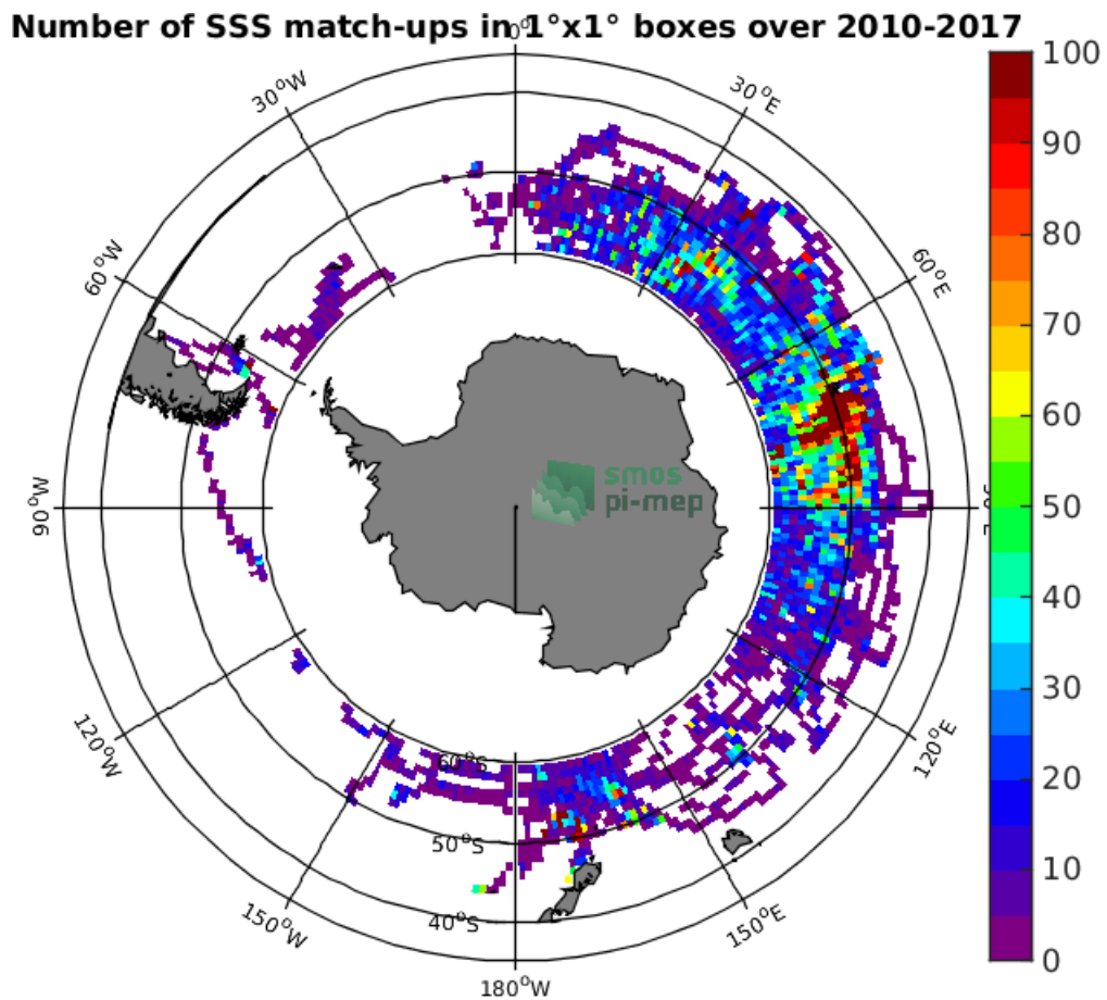
Figure 4: Number of SSS match-ups between Sea mammals SSS and the SMOS-L3-CATDS-CECOS-LOCEAN-V4-9DAYS-25KM SSS product for the Roaring Forties and Furious Fifties Pi-MEP region over 1°x1° boxes and for the full satellite product period.
