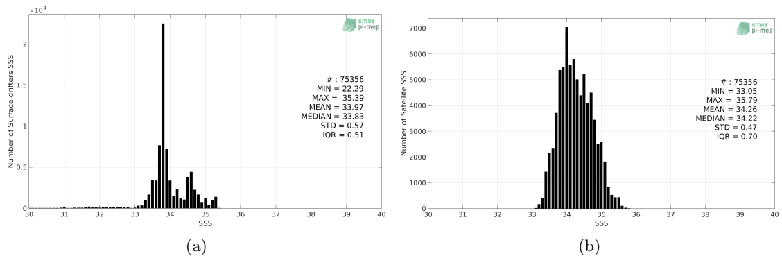
Figure 2: Histograms of SSS from Surface drifters (a) and SMOS SSS L3 v4 - 9 Days (CATDS-CECOS-LOCEAN) (b) considering all match-up pairs per bins of 0.1 over the Roaring Forties and Furious Fifties Pi-MEP region and for the full satellite product period.
