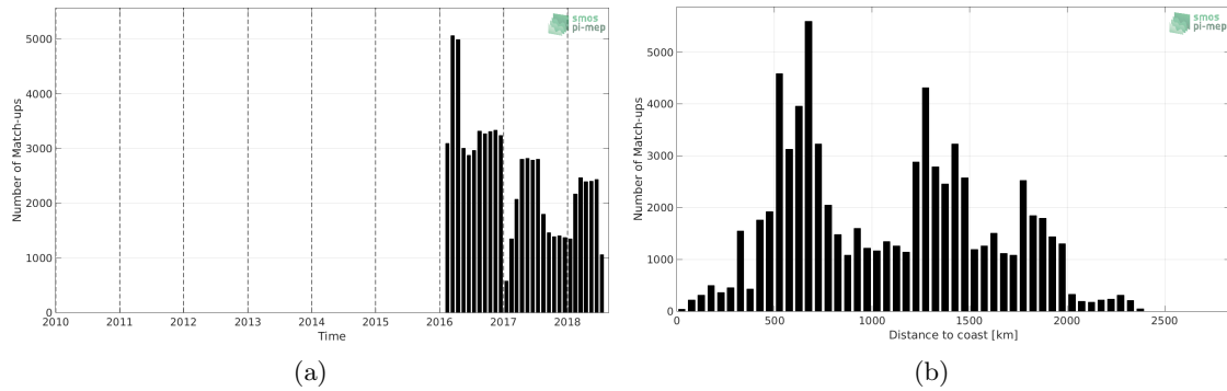
Figure 1: Number of match-ups between Surface drifters and SMOS SSS L3 v4 - 9 Days (CATDS-CECOS-LOCEAN) SSS as a function of time (a) and as function of the distance to coast (b) over the Roaring Forties and Furious Fifties Pi-MEP region and for the full satellite product period.
