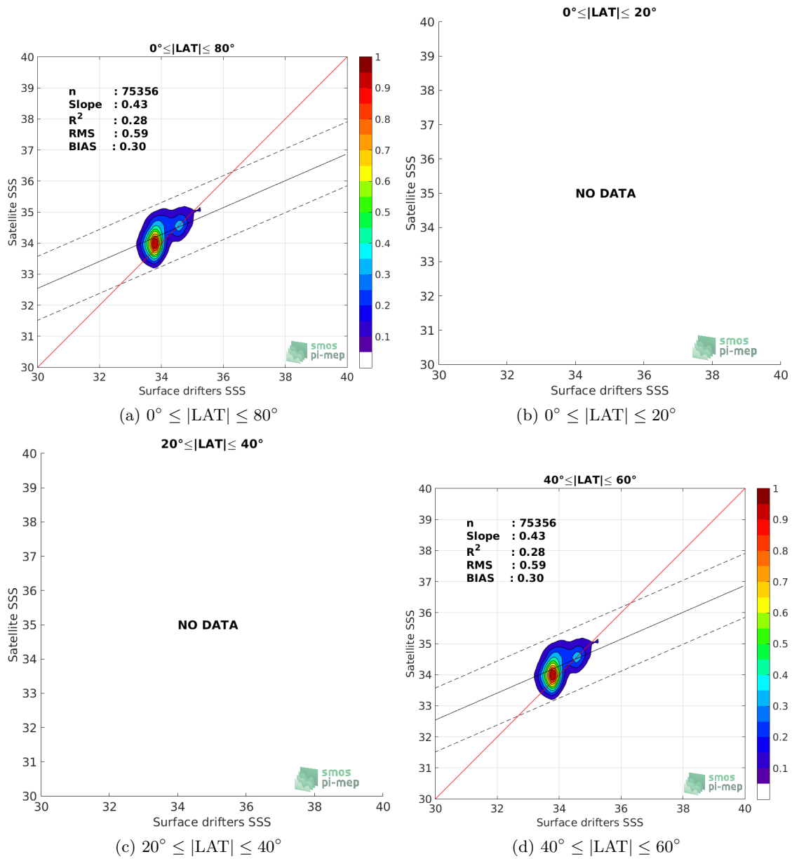
Figure 8: Contour maps of the concentration of SMOS SSS L3 v4 - 9 Days (CATDS-CECOS-LOCEAN) SSS (y-axis) versus Surface drifters SSS (x-axis) at match-up pairs for different latitude bands. For each plot, the red line shows x=y . The black thin and dashed lines indicate a linear fit through the data cloud and the \pm 95\% confidence levels, respectively. The number match-up pairs n , the slope and R^2 coefficient of the linear fit, the root mean square (RMS) and the mean bias between satellite and in situ data are indicated for each latitude band in each plots.
