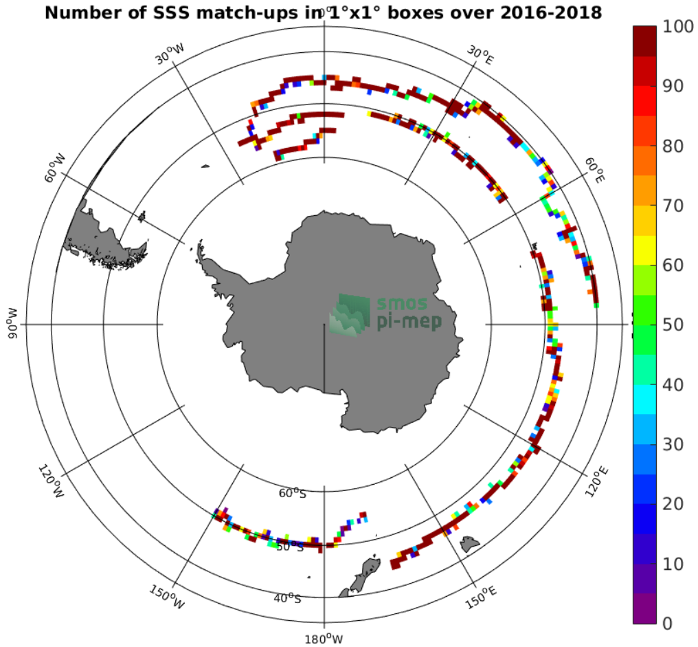
Figure 3: Number of SSS match-ups between Surface drifters SSS and the SMOS SSS L3 v4 - 9 Days (CATDS-CECOS-LOCEAN) SSS product for the Roaring Forties and Furious Fifties Pi-MEP region over 1^\circ \times 1^\circ boxes and for the full satellite product period.
