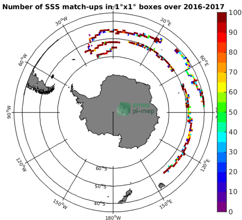
Figure 3: Number of SSS match-ups between Surface drifters SSS and the SMOS-L3-CATDS-CECOS-LOCEAN-V4-9DAYS-25KM SSS product for the Roaring Forties and Furious Fifties Pi-MEP region over 1^\circ \times 1^\circ boxes and for the full satellite product period.
