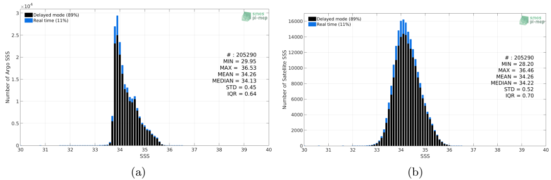
Figure 2: Histograms of SSS from Argo (a) and SMOS SSS L3 v4 - 9 Days (CATDS-CECOS-LOCEAN) (b) considering all match-up pairs per bins of 0.1 over the Roaring Forties and Furious Fifties Pi-MEP region and for the full satellite product period.
