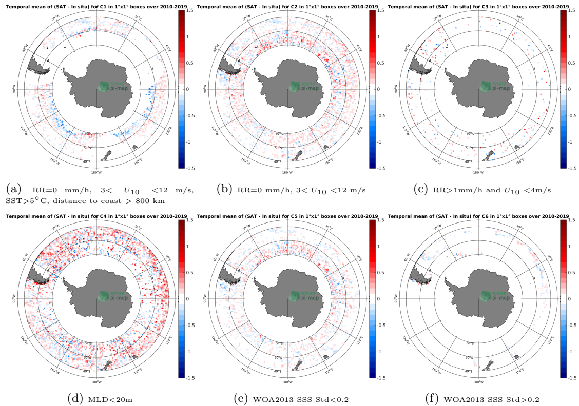
Figure 12: Temporal mean gridded over spatial boxes of size 1^{\circ}\times 1^{\circ} of \Delta\text{SSS} (SMOS SSS L3 v4 - 9 Days (CATDS-CECOS-LOCEAN) - Argo) for 6 different subdatasets corresponding to:RR=0 mm/h, 3 < U_{10} < 12 m/s, SST >5^{\circ}\text{C} , distance to coast > 800 km (a), RR=0 mm/h, 3 < U_{10} < 12 m/s (b), RR >1 mm/h and U_{10} < 4 m/s (c),MLD <20 m (d),WOA2013 SSS Std <0.2 (e),WOA2013 SSS Std >0.2 (f).
