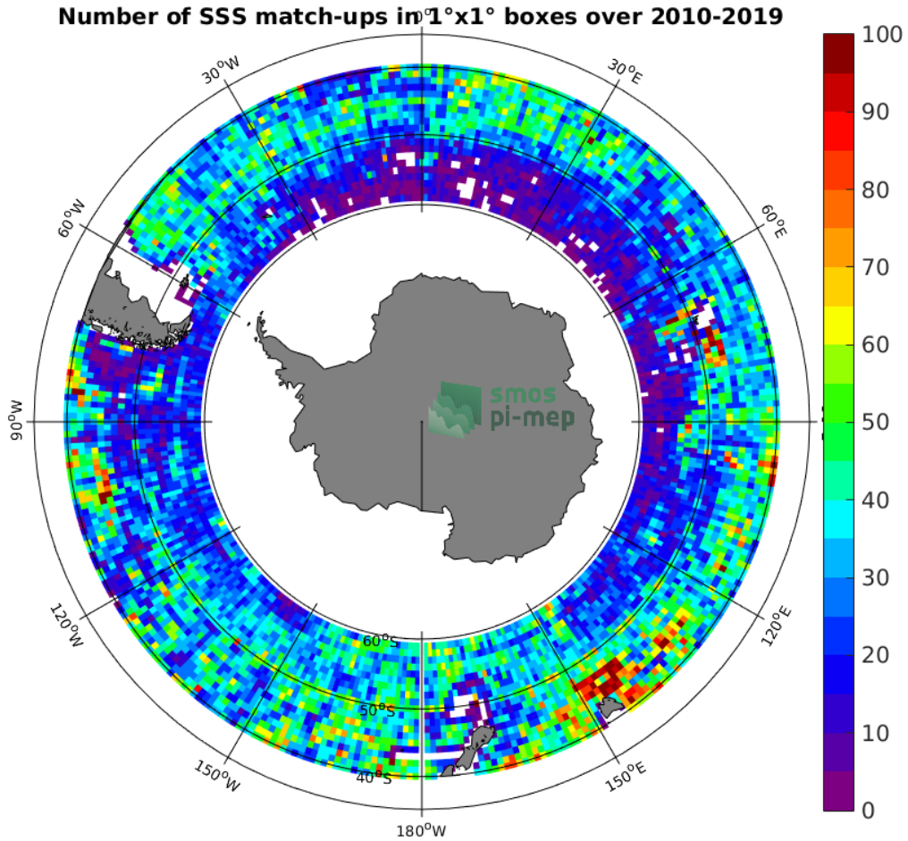
Figure 4: Number of SSS match-ups between Argo SSS and the SMOS SSS L3 v4 - 9 Days (CATDS-CECOS-LOCEAN) SSS product for the Roaring Forties and Furious Fifties Pi-MEP region over 1°x1° boxes and for the full satellite product period.
