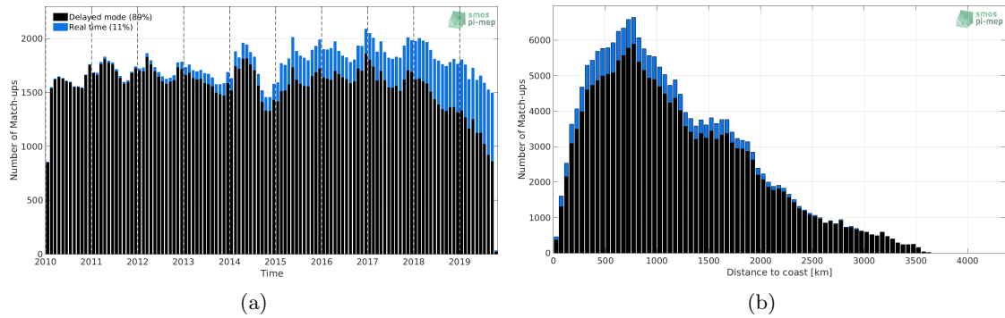
Figure 1: Number of match-ups between Argo and SMOS SSS L3 v4 - 9 Days (CATDS-CECOS-LOCEAN) SSS as a function of time (a) and as function of the distance to coast (b) over the Roaring Forties and Furious Fifties Pi-MEP region and for the full satellite product period.
