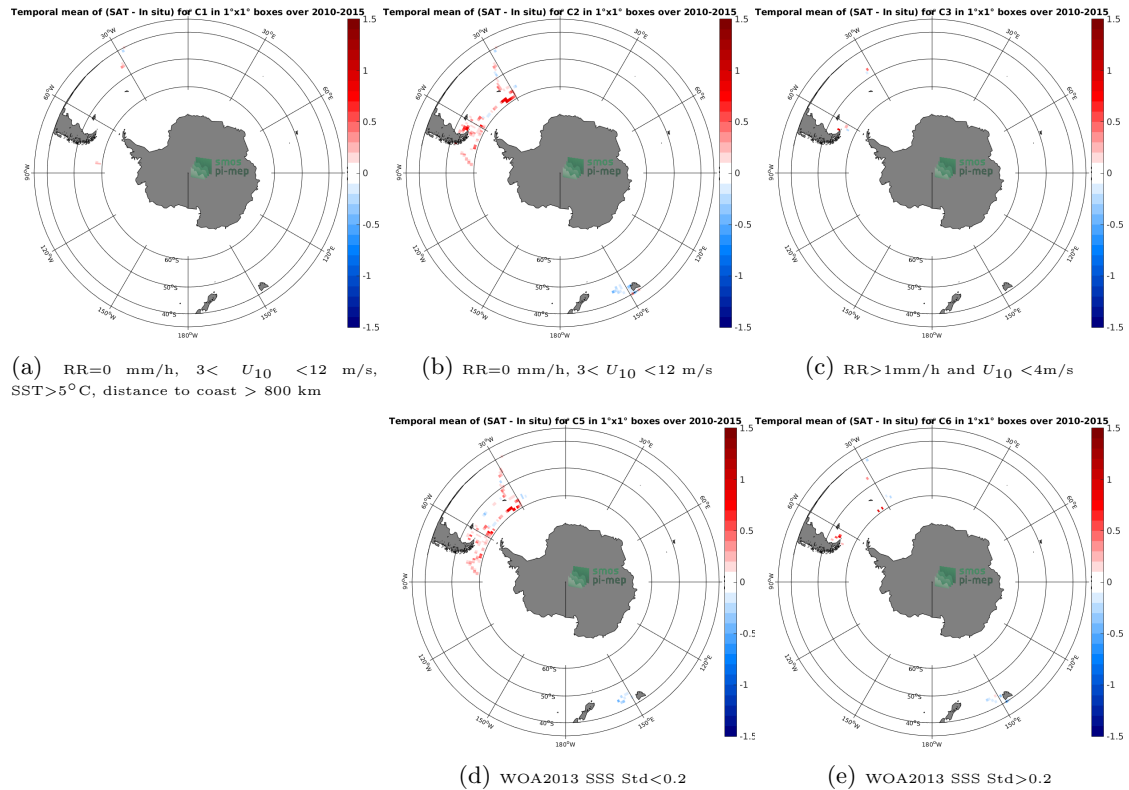
Figure 12: Temporal mean gridded over spatial boxes of size 1^{\circ}\times 1^{\circ} of \Delta\text{SSS} (SMOS SSS L3 v4 - 18 Days (CATDS-CECOS-LOCEAN) - TSG (SAMOS)) for 5 different subdatasets corresponding to: RR=0 mm/h, 3 < U_{10} < 12 m/s, SST >5^{\circ}\text{C} , distance to coast > 800 km (a), RR=0 mm/h, 3 < U_{10} < 12 m/s (b), RR >1 mm/h and U_{10} < 4 m/s (c), WOA2013 SSS Std <0.2 (d), WOA2013 SSS Std >0.2 (e).
