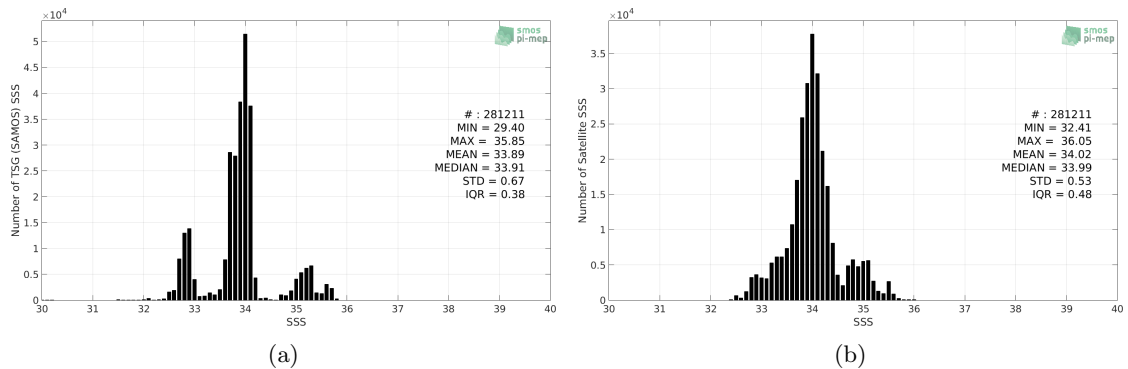
Figure 2: Histograms of SSS from TSG (SAMOS) (a) and SMOS SSS L3 v4 - 18 Days (CATDS-CECOS-LOCEAN) (b) considering all match-up pairs per bins of 0.1 over the Roaring Forties and Furious Fifties Pi-MEP region and for the full satellite product period.
