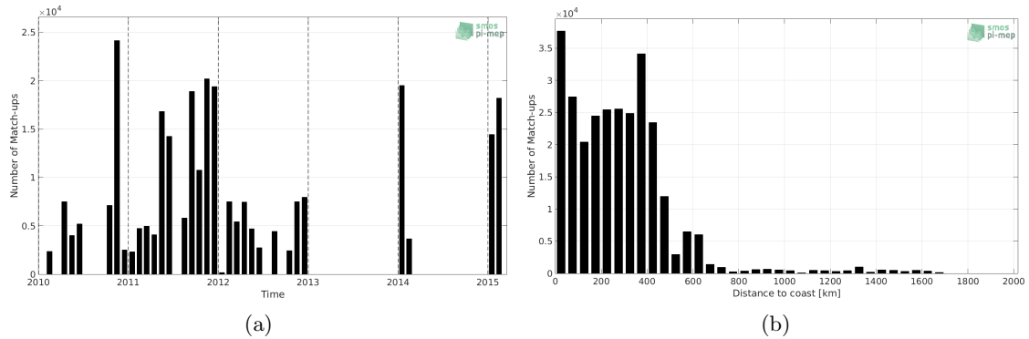
Figure 1: Number of match-ups between TSG (SAMOS) and SMOS SSS L3 v4 - 18 Days (CATDS-CECOS-LOCEAN) SSS as a function of time (a) and as function of the distance to coast (b) over the Roaring Forties and Furious Fifties Pi-MEP region and for the full satellite product period.
