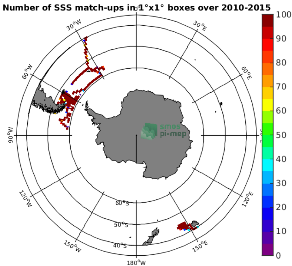
Figure 4: Number of SSS match-ups between TSG-SAMOS SSS and the SMOS-L3-CATDS-CECOS-LOCEAN-V4-18DAYS-25KM SSS product for the Roaring Forties and Furious Fifties Pi-MEP region over 1^\circ \times 1^\circ boxes and for the full satellite product period.
