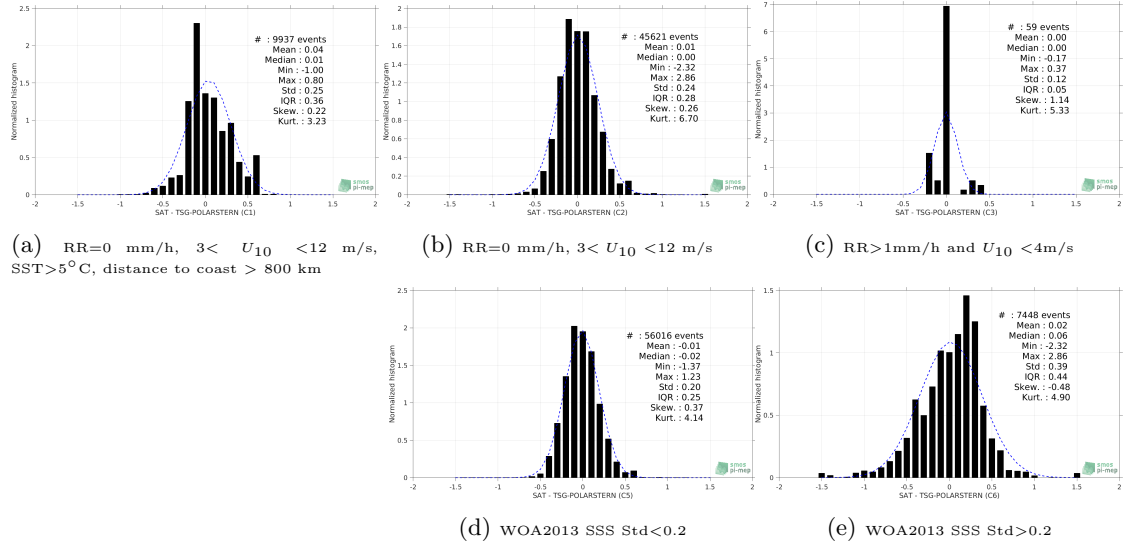
Figure 13: Normalized histogram of \Delta SSS (SMOS-L3-CATDS-CECOS-LOCEAN-V4-18DAYS-25KM - TSG-POLARSTERN) for 5 different subdatasets corresponding to: RR=0 mm/h, 3 < U_{10} < 12 m/s, SST > 5^\circ C , distance to coast > 800 km (a), RR=0 mm/h, 3 < U_{10} < 12 m/s (b), RR > 1 mm/h and U_{10} < 4 m/s (c), WOA2013 SSS Std < 0.2 (d), WOA2013 SSS Std > 0.2 (e).
