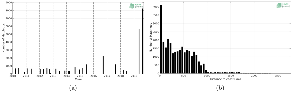
Figure 1: Number of match-ups between TSG (LEGOS-DM) and SMOS SSS L3 v4 - 18 Days (CATDS-CECOS-LOCEAN) SSS as a function of time (a) and as function of the distance to coast (b) over the Roaring Forties and Furious Fifties Pi-MEP region and for the full satellite product period.
