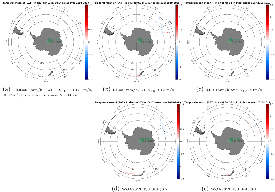
Figure 12: Temporal mean gridded over spatial boxes of size 1^{\circ}\times 1^{\circ} of \Delta\text{SSS} (SMOS SSS L3 v4 - 18 Days (CATDS-CECOS-LOCEAN) - TSG (LEGOS-DM)) for 5 different subdatasets corresponding to:RR=0 mm/h, 3 < U_{10} < 12 m/s, SST >5^{\circ}\text{C} , distance to coast > 800 km (a), RR=0 mm/h, 3 < U_{10} < 12 m/s (b), RR >1 mm/h and U_{10} < 4 m/s (c), WOA2013 SSS Std <0.2 (d), WOA2013 SSS Std >0.2 (e).
