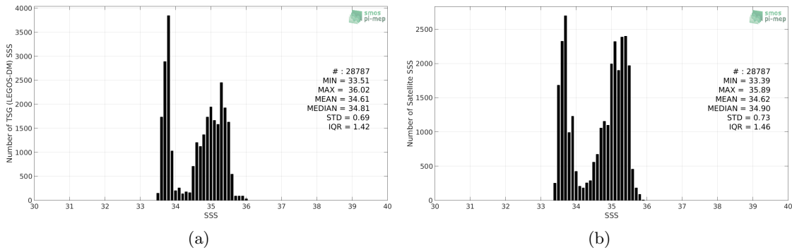
Figure 2: Histograms of SSS from TSG (LEGOS-DM) (a) and SMOS SSS L3 v4 - 18 Days (CATDS-CECOS-LOCEAN) (b) considering all match-up pairs per bins of 0.1 over the Roaring Forties and Furious Fifties Pi-MEP region and for the full satellite product period.
