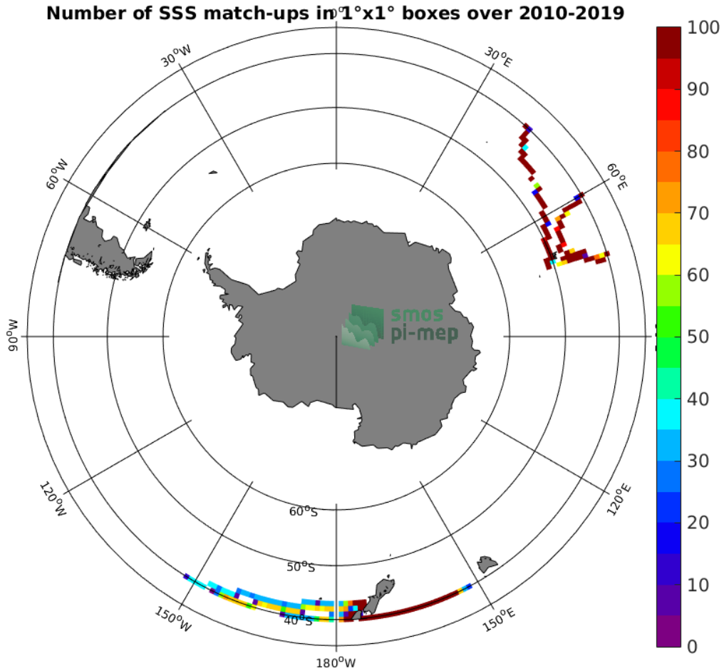
Figure 4: Number of SSS match-ups between TSG (LEGOS-DM) SSS and the SMOS SSS L3 v4 - 18 Days (CATDS-CECOS-LOCEAN) SSS product for the Roaring Forties and Furious Fifties Pi-MEP region over 1^\circ \times 1^\circ boxes and for the full satellite product period.
