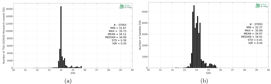
Figure 2: Histograms of SSS from TSG (GOSUD-Research-vessel) (a) and SMOS SSS L3 v4 - 18 Days (CATDS-CECOS-LOCEAN) (b) considering all match-up pairs per bins of 0.1 over the Roaring Forties and Furious Fifties Pi-MEP region and for the full satellite product period.
