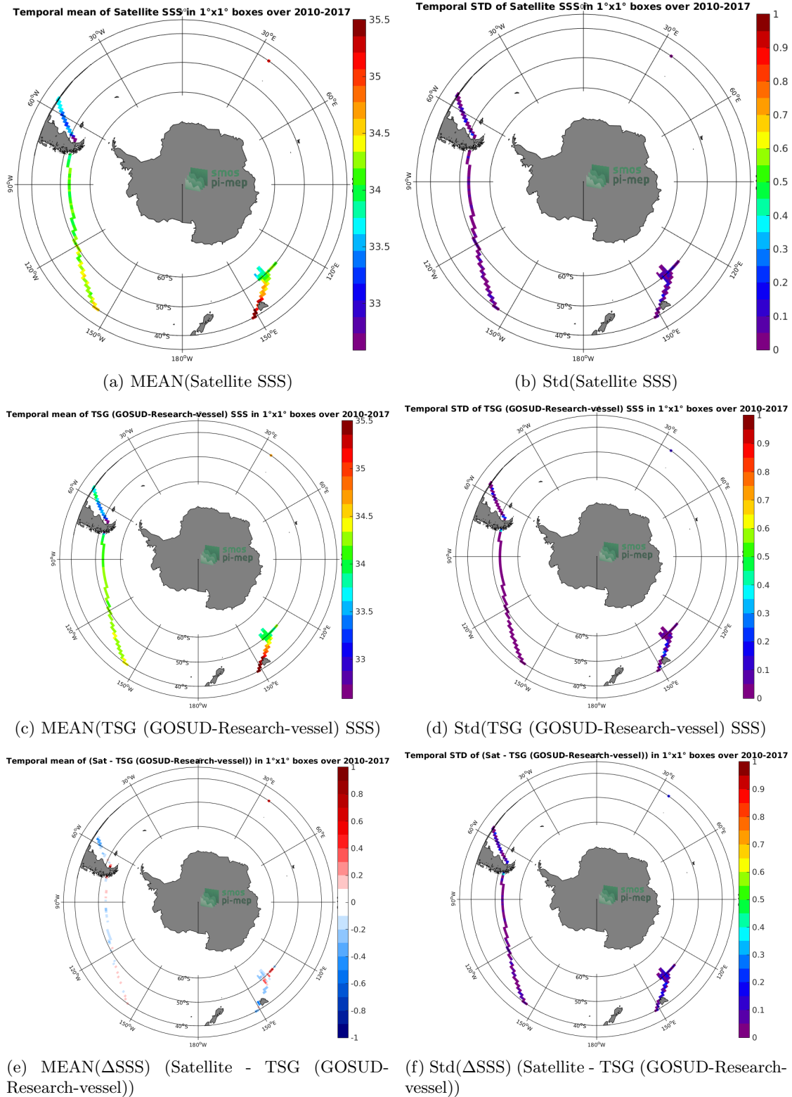
Figure 6: Temporal mean (left) and Std (right) of SSS from SMOS SSS L3 v4 - 18 Days (CATDS-CECOS-LOCEAN) (top), TSG (GOSUD-Research-vessel) (middle), and of \Delta SSS (Satellite - TSG (GOSUD-Research-vessel)). Only match-up pairs are used to generate these maps.
