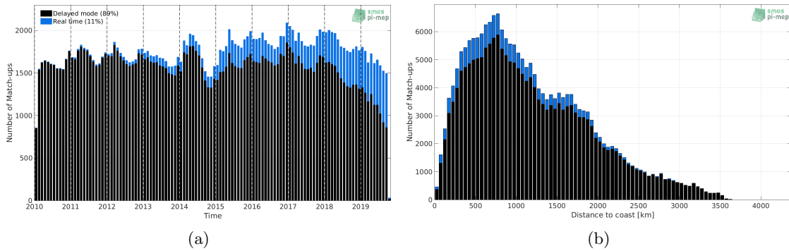
Figure 1: Number of match-ups between Argo and SMOS SSS L3 v4 - 18 Days (CATDS-CECOS-LOCEAN) SSS as a function of time (a) and as function of the distance to coast (b) over the Roaring Forties and Furious Fifties Pi-MEP region and for the full satellite product period.
