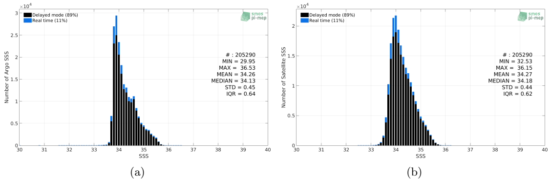
Figure 2: Histograms of SSS from Argo (a) and SMOS SSS L3 v4 - 18 Days (CATDS-CECOS-LOCEAN) (b) considering all match-up pairs per bins of 0.1 over the Roaring Forties and Furious Fifties Pi-MEP region and for the full satellite product period.
