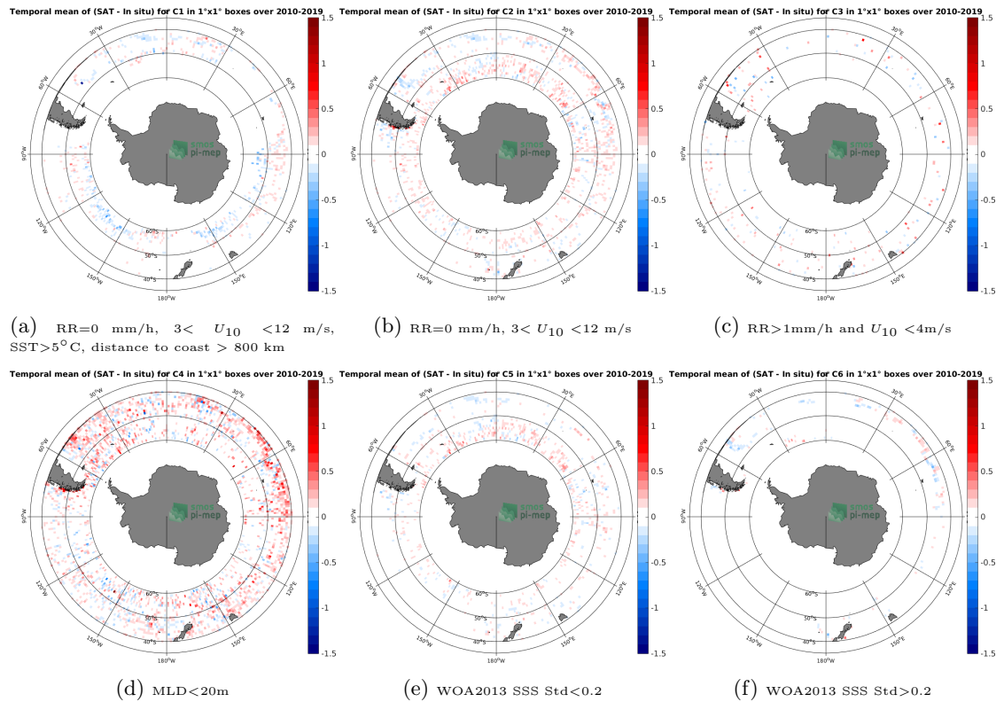
Figure 12: Temporal mean gridded over spatial boxes of size 1^{\circ}\times 1^{\circ} of \Delta\text{SSS} (SMOS SSS L3 v4 - 18 Days (CATDS-CECOS-LOCEAN) - Argo) for 6 different subdatasets corresponding to:RR=0 mm/h, 3 < U_{10} < 12 m/s, SST >5^{\circ}\text{C} , distance to coast > 800 km (a), RR=0 mm/h, 3 < U_{10} < 12 m/s (b), RR >1 mm/h and U_{10} < 4 m/s (c),MLD <20 m (d),WOA2013 SSS Std <0.2 (e),WOA2013 SSS Std >0.2 (f).
