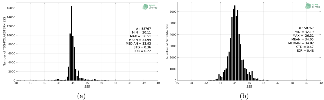
Figure 2: Histograms of SSS from TSG-POLARSTERN (a) and SMOS-L3-CATDS-CECOS-LOCEAN-V3-9DAYS-25KM (b) considering all match-up pairs per bins of 0.1 over the Roaring Forties and Furious Fifties Pi-MEP region and for the full satellite product period.
