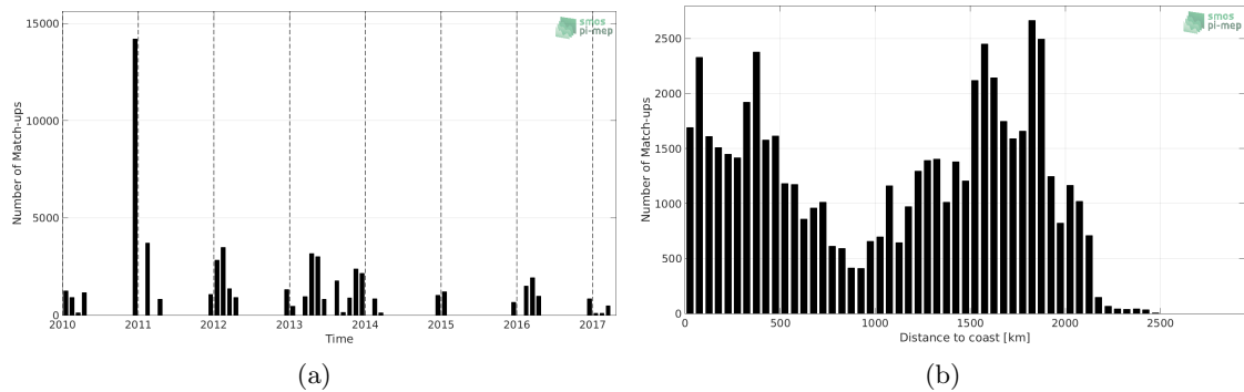
Figure 1: Number of match-ups between TSG-POLARSTERN and SMOS-L3-CATDS-CECOS-LOCEAN-V3-9DAYS-25KM SSS as a function of time (a) and as function of the distance to coast (b) over the Roaring Forties and Furious Fifties Pi-MEP region and for the full satellite product period.
