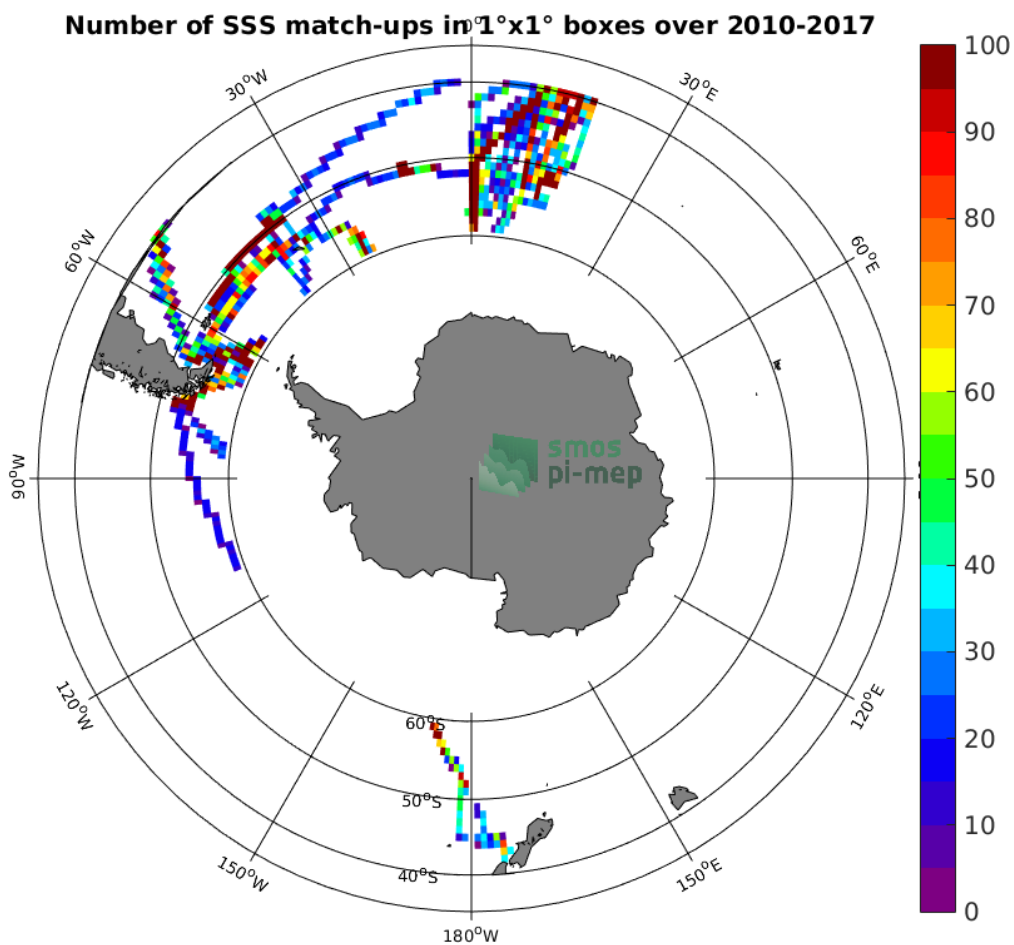
Figure 4: Number of SSS match-ups between TSG-POLARSTERN SSS and the SMOS-L3-CATDS-CECOS-LOCEAN-V3-9DAYS-25KM SSS product for the Roaring Forties and Furious Fifties Pi-MEP region over 1^{\circ} \times 1^{\circ} boxes and for the full satellite product period.
