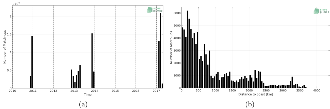
Figure 1: Number of match-ups between TSG-GOSUD-Sailing-ship and SMOS-L3-CATDS-CECOS-LOCEAN-V3-9DAYS-25KM SSS as a function of time (a) and as function of the distance to coast (b) over the Roaring Forties and Furious Fifties Pi-MEP region and for the full satellite product period.
