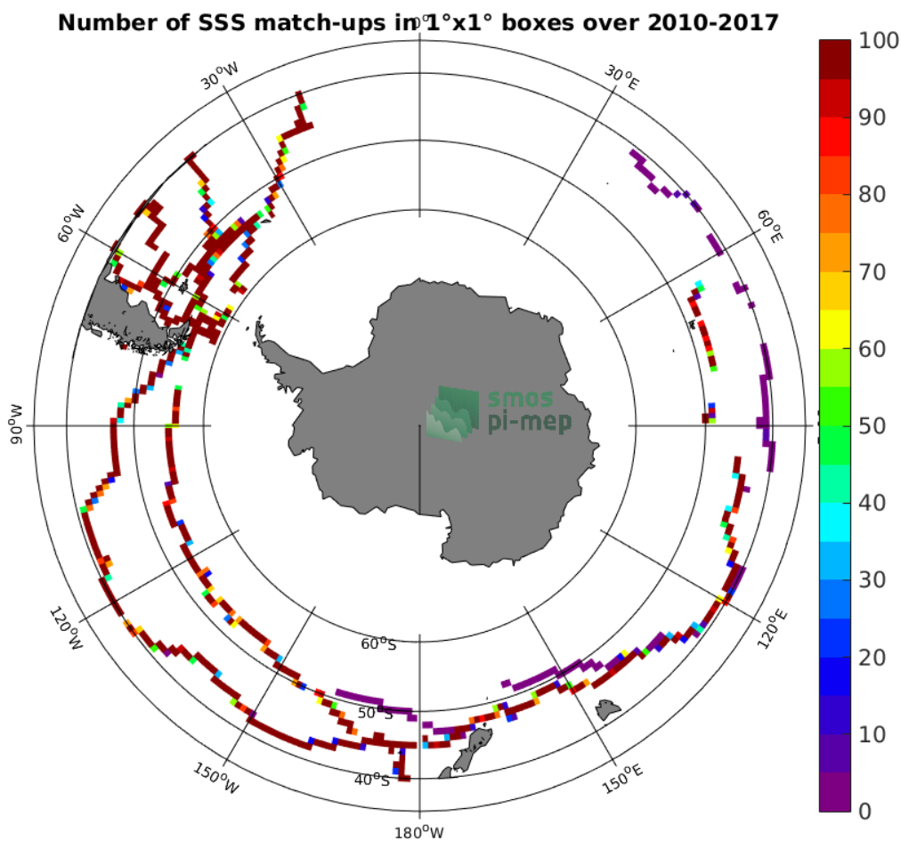
Figure 4: Number of SSS match-ups between TSG-GOSUD-Sailing-ship SSS and the SMOS-L3-CATDS-CECOS-LOCEAN-V3-9DAYS-25KM SSS product for the Roaring Forties and Furious Fifties Pi-MEP region over 1°x1° boxes and for the full satellite product period.
