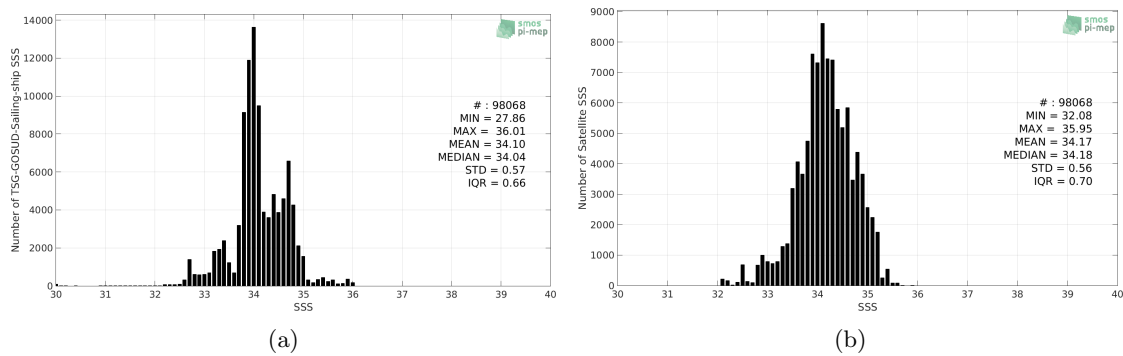
Figure 2: Histograms of SSS from TSG-GOSUD-Sailing-ship (a) and SMOS-L3-CATDS-CECOS-LOCEAN-V3-9DAYS-25KM (b) considering all match-up pairs per bins of 0.1 over the Roaring Forties and Furious Fifties Pi-MEP region and for the full satellite product period.
