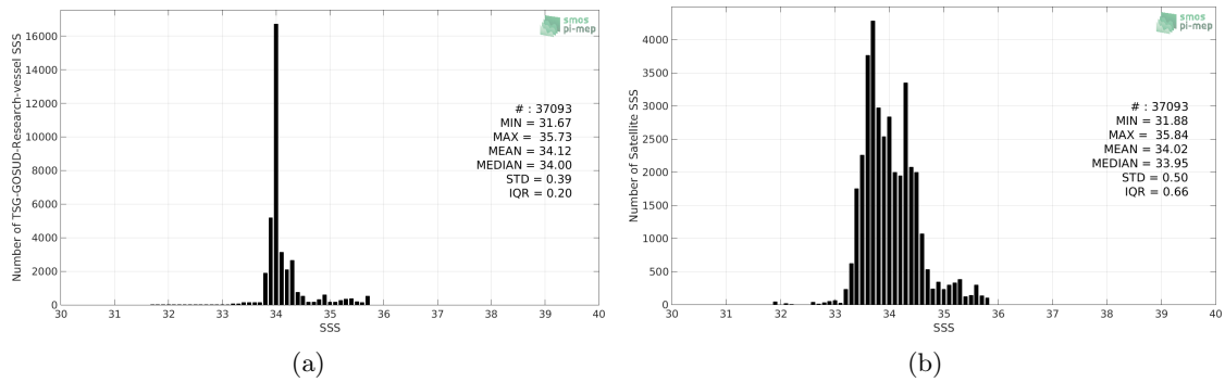
Figure 2: Histograms of SSS from TSG-GOSUD-Research-vessel (a) and SMOS-L3-CATDS-CECOS-LOCEAN-V3-9DAYS-25KM (b) considering all match-up pairs per bins of 0.1 over the Roaring Forties and Furious Fifties Pi-MEP region and for the full satellite product period.
