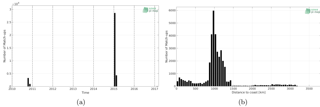
Figure 1: Number of match-ups between TSG-GOSUD-Research-vessel and SMOS-L3-CATDS-CECOS-LOCEAN-V3-9DAYS-25KM SSS as a function of time (a) and as function of the distance to coast (b) over the Roaring Forties and Furious Fifties Pi-MEP region and for the full satellite product period.
