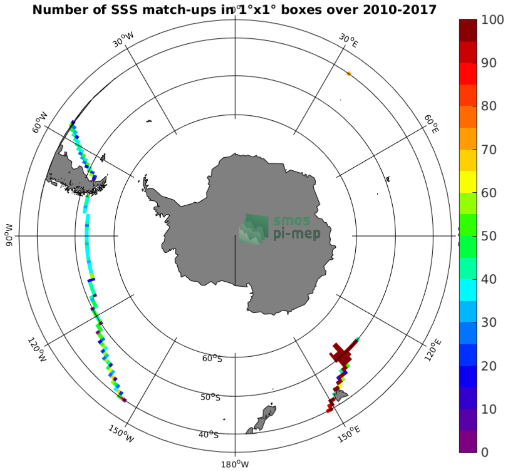
Figure 4: Number of SSS match-ups between TSG-GOSUD-Research-vessel SSS and the SMOS-L3-CATDS-CECOS-LOCEAN-V3-9DAYS-25KM SSS product for the Roaring Forties and Furious Fifties Pi-MEP region over 1°x1° boxes and for the full satellite product period.
