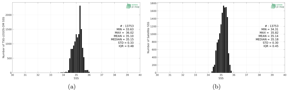
Figure 2: Histograms of SSS from TSG-LEGOS-DM (a) and SMOS-L3-CATDS-CECOS-LOCEAN-V3-18DAYS-25KM (b) considering all match-up pairs per bins of 0.1 over the Roaring Forties and Furious Fifties Pi-MEP region and for the full satellite product period.
