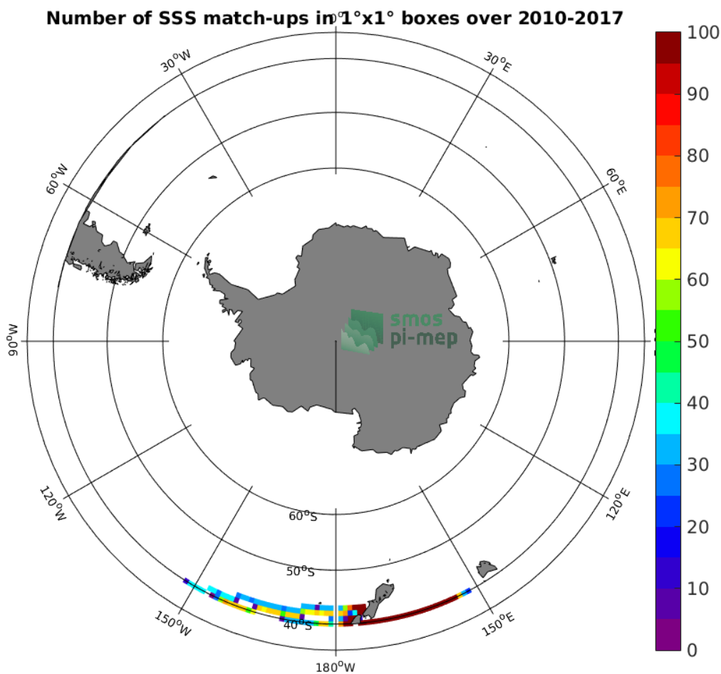
Figure 4: Number of SSS match-ups between TSG-LEGOS-DM SSS and the SMOS-L3-CATDS-CECOS-LOCEAN-V3-18DAYS-25KM SSS product for the Roaring Forties and Furious Fifties Pi-MEP region over 1°x1° boxes and for the full satellite product period.
