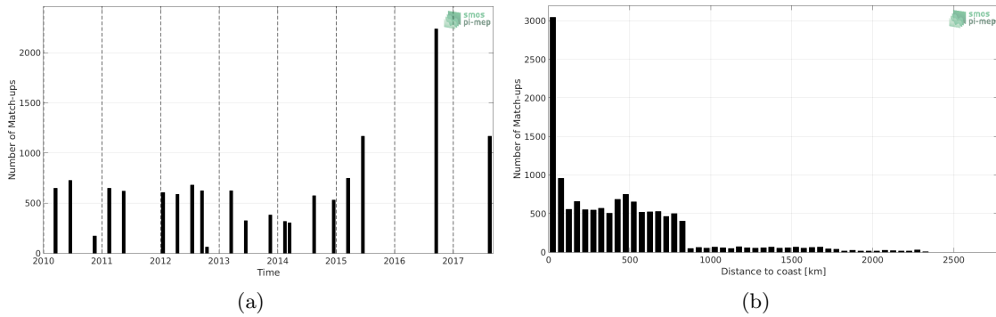
Figure 1: Number of match-ups between TSG-LEGOS-DM and SMOS-L3-CATDS-CECOS-LOCEAN-V3-18DAYS-25KM SSS as a function of time (a) and as function of the distance to coast (b) over the Roaring Forties and Furious Fifties Pi-MEP region and for the full satellite product period.
