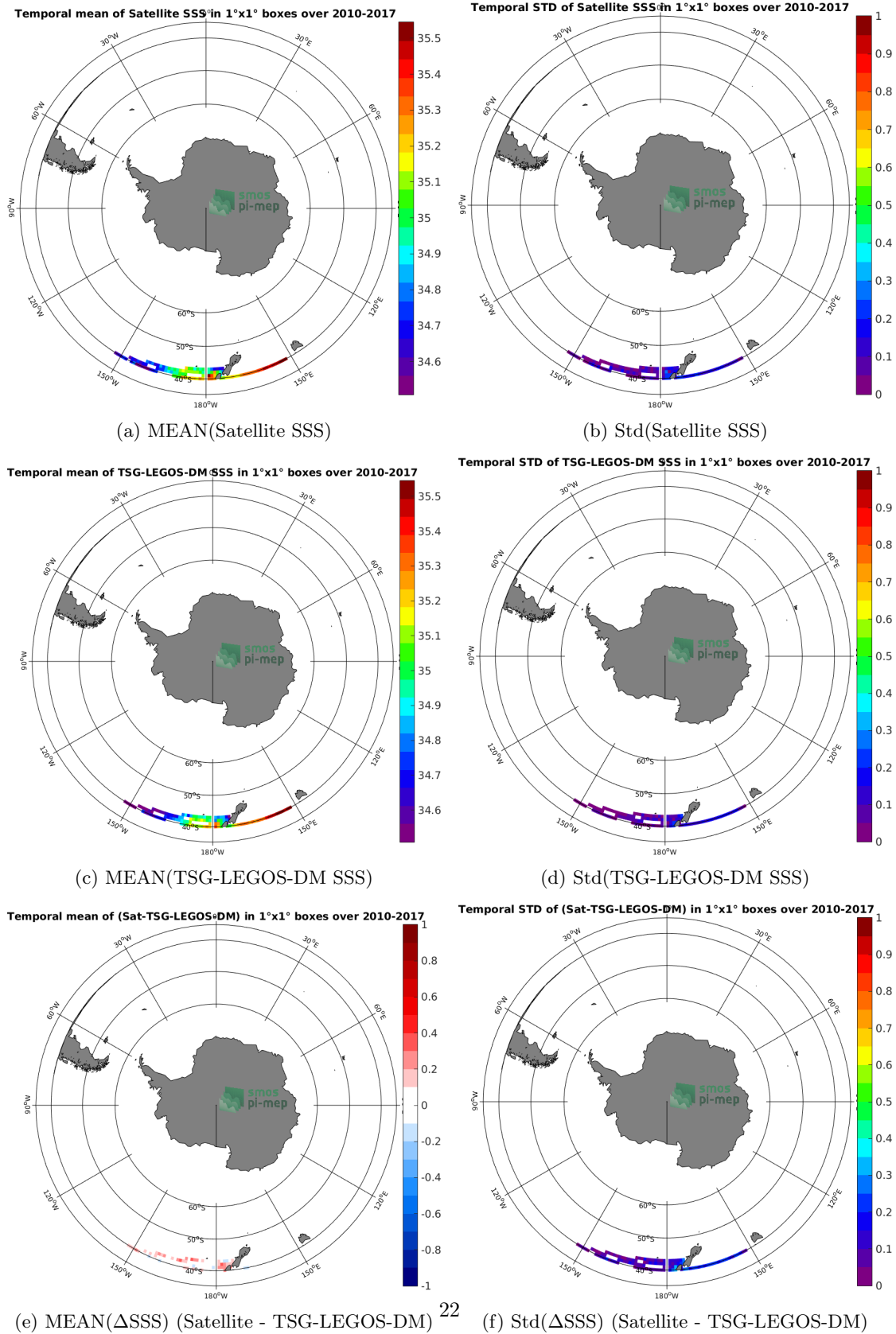
Figure 6: Temporal mean (left) and Std (right) of SSS from SMOS-L3-CATDS-CECOS-LOCEAN-V3-18DAYS-25KM (top), TSG-LEGOS-DM (middle), and of \Delta SSS (Satellite - TSG-LEGOS-DM). Only match-up pairs are used to generate these maps.
