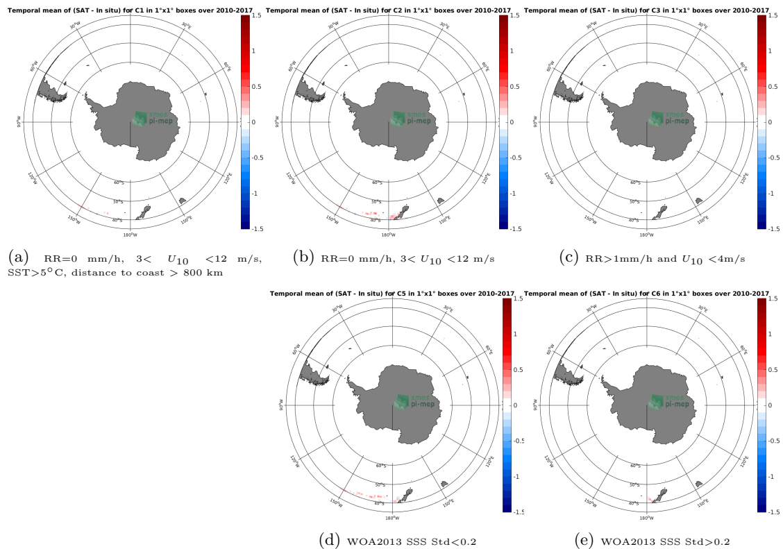
Figure 12: Temporal mean gridded over spatial boxes of size 1^\circ \times 1^\circ of \Delta SSS (SMOS-L3-CATDS-CECOS-LOCEAN-V3-18DAYS-25KM - TSG-LEGOS-DM) for 5 different subdatasets corresponding to:RR=0 mm/h, 3 < U_{10} < 12 m/s, SST >5^\circ C, distance to coast > 800 km (a), RR=0 mm/h, 3 < U_{10} < 12 m/s (b), RR >1 mm/h and U_{10} < 4 m/s (c), WOA2013 SSS Std <0.2 (d), WOA2013 SSS Std >0.2 (e).
