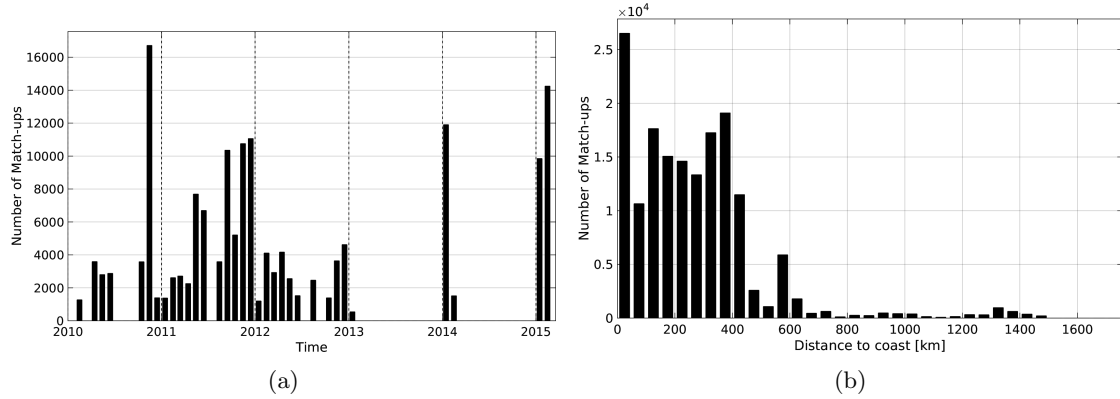
Figure 1: Number of match-ups between TSG-SAMOS and SMOS-L3-CATDS-CECOS-LOCEAN-V2.1-9DAYS-25KM SSS as a function of time (a) and as function of the distance to coast (b) over the Roaring Forties and Furious Fifties Pi-MEP region and for the full satellite product period.
