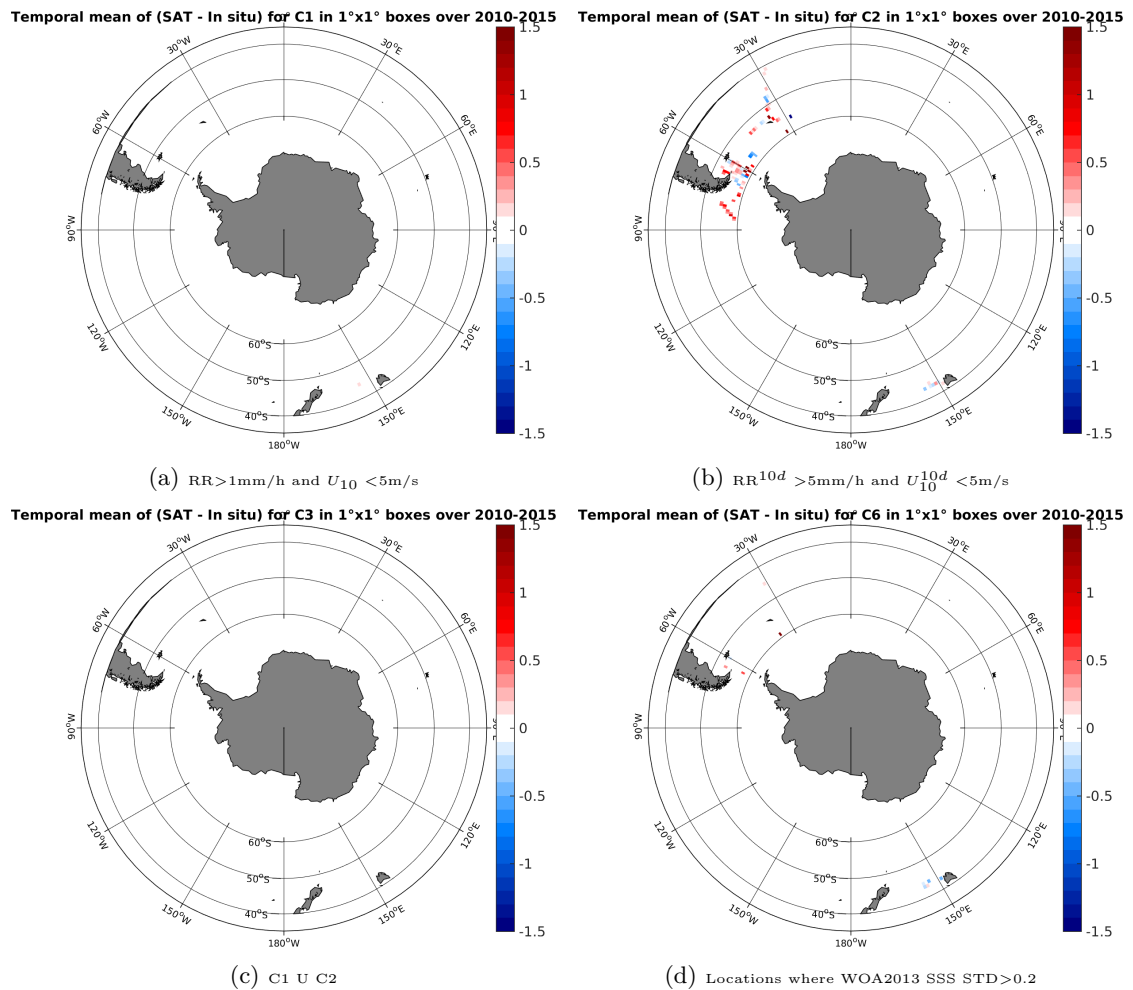
Figure 12: Temporal mean gridded over spatial boxes of size 1^\circ \times 1^\circ of \Delta SSS (SMOS-L3-CATDS-CECOS-LOCEAN-V2.1-9DAYS-25KM - TSG-SAMOS) for 4 different subdatasets corresponding to: RR > 1\text{mm/h} and U_{10} < 5\text{m/s} (a), RR^{10d} > 5\text{mm/h} and U_{10}^{10d} < 5\text{m/s} (b), C1 U C2 (c), Locations where WOA2013 SSS STD > 0.2 (d).
