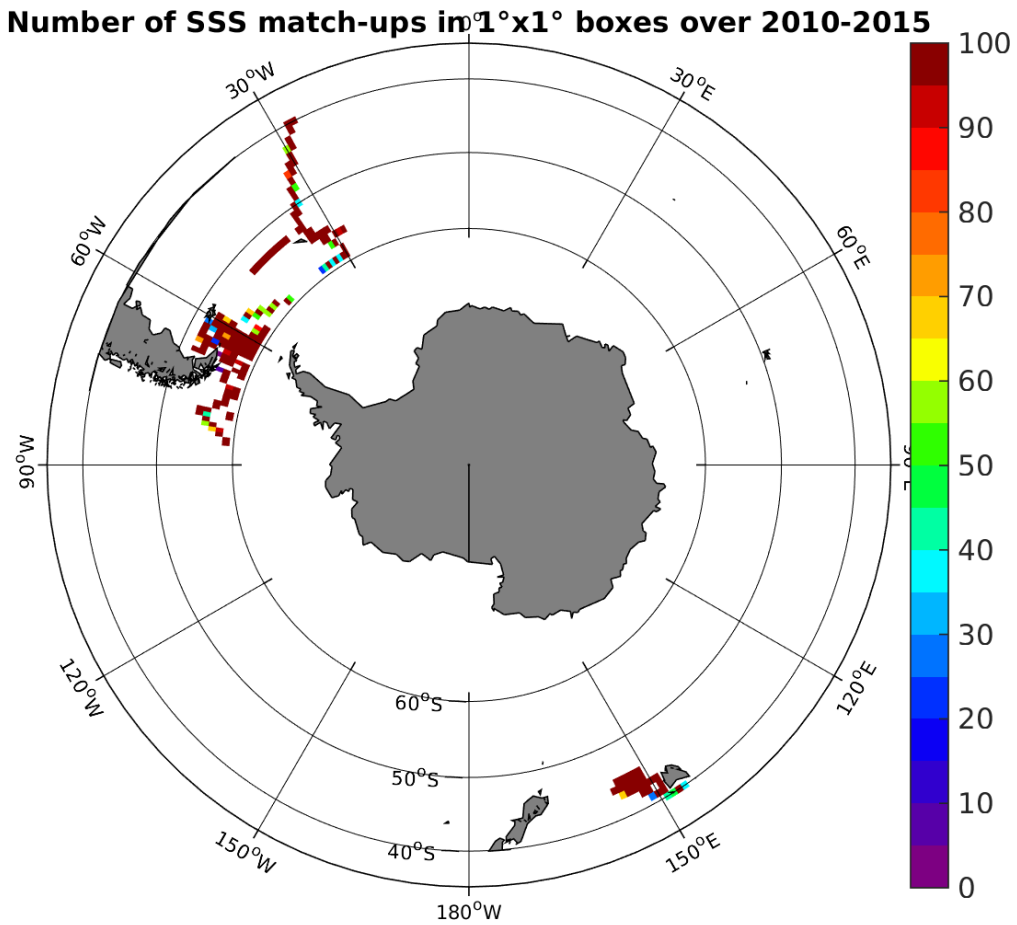
Figure 4: Number of SSS match-ups between TSG-SAMOS SSS and the SMOS-L3-CATDS-CECOS-LOCEAN-V2.1-9DAYS-25KM SSS product for the Roaring Forties and Furious Fifties Pi-MEP region over 1^\circ \times 1^\circ boxes and for the full satellite product period.
