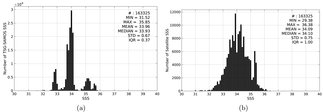
Figure 2: Histograms of SSS from TSG-SAMOS (a) and SMOS-L3-CATDS-CECOS-LOCEAN-V2.1-9DAYS-25KM (b) considering all match-up pairs per bins of 0.1 over the Roaring Forties and Furious Fifties Pi-MEP region and for the full satellite product period.
