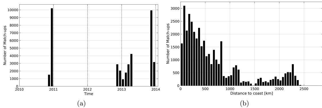
Figure 1: Number of match-ups between TSG-GOSUD-Sailing-ship and SMOS-L3-CATDS-CECOS-LOCEAN-V2.1-9DAYS-25KM SSS as a function of time (a) and as function of the distance to coast (b) over the Roaring Forties and Furious Fifties Pi-MEP region and for the full satellite product period.
