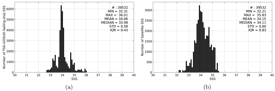
Figure 2: Histograms of SSS from TSG-GOSUD-Sailing-ship (a) and SMOS-L3-CATDS-CECOS-LOCEAN-V2.1-9DAYS-25KM (b) considering all match-up pairs per bins of 0.1 over the Roaring Forties and Furious Fifties Pi-MEP region and for the full satellite product period.
