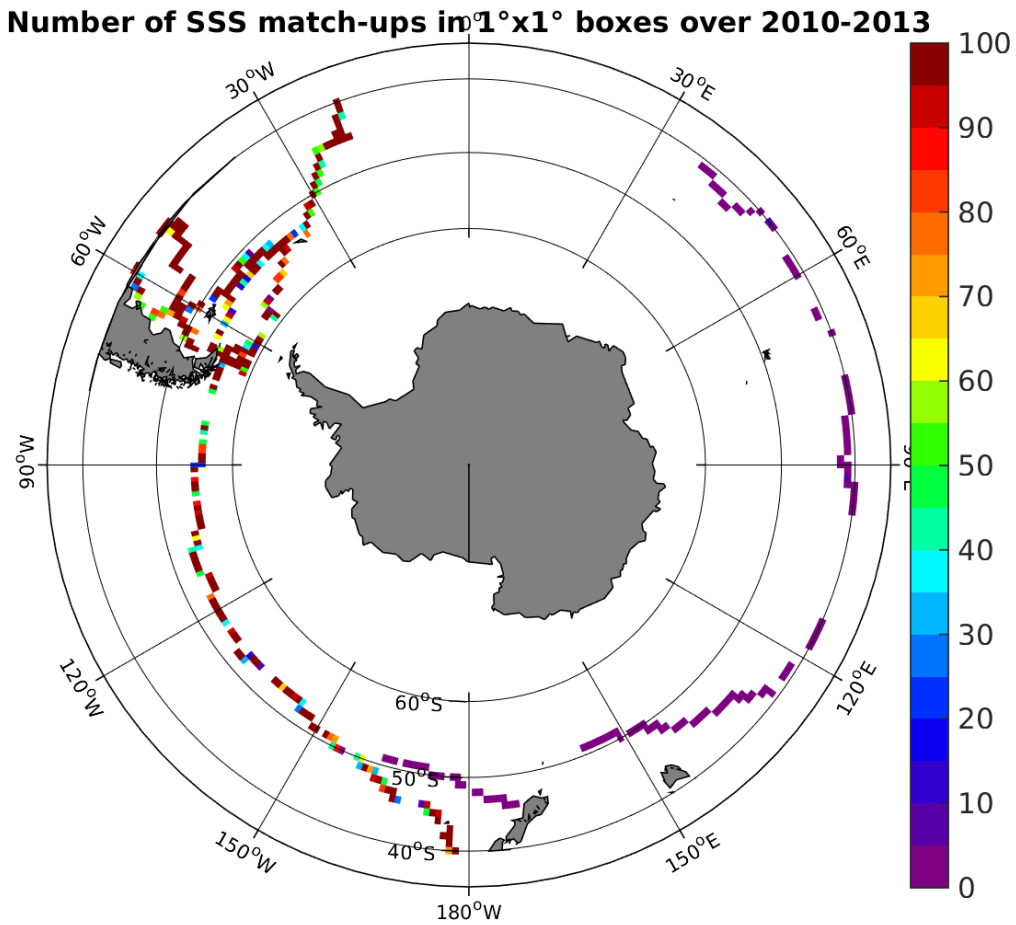
Figure 4: Number of SSS match-ups between TSG-GOSUD-Sailing-ship SSS and the SMOS-L3-CATDS-CECOS-LOCEAN-V2.1-9DAYS-25KM SSS product for the Roaring Forties and Furious Fifties Pi-MEP region over 1^\circ \times 1^\circ boxes and for the full satellite product period.
