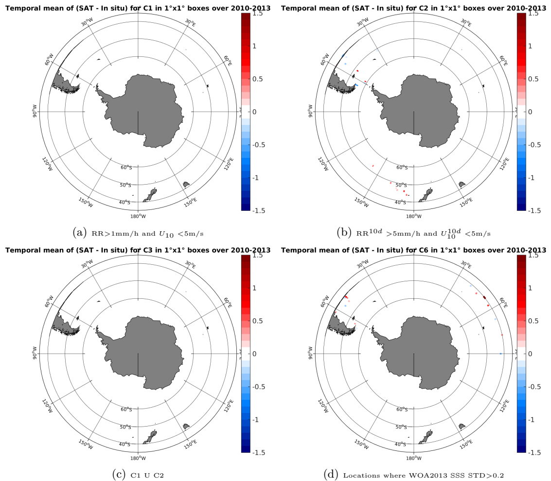
Figure 12: Temporal mean gridded over spatial boxes of size 1^\circ \times 1^\circ of \Delta SSS (SMOS-L3-CATDS-CECOS-LOCEAN-V2.1-9DAYS-25KM - TSG-GOSUD-Sailing-ship) for 4 different subdatasets corresponding to: RR > 1\text{mm/h} and U_{10} < 5\text{m/s} (a), RR^{10d} > 5\text{mm/h} and U_{10}^{10d} < 5\text{m/s} (b), C1 U C2 (c),Locations where WOA2013 SSS STD > 0.2 (d).
