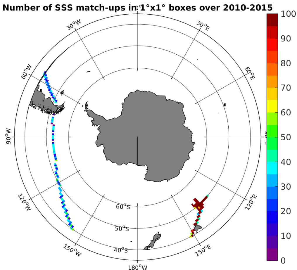
Figure 4: Number of SSS match-ups between TSG-GOSUD-Research-vessel SSS and the SMOS-L3-CATDS-CECOS-LOCEAN-V2.1-9DAYS-25KM SSS product for the Roaring Forties and Furious Fifties Pi-MEP region over 1°x1° boxes and for the full satellite product period.
