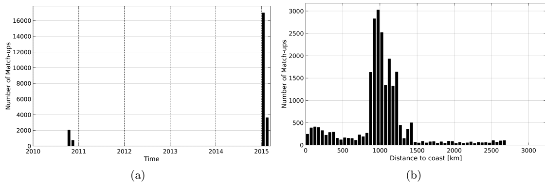
Figure 1: Number of match-ups between TSG-GOSUD-Research-vessel and SMOS-L3-CATDS-CECOS-LOCEAN-V2.1-9DAYS-25KM SSS as a function of time (a) and as function of the distance to coast (b) over the Roaring Forties and Furious Fifties Pi-MEP region and for the full satellite product period.
