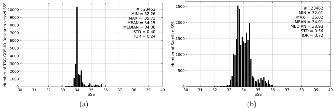
Figure 2: Histograms of SSS from TSG-GOSUD-Research-vessel (a) and SMOS-L3-CATDS-CECOS-LOCEAN-V2.1-9DAYS-25KM (b) considering all match-up pairs per bins of 0.1 over the Roaring Forties and Furious Fifties Pi-MEP region and for the full satellite product period.
