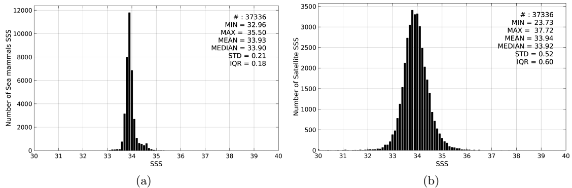
Figure 2: Histograms of SSS from Sea mammals (a) and SMOS-L3-CATDS-CECOS-LOCEAN-V2.1-9DAYS-25KM (b) considering all match-up pairs per bins of 0.1 over the Roaring Forties and Furious Fifties Pi-MEP region and for the full satellite product period.
