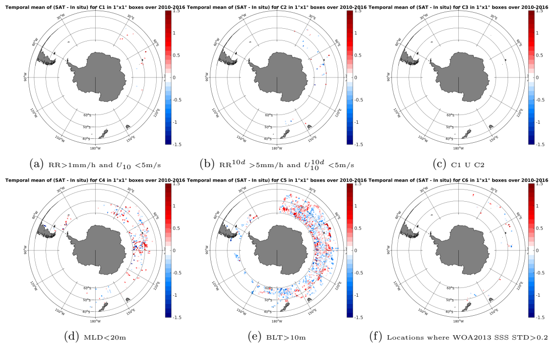
Figure 12: Temporal mean gridded over spatial boxes of size 1^\circ \times 1^\circ of \Delta SSS (SMOS-L3-CATDS-CECOS-LOCEAN-V2.1-9DAYS-25KM - Sea mammals) for 6 different subdatasets corresponding to: RR > 1\text{mm/h} and U_{10} < 5\text{m/s} (a), RR^{10d} > 5\text{mm/h} and U_{10}^{10d} < 5\text{m/s} (b), C1 U C2 (c), MLD < 20\text{m} (d), BLT > 10\text{m} (e), Locations where WOA2013 SSS STD > 0.2 (f).
