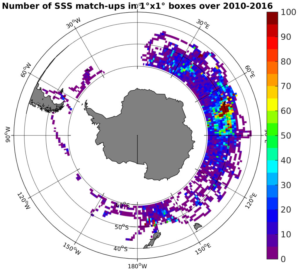
Figure 4: Number of SSS match-ups between Sea mammals SSS and the SMOS-L3-CATDS-CECOS-LOCEAN-V2.1-9DAYS-25KM SSS product for the Roaring Forties and Furious Fifties Pi-MEP region over 1^\circ \times 1^\circ boxes and for the full satellite product period.
