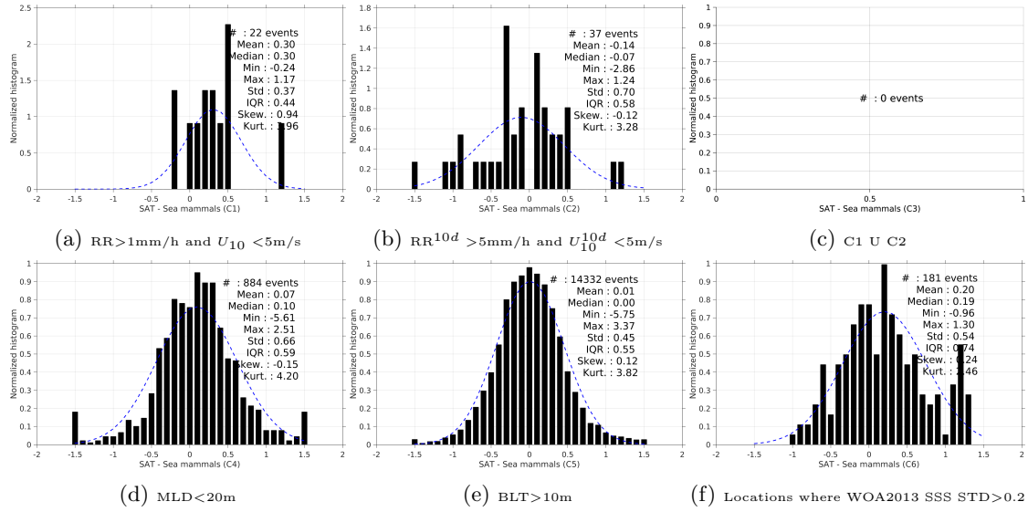
Figure 13: Normalized histogram of \Delta SSS (SMOS-L3-CATDS-CECOS-LOCEAN-V2.1-9DAYS-25KM - Sea mammals) for 6 different subdatasets corresponding to: RR>1mm/h and U_{10} < 5\text{m/s} (a), RR^{10d} > 5\text{mm/h} and U_{10}^{10d} < 5\text{m/s} (b), C1 U C2 (c),MLD<20m (d),BLT>10m (e),Locations where WOA2013 SSS STD>0.2 (f).
