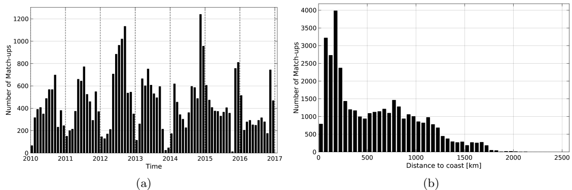
Figure 1: Number of match-ups between Sea mammals and SMOS-L3-CATDS-CECOS-LOCEAN-V2.1-9DAYS-25KM SSS as a function of time (a) and as function of the distance to coast (b) over the Roaring Forties and Furious Fifties Pi-MEP region and for the full satellite product period.
