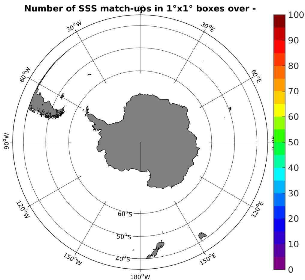
Figure 3: Number of SSS match-ups between Surface drifters SSS and the SMOS-L3-CATDS-CECOS-LOCEAN-V2.1-9DAYS-25KM SSS product for the Roaring Forties and Furious Fifties Pi-MEP region over 1°x1° boxes and for the full satellite product period.
