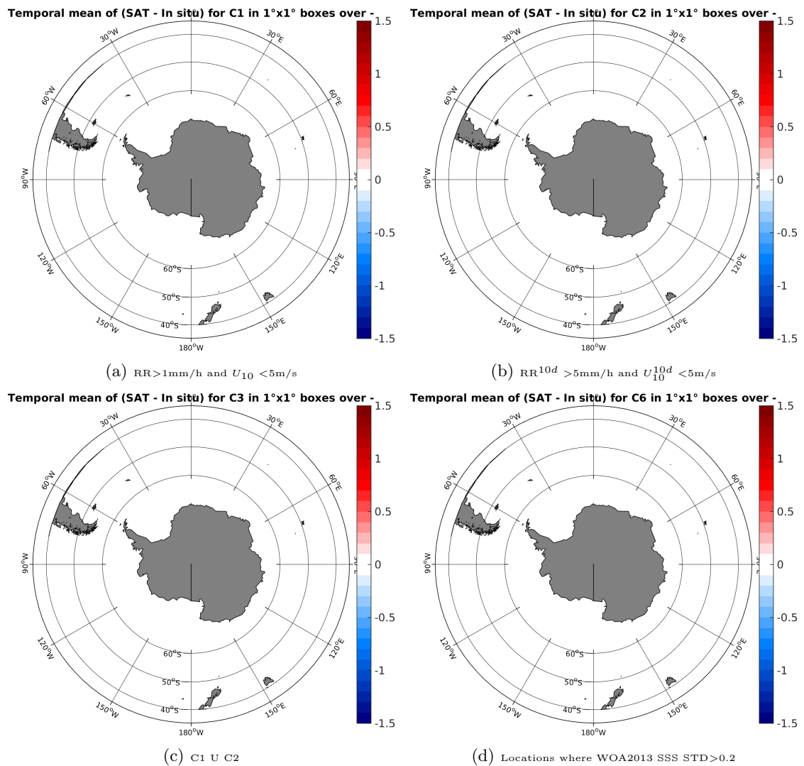
Figure 11: Temporal mean gridded over spatial boxes of size 1^\circ \times 1^\circ of \Delta SSS (SMOS-L3-CATDS-CECOS-LOCEAN-V2.1-9DAYS-25KM - Surface drifters) for 4 different subdatasets corresponding to:RR >1 mm/h and U_{10} < 5 m/s (a), RR 10d > 5 mm/h and U_{10}^{10d} < 5 m/s (b), C1 U C2 (c),Locations where WOA2013 SSS STD >0.2 (d).
