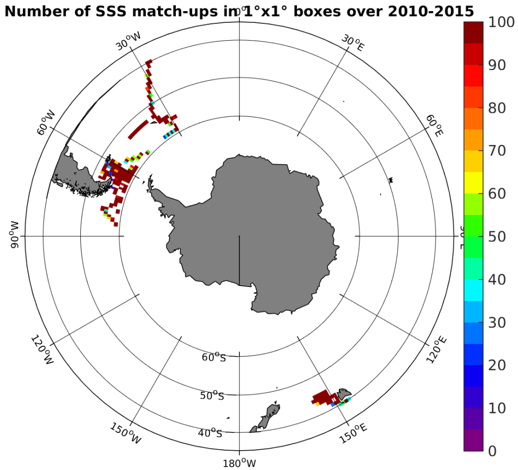
Figure 4: Number of SSS match-ups between TSG-SAMOS SSS and the SMOS-L3-CATDS-CECOS-LOCEAN-V2-9DAYS-25KM SSS product for the Roaring Forties and Furious Fifties Pi-MEP region over 1^\circ \times 1^\circ boxes and for the full satellite product period.
