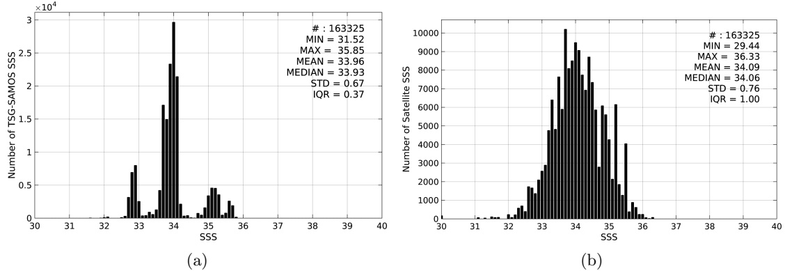
Figure 2: Histograms of SSS from TSG-SAMOS (a) and SMOS-L3-CATDS-CECOS-LOCEAN-V2-9DAYS-25KM (b) considering all match-up pairs per bins of 0.1 over the Roaring Forties and Furious Fifties Pi-MEP region and for the full satellite product period.
