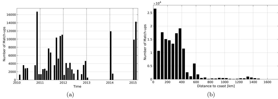
Figure 1: Number of match-ups between TSG-SAMOS and SMOS-L3-CATDS-CECOS-LOCEAN-V2-9DAYS-25KM SSS as a function of time (a) and as function of the distance to coast (b) over the Roaring Forties and Furious Fifties Pi-MEP region and for the full satellite product period.
