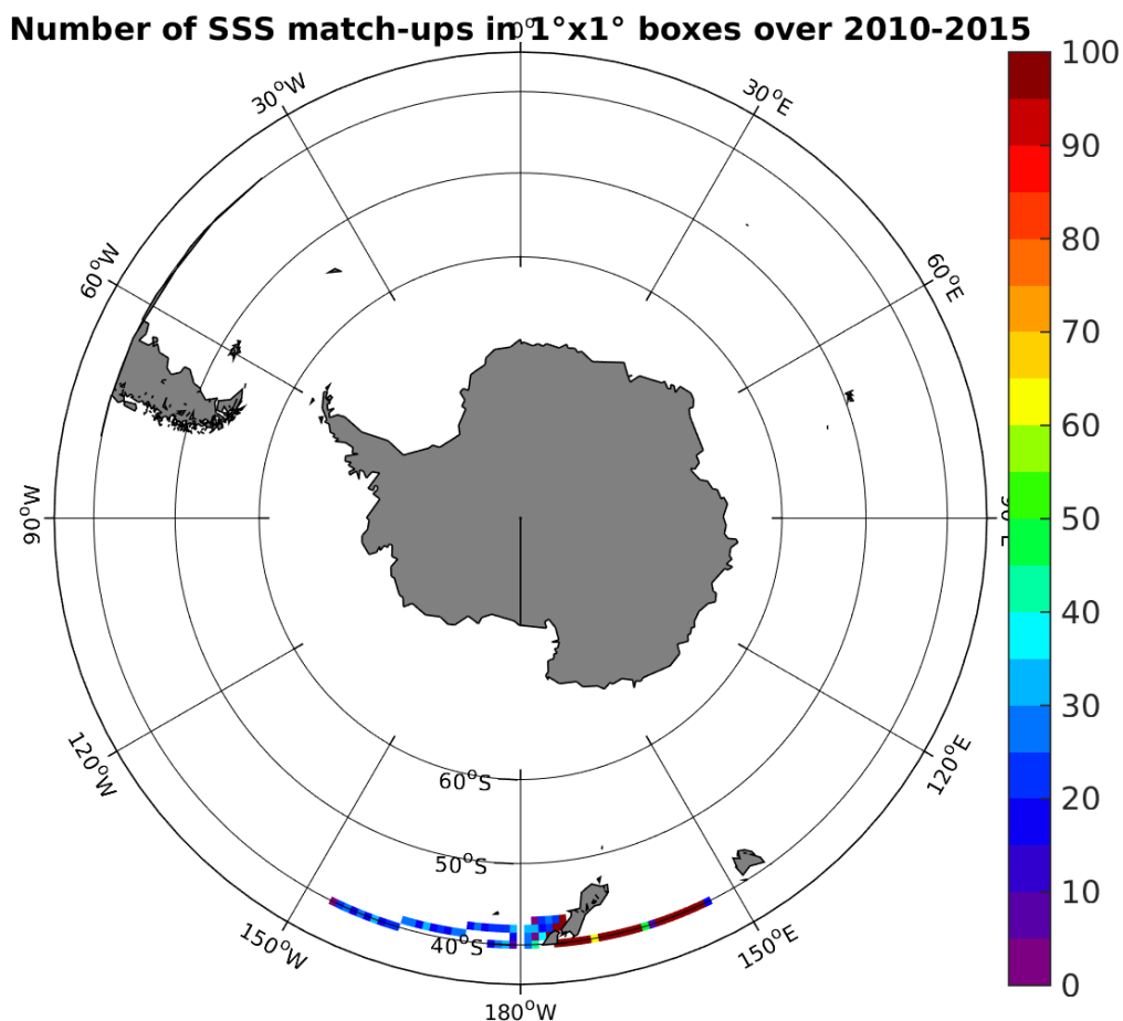
Figure 4: Number of SSS match-ups between TSG-LEGOS-DM SSS and the SMOS-L3-CATDS-CECOS-LOCEAN-V2-9DAYS-25KM SSS product for the Roaring Forties and Furious Fifties Pi-MEP region over 1°x1° boxes and for the full satellite product period.
