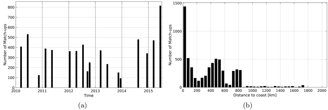
Figure 1: Number of match-ups between TSG-LEGOS-DM and SMOS-L3-CATDS-CECOS-LOCEAN-V2-9DAYS-25KM SSS as a function of time (a) and as function of the distance to coast (b) over the Roaring Forties and Furious Fifties Pi-MEP region and for the full satellite product period.
