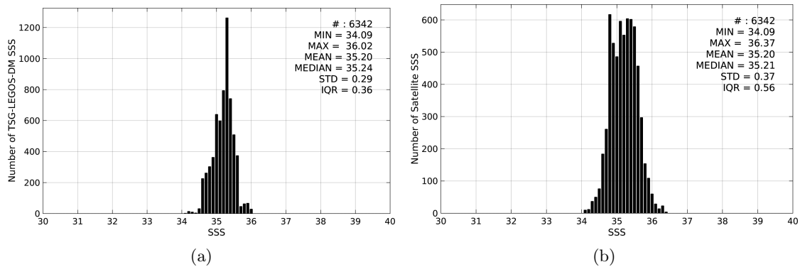
Figure 2: Histograms of SSS from TSG-LEGOS-DM (a) and SMOS-L3-CATDS-CECOS-LOCEAN-V2-9DAYS-25KM (b) considering all match-up pairs per bins of 0.1 over the Roaring Forties and Furious Fifties Pi-MEP region and for the full satellite product period.
