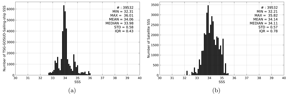
Figure 2: Histograms of SSS from TSG-GOSUD-Sailing-ship (a) and SMOS-L3-CATDS-CECOS-LOCEAN-V2-9DAYS-25KM (b) considering all match-up pairs per bins of 0.1 over the Roaring Forties and Furious Fifties Pi-MEP region and for the full satellite product period.
