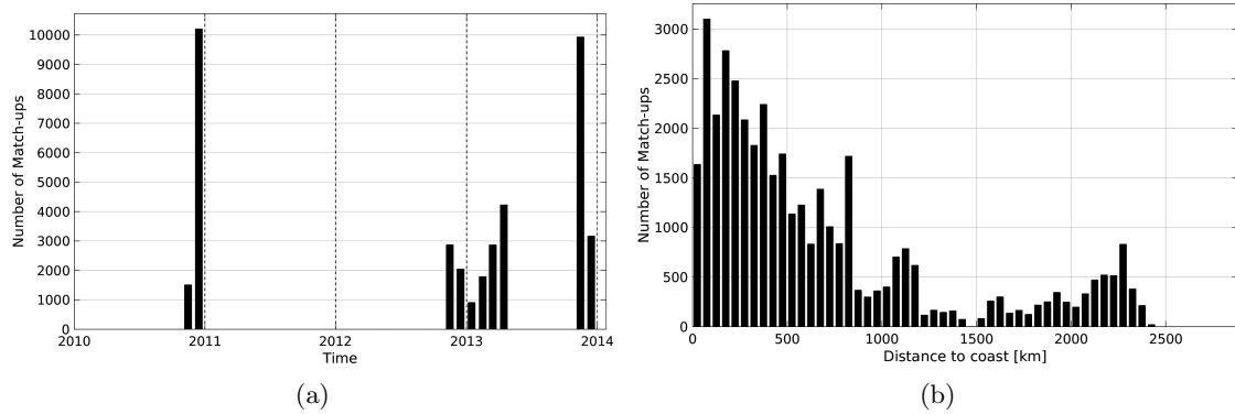
Figure 1: Number of match-ups between TSG-GOSUD-Sailing-ship and SMOS-L3-CATDS-CECOS-LOCEAN-V2-9DAYS-25KM SSS as a function of time (a) and as function of the distance to coast (b) over the Roaring Forties and Furious Fifties Pi-MEP region and for the full satellite product period.
