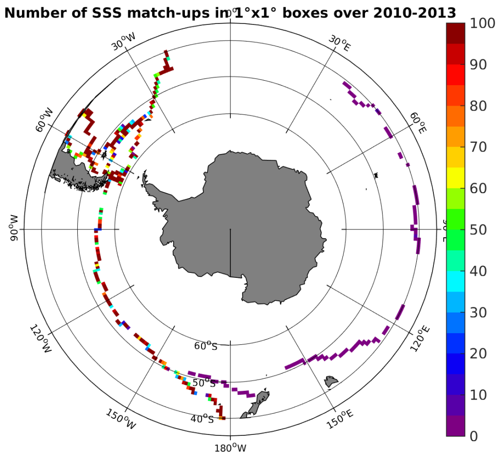
Figure 4: Number of SSS match-ups between TSG-GOSUD-Sailing-ship SSS and the SMOS-L3-CATDS-CECOS-LOCEAN-V2-9DAYS-25KM SSS product for the Roaring Forties and Furious Fifties Pi-MEP region over 1^\circ \times 1^\circ boxes and for the full satellite product period.
