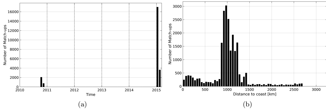
Figure 1: Number of match-ups between TSG-GOSUD-Research-vessel and SMOS-L3-CATDS-CECOS-LOCEAN-V2-9DAYS-25KM SSS as a function of time (a) and as function of the distance to coast (b) over the Roaring Forties and Furious Fifties Pi-MEP region and for the full satellite product period.
