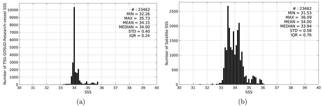
Figure 2: Histograms of SSS from TSG-GOSUD-Research-vessel (a) and SMOS-L3-CATDS-CECOS-LOCEAN-V2-9DAYS-25KM (b) considering all match-up pairs per bins of 0.1 over the Roaring Forties and Furious Fifties Pi-MEP region and for the full satellite product period.
