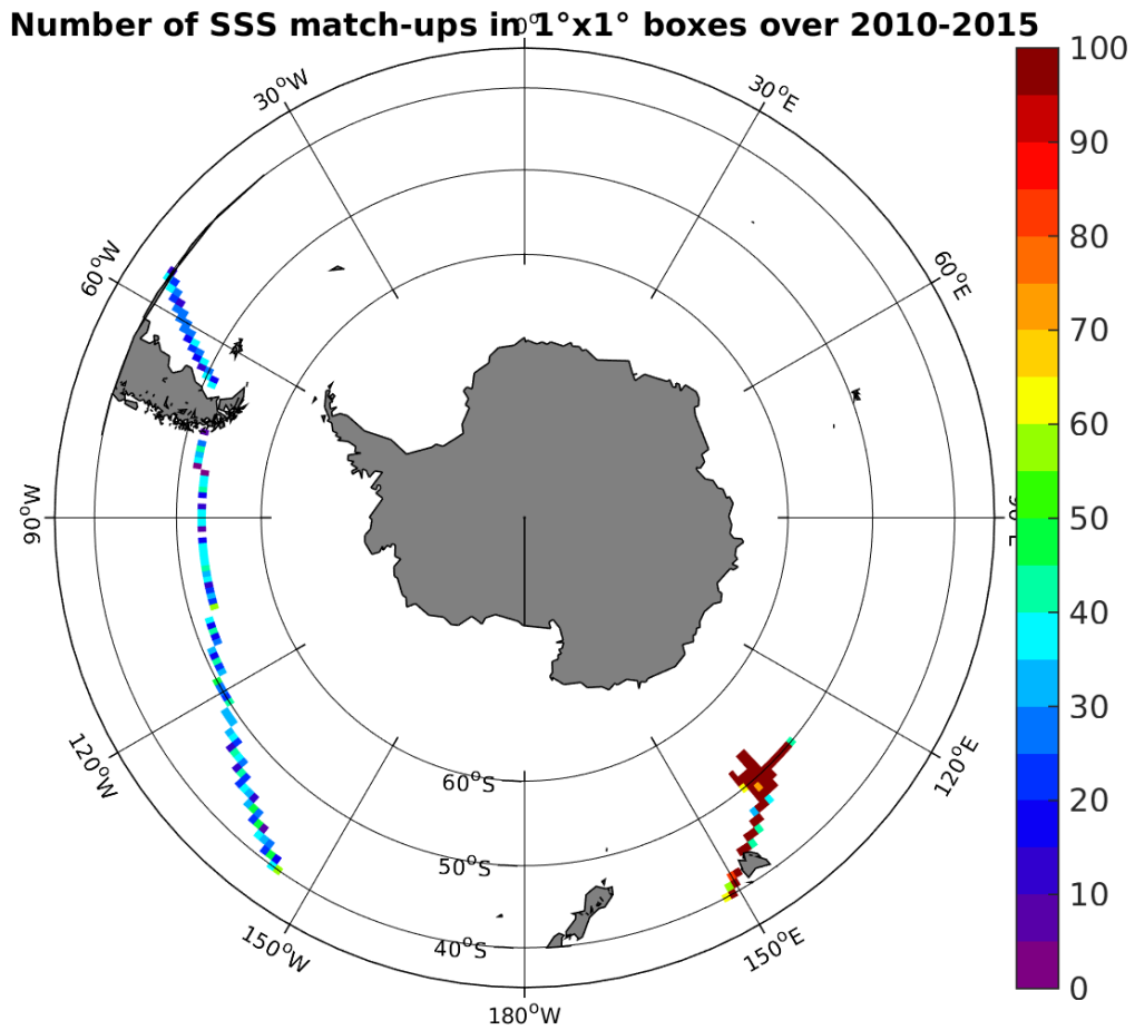
Figure 4: Number of SSS match-ups between TSG-GOSUD-Research-vessel SSS and the SMOS-L3-CATDS-CECOS-LOCEAN-V2-9DAYS-25KM SSS product for the Roaring Forties and Furious Fifties Pi-MEP region over 1^\circ \times 1^\circ boxes and for the full satellite product period.
