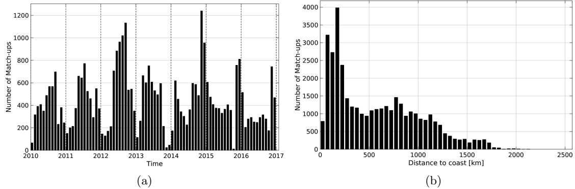
Figure 1: Number of match-ups between Sea mammals and SMOS-L3-CATDS-CECOS-LOCEAN-V2-9DAYS-25KM SSS as a function of time (a) and as function of the distance to coast (b) over the Roaring Forties and Furious Fifties Pi-MEP region and for the full satellite product period.
