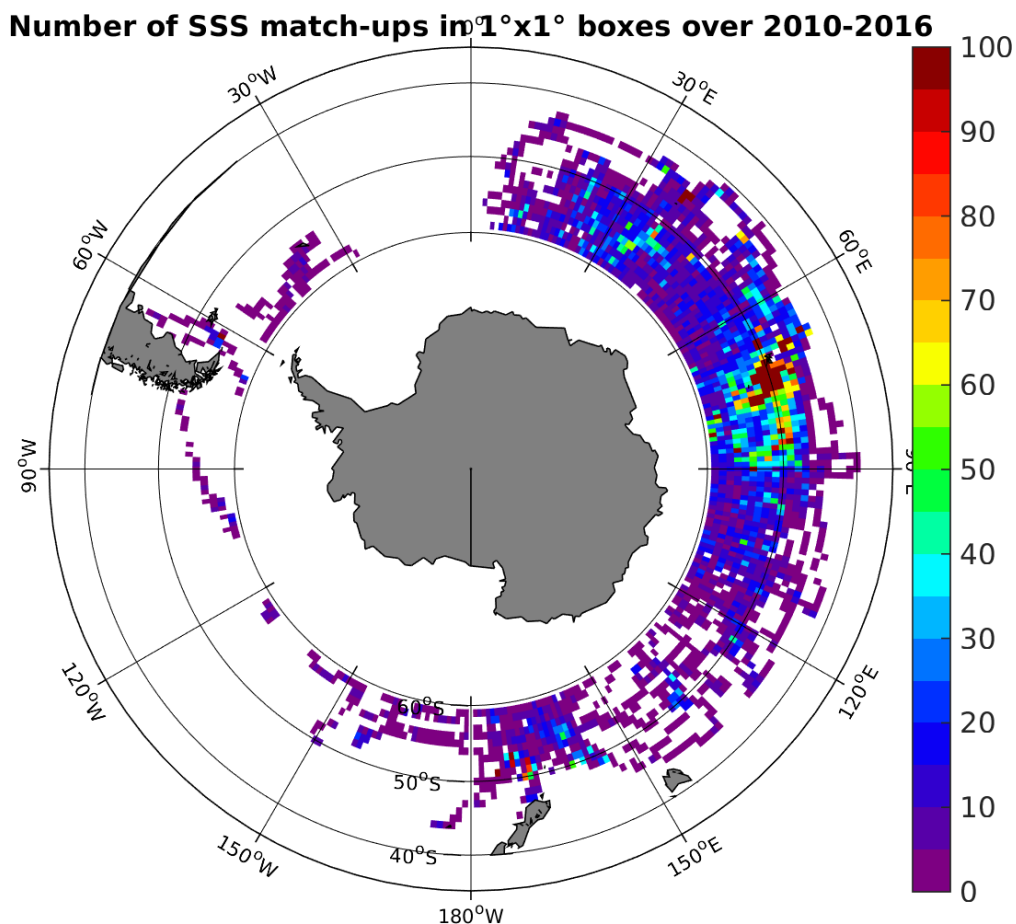
Figure 4: Number of SSS match-ups between Sea mammals SSS and the SMOS-L3-CATDS-CECOS-LOCEAN-V2-9DAYS-25KM SSS product for the Roaring Forties and Furious Fifties Pi-MEP region over 1^\circ \times 1^\circ boxes and for the full satellite product period.
