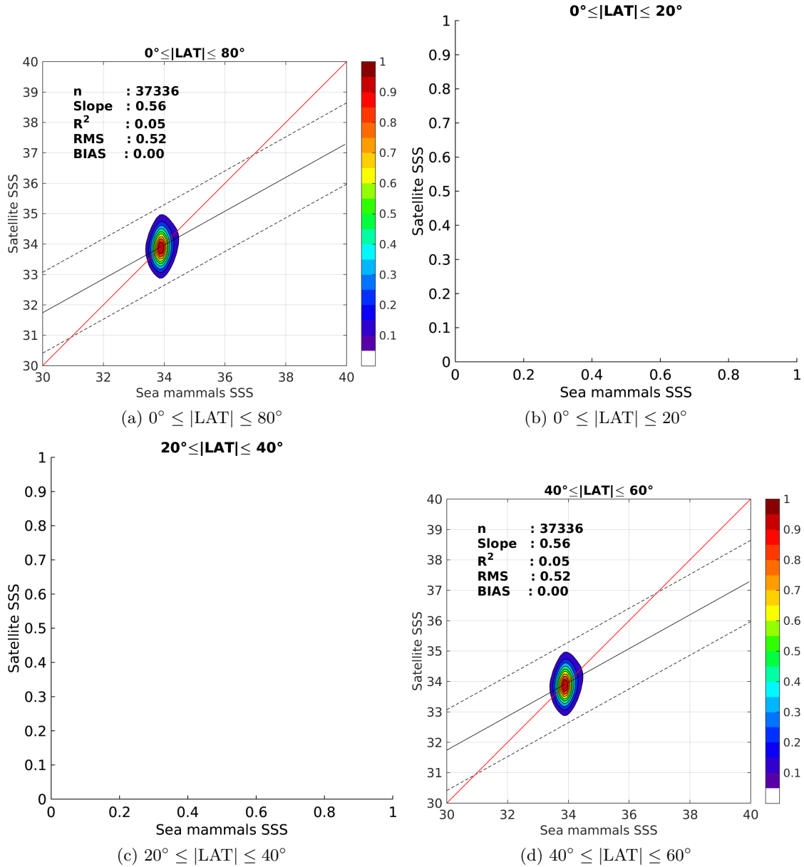
Figure 9: Contour maps of the concentration of SMOS-L3-CATDS-CECOS-LOCEAN-V2-9DAYS-25KM SSS (y-axis) versus Sea mammals SSS (x-axis) at match-up pairs for different latitude bands. For each plot, the red line shows x=y . The black thin and dashed lines indicate a linear fit through the data cloud and the \pm 95\% confidence levels, respectively. The number of match-up pairs n , the slope and R^2 coefficient of the linear fit, the root mean square (RMS) and the mean bias between satellite and in situ data are indicated for each latitude band in each plot.
