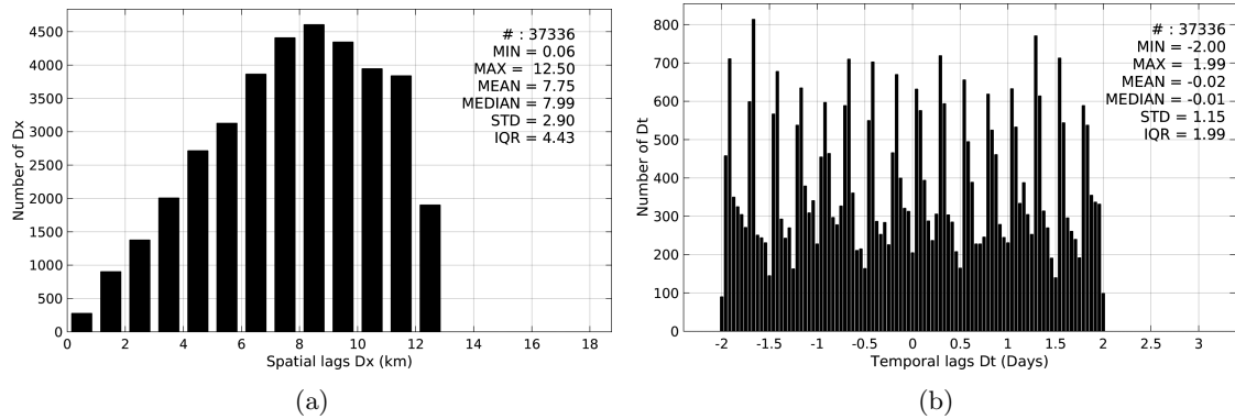
Figure 5: Histograms of the spatial (a) and temporal (b) lags between the time of the Sea mammals measurements and the date of the corresponding SMOS-L3-CATDS-CECOS-LOCEAN-V2-9DAYS-25KM SSS product.
