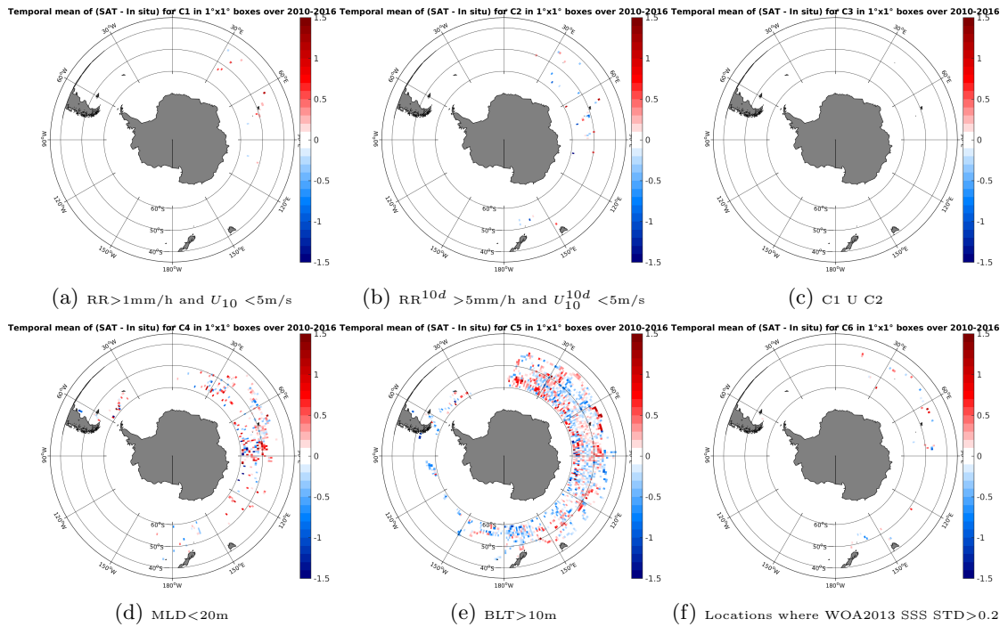
Figure 12: Temporal mean gridded over spatial boxes of size 1^\circ \times 1^\circ of \Delta SSS (SMOS-L3-CATDS-CECOS-LOCEAN-V2-9DAYS-25KM - Sea mammals) for 6 different subdatasets corresponding to: RR > 1\text{mm/h} and U_{10} < 5\text{m/s} (a), RR^{10d} > 5\text{mm/h} and U_{10}^{10d} < 5\text{m/s} (b), C1 U C2 (c), MLD < 20\text{m} (d), BLT > 10\text{m} (e), Locations where WOA2013 SSS STD > 0.2 (f).
