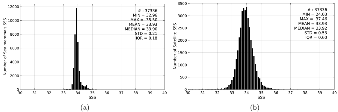
Figure 2: Histograms of SSS from Sea mammals (a) and SMOS-L3-CATDS-CECOS-LOCEAN-V2-9DAYS-25KM (b) considering all match-up pairs per bins of 0.1 over the Roaring Forties and Furious Fifties Pi-MEP region and for the full satellite product period.
