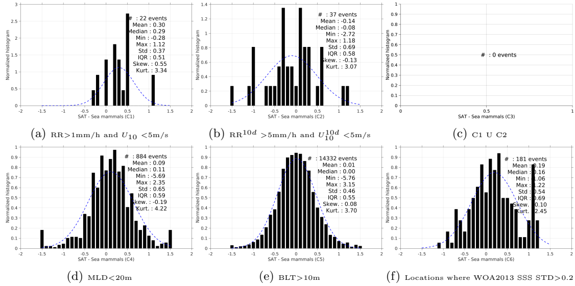
Figure 13: Normalized histogram of \Delta SSS (SMOS-L3-CATDS-CECOS-LOCEAN-V2-9DAYS-25KM - Sea mammals) for 6 different subdatasets corresponding to: RR>1mm/h and U_{10} < 5\text{m/s} (a), RR 10d >5mm/h and U_{10}^{10d} < 5\text{m/s} (b), C1 U C2 (c),MLD<20m (d),BLT>10m (e),Locations where WOA2013 SSS STD>0.2 (f).
