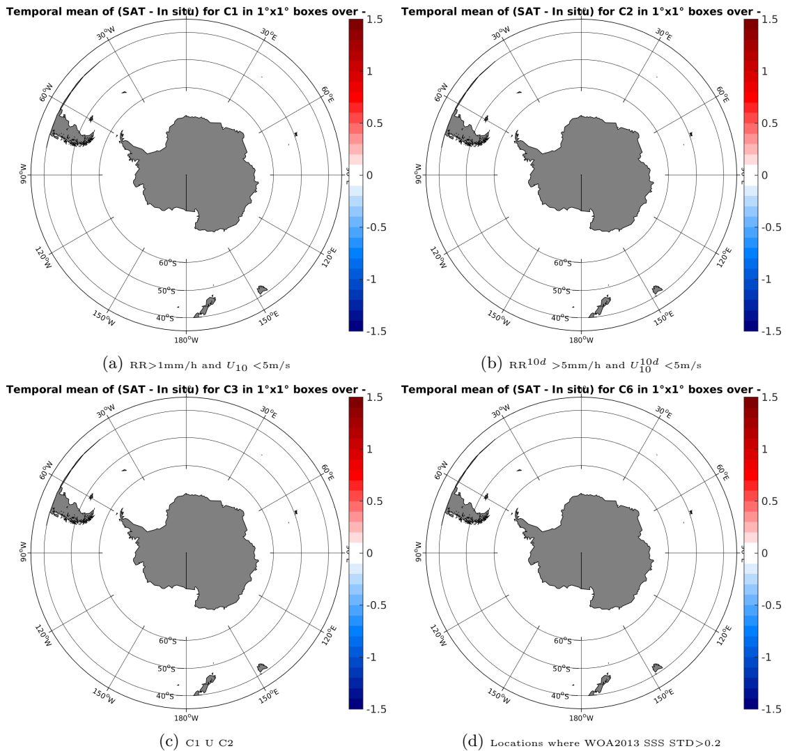
Figure 11: Temporal mean gridded over spatial boxes of size 1^\circ \times 1^\circ of \Delta SSS (SMOS-L3-CATDS-CECOS-LOCEAN-V2-9DAYS-25KM - Surface drifters) for 4 different subdatasets corresponding to: RR > 1\text{mm/h} and U_{10} < 5\text{m/s} (a), RR^{10d} > 5\text{mm/h} and U_{10}^{10d} < 5\text{m/s} (b), C1 U C2 (c), Locations where WOA2013 SSS STD > 0.2 (d).
