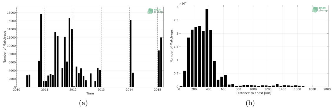
Figure 1: Number of match-ups between TSG (SAMOS) and SMOS SSS L3 v2 - Monthly - 0.25 Deg (CATDS-CECOS-IFREMER) SSS as a function of time (a) and as function of the distance to coast (b) over the Roaring Forties and Furious Fifties Pi-MEP region and for the full satellite product period.
