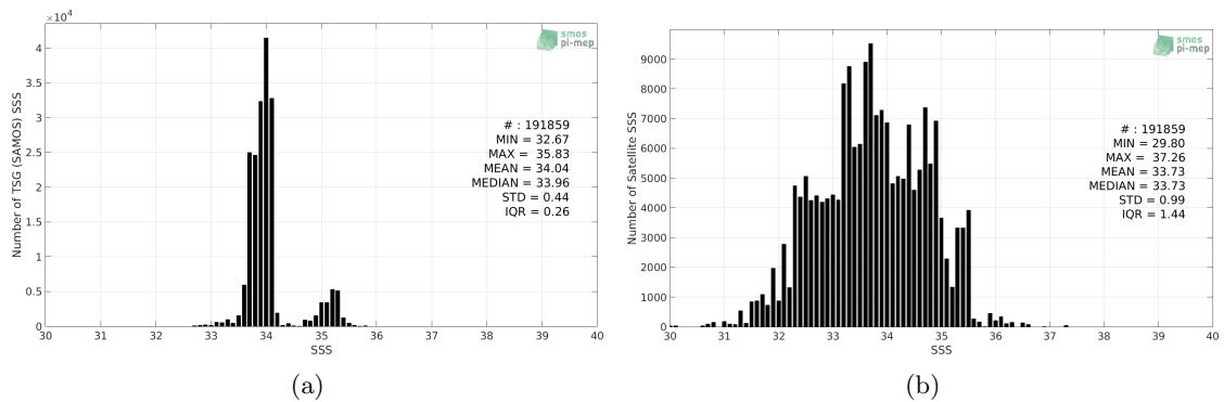
Figure 2: Histograms of SSS from TSG (SAMOS) (a) and SMOS SSS L3 v2 - Monthly - 0.25 Deg (CATDS-CECOS-IFREMER) (b) considering all match-up pairs per bins of 0.1 over the Roaring Forties and Furious Fifties Pi-MEP region and for the full satellite product period.
