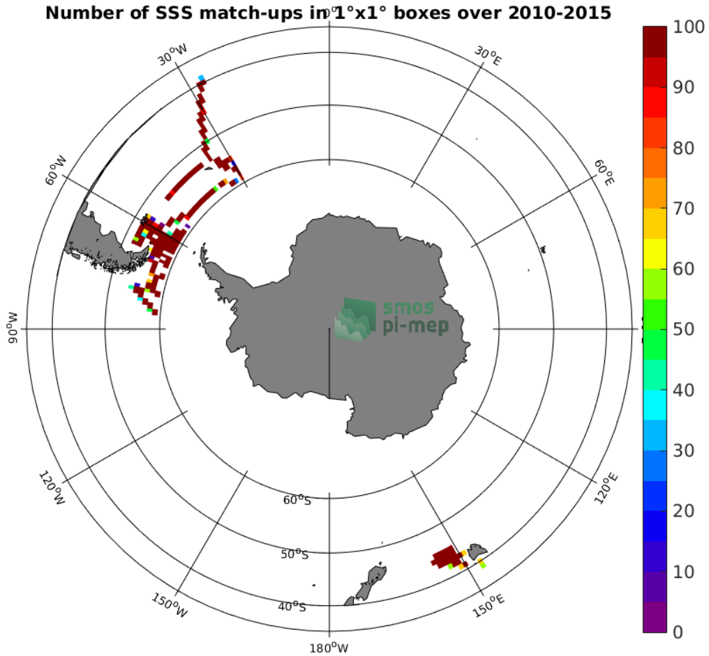
Figure 4: Number of SSS match-ups between TSG (SAMOS) SSS and the SMOS SSS L3 v2 - Monthly - 0.25 Deg (CATDS-CECOS-IFREMER) SSS product for the Roaring Forties and Furious Fifties Pi-MEP region over 1°x1° boxes and for the full satellite product period.
