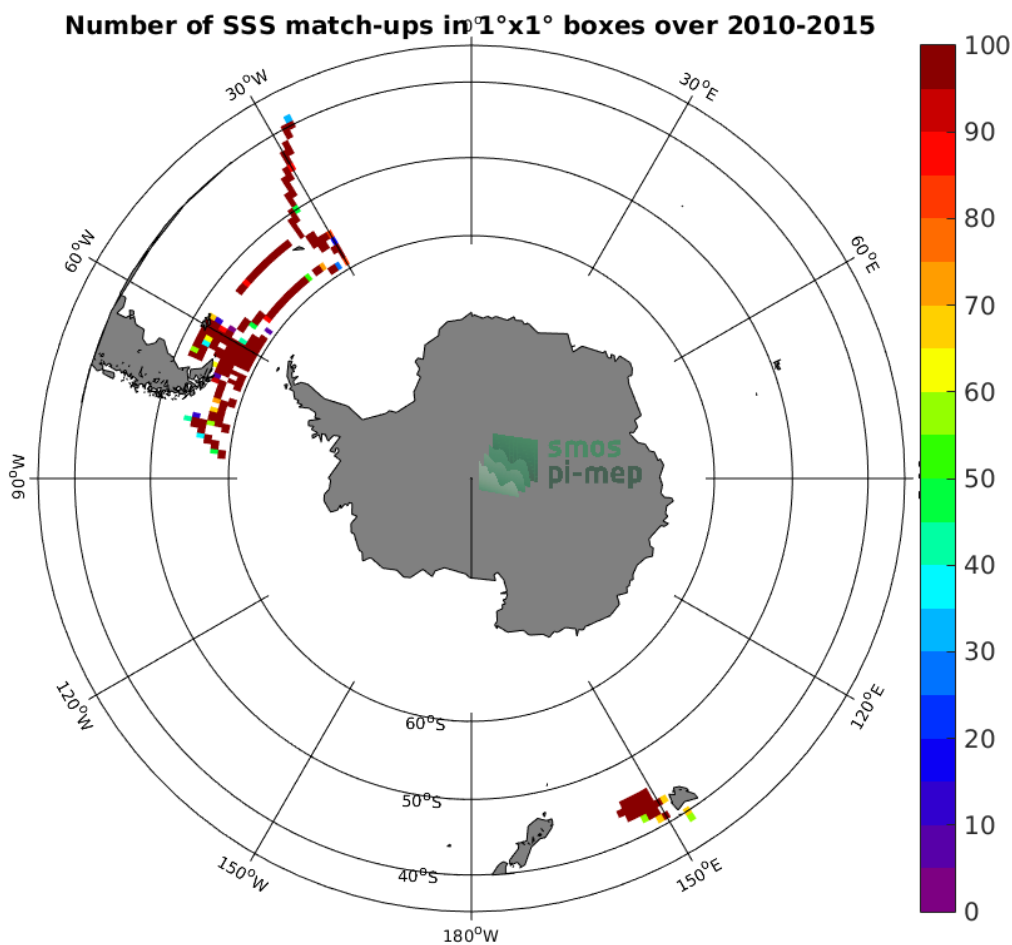
Figure 4: Number of SSS match-ups between TSG-SAMOS SSS and the SMOS L3 v2 - Monthly - 0.25 Deg (CATDS-CECOS-IFREMER) SSS product for the Roaring Forties and Furious Fifties Pi-MEP region over 1°x1° boxes and for the full satellite product period.
