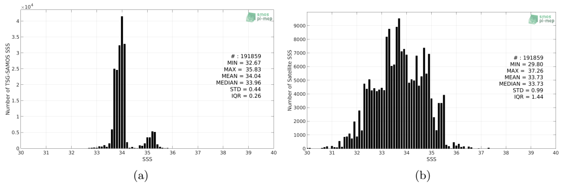
Figure 2: Histograms of SSS from TSG-SAMOS (a) and SMOS L3 v2 - Monthly - 0.25 Deg (CATDS-CECOS-IFREMER) (b) considering all match-up pairs per bins of 0.1 over the Roaring Forties and Furious Fifties Pi-MEP region and for the full satellite product period.
