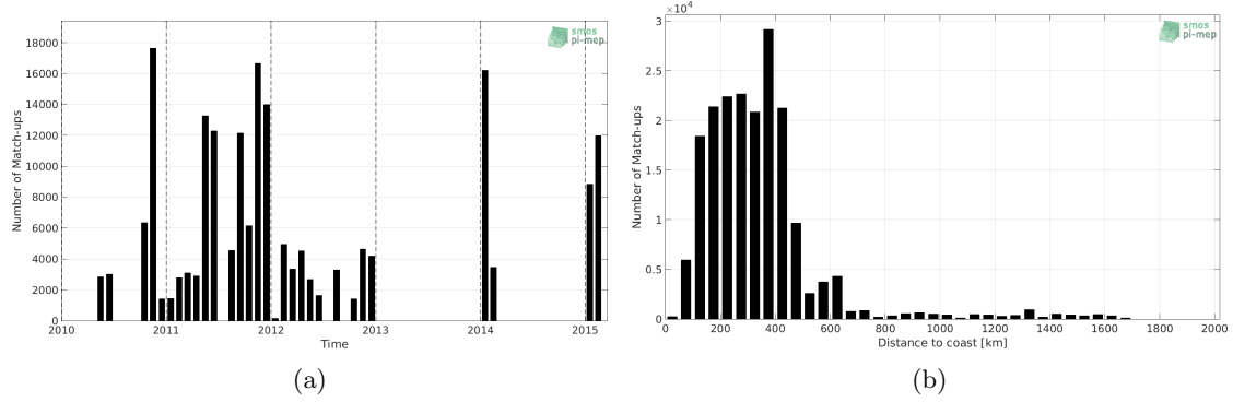
Figure 1: Number of match-ups between TSG-SAMOS and SMOS L3 v2 - Monthly - 0.25 Deg (CATDS-CECOS-IFREMER) SSS as a function of time (a) and as function of the distance to coast (b) over the Roaring Forties and Furious Fifties Pi-MEP region and for the full satellite product period.
