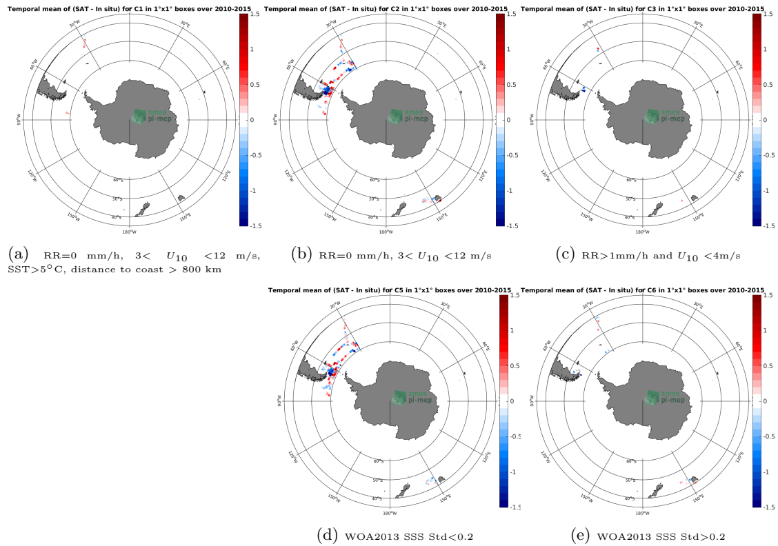
Figure 12: Temporal mean gridded over spatial boxes of size 1^\circ \times 1^\circ of \Delta SSS (SMOS-L3-CATDS-IFREMER-CECOS-V2-MONTHLY-0.25DEG - TSG-SAMOS) for 5 different subdatasets corresponding to:RR=0 mm/h, 3 < U_{10} < 12 m/s, SST >5^\circ C, distance to coast > 800 km (a), RR=0 mm/h, 3 < U_{10} < 12 m/s (b), RR >1 mm/h and U_{10} < 4 m/s (c), WOA2013 SSS Std <0.2 (d), WOA2013 SSS Std >0.2 (e).
