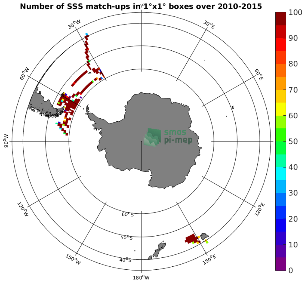
Figure 4: Number of SSS match-ups between TSG-SAMOS SSS and the SMOS-L3-CATDS-IFREMER-CECOS-V2-MONTHLY-0.25DEG SSS product for the Roaring Forties and Furious Fifties Pi-MEP region over 1°x1° boxes and for the full satellite product period.
