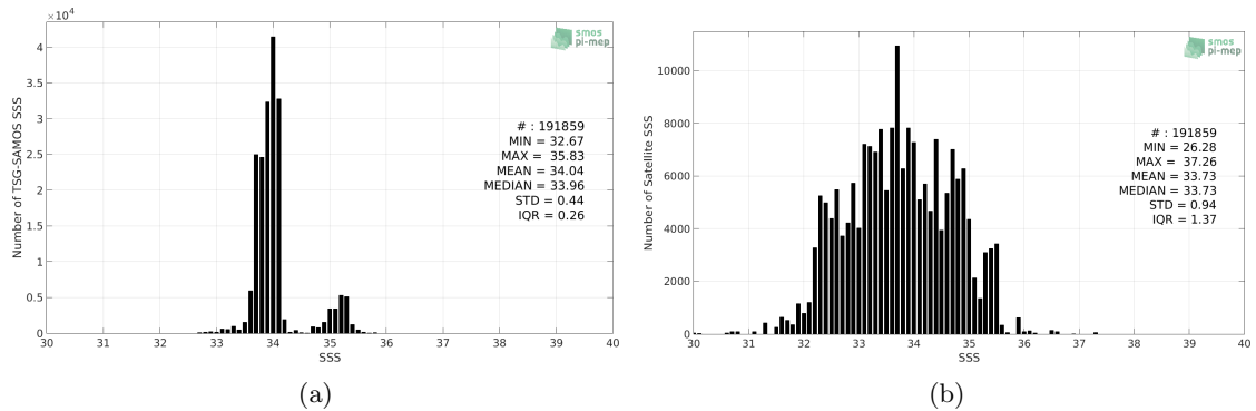
Figure 2: Histograms of SSS from TSG-SAMOS (a) and SMOS-L3-CATDS-IFREMER-CECOS-V2-MONTHLY-0.25DEG (b) considering all match-up pairs per bins of 0.1 over the Roaring Forties and Furious Fifties Pi-MEP region and for the full satellite product period.
