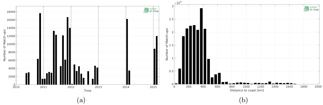
Figure 1: Number of match-ups between TSG-SAMOS and SMOS-L3-CATDS-IFREMER-CECOS-V2-MONTHLY-0.25DEG SSS as a function of time (a) and as function of the distance to coast (b) over the Roaring Forties and Furious Fifties Pi-MEP region and for the full satellite product period.
