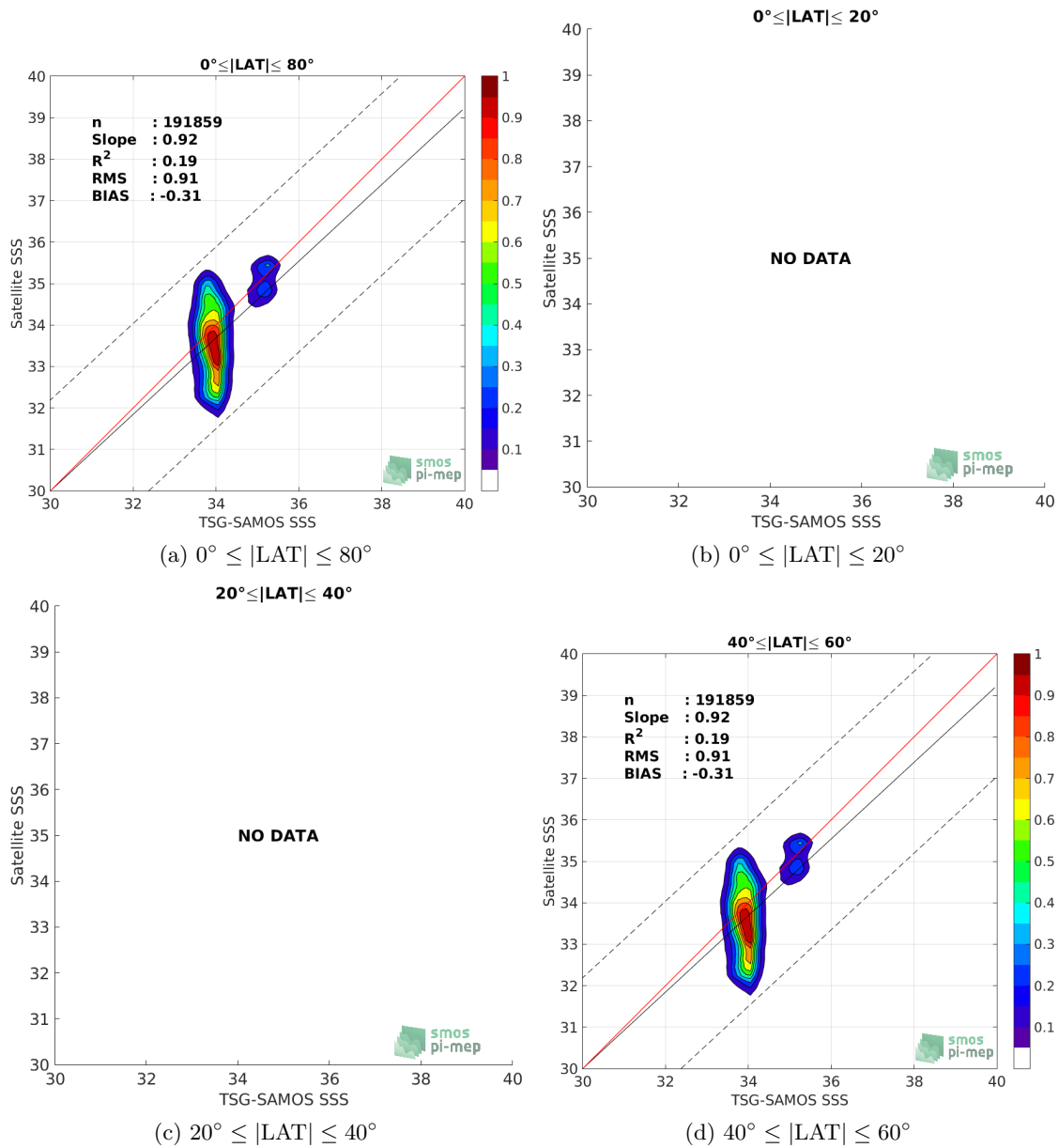
Figure 9: Contour maps of the concentration of SMOS-L3-CATDS-IFREMER-CECOS-V2-MONTHLY-0.25DEG SSS ( y -axis) versus TSG-SAMOS SSS ( x -axis) at match-up pairs for different latitude bands. For each plot, the red line shows x=y . The black thin and dashed lines indicate a linear fit through the data cloud and the \pm 95\% confidence levels, respectively. The number match-up pairs n , the slope and R^2 coefficient of the linear fit, the root mean square (RMS) and the mean bias between satellite and in situ data are indicated for each latitude band in each plots.
