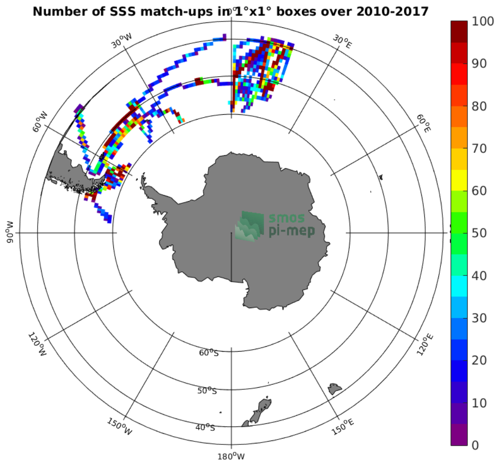
Figure 4: Number of SSS match-ups between TSG (Polarstern) SSS and the SMOS SSS L3 v2 - Monthly - 0.25 Deg (CATDS-CECOS-IFREMER) SSS product for the Roaring Forties and Furious Fifties Pi-MEP region over 1^\circ \times 1^\circ boxes and for the full satellite product period.
