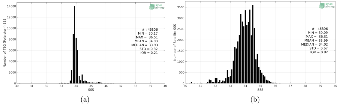
Figure 2: Histograms of SSS from TSG (Polarstern) (a) and SMOS SSS L3 v2 - Monthly - 0.25 Deg (CATDS-CECOS-IFREMER) (b) considering all match-up pairs per bins of 0.1 over the Roaring Forties and Furious Fifties Pi-MEP region and for the full satellite product period.
