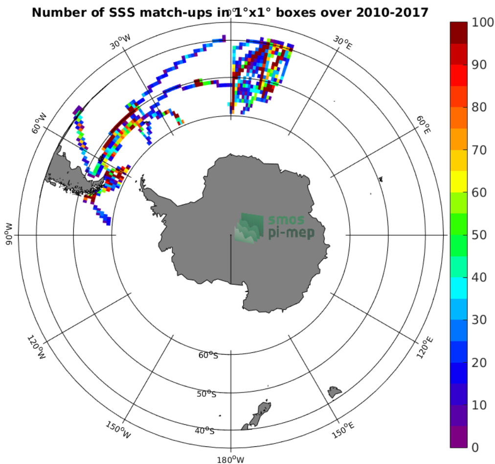
Figure 4: Number of SSS match-ups between TSG-POLARSTERN SSS and the SMOS L3 v2 - Monthly - 0.25 Deg (CATDS-CECOS-IFREMER) SSS product for the Roaring Forties and Furious Fifties Pi-MEP region over 1°x1° boxes and for the full satellite product period.
