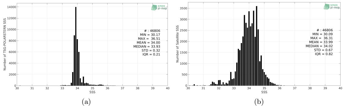
Figure 2: Histograms of SSS from TSG-POLARSTERN (a) and SMOS L3 v2 - Monthly - 0.25 Deg (CATDS-CECOS-IFREMER) (b) considering all match-up pairs per bins of 0.1 over the Roaring Forties and Furious Fifties Pi-MEP region and for the full satellite product period.
