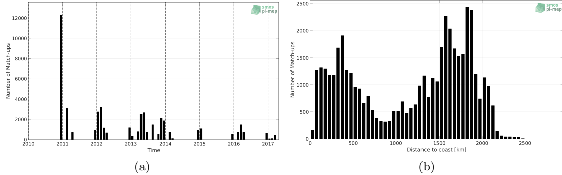
Figure 1: Number of match-ups between TSG-POLARSTERN and SMOS L3 v2 - Monthly - 0.25 Deg (CATDS-CECOS-IFREMER) SSS as a function of time (a) and as function of the distance to coast (b) over the Roaring Forties and Furious Fifties Pi-MEP region and for the full satellite product period.
