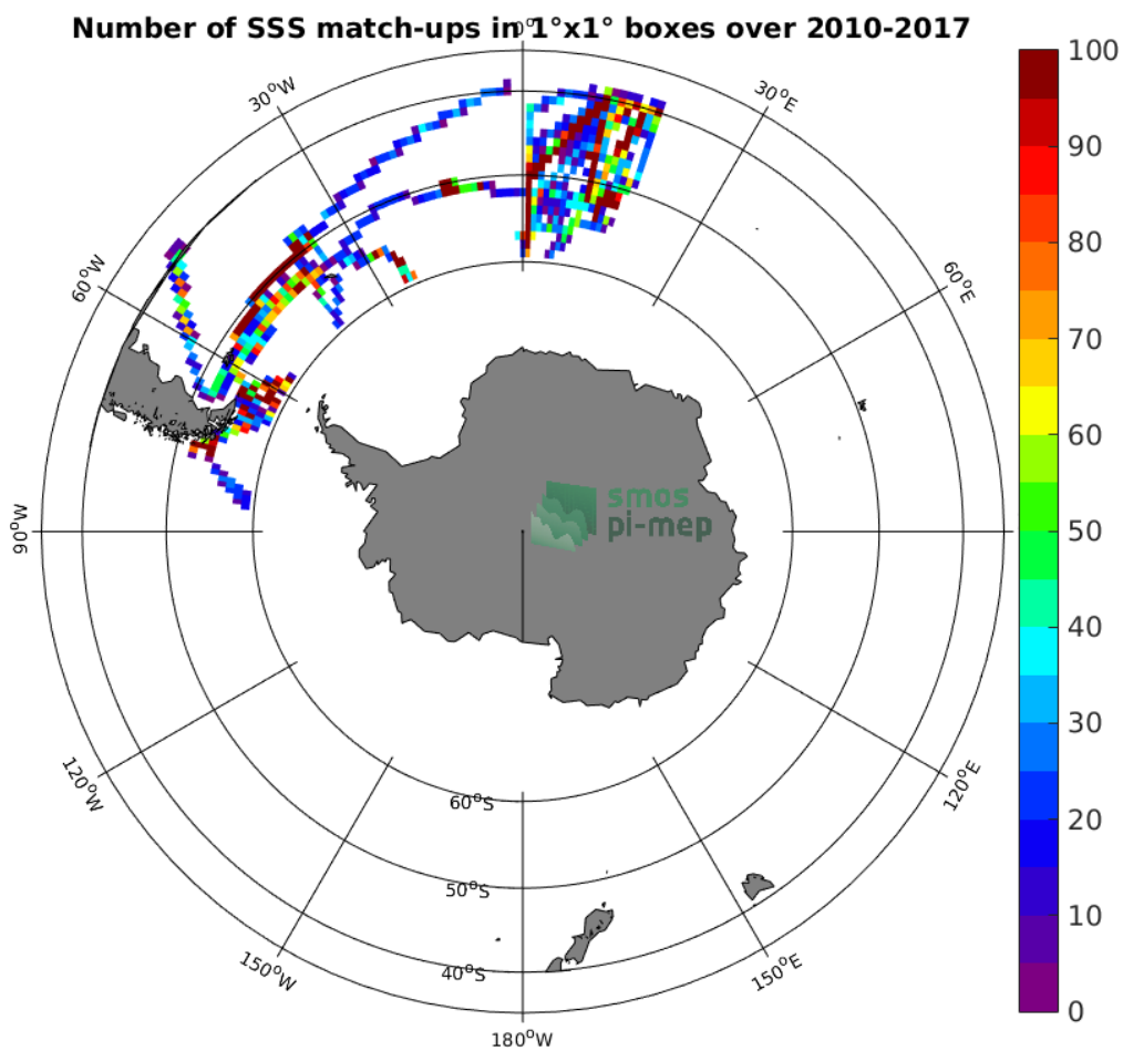
Figure 4: Number of SSS match-ups between TSG-POLARSTERN SSS and the SMOS-L3-CATDS-IFREMER-CECOS-V2-MONTHLY-0.25DEG SSS product for the Roaring Forties and Furious Fifties Pi-MEP region over 1°x1° boxes and for the full satellite product period.
