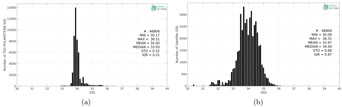
Figure 2: Histograms of SSS from TSG-POLARSTERN (a) and SMOS-L3-CATDS-IFREMER-CECOS-V2-MONTHLY-0.25DEG (b) considering all match-up pairs per bins of 0.1 over the Roaring Forties and Furious Fifties Pi-MEP region and for the full satellite product period.
