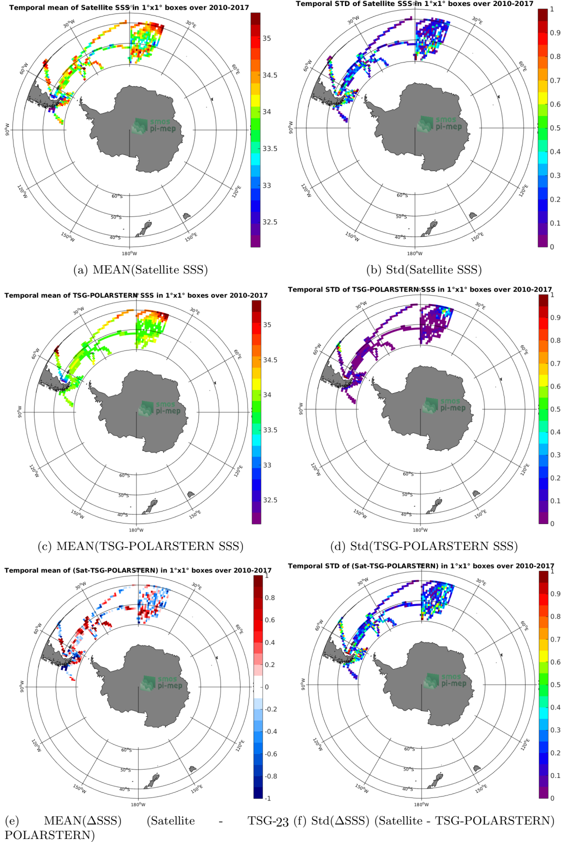
Figure 6: Temporal mean (left) and Std (right) of SSS from SMOS-L3-CATDS-IFREMER-CECOS-V2-MONTHLY-0.25DEG (top), TSG-POLARSTERN (middle), and of \Delta SSS (Satellite - TSG-POLARSTERN). Only match-up pairs are used to generate these maps.
