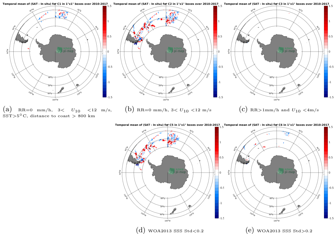
Figure 12: Temporal mean gridded over spatial boxes of size 1^\circ \times 1^\circ of \Delta SSS (SMOS-L3-CATDS-IFREMER-CECOS-V2-MONTHLY-0.25DEG - TSG-POLARSTERN) for 5 different subdatasets corresponding to:RR=0 mm/h, 3 < U_{10} < 12 m/s, SST >5^\circ C, distance to coast > 800 km (a), RR=0 mm/h, 3 < U_{10} < 12 m/s (b), RR >1 mm/h and U_{10} < 4 m/s (c), WOA2013 SSS Std <0.2 (d), WOA2013 SSS Std >0.2 (e).
