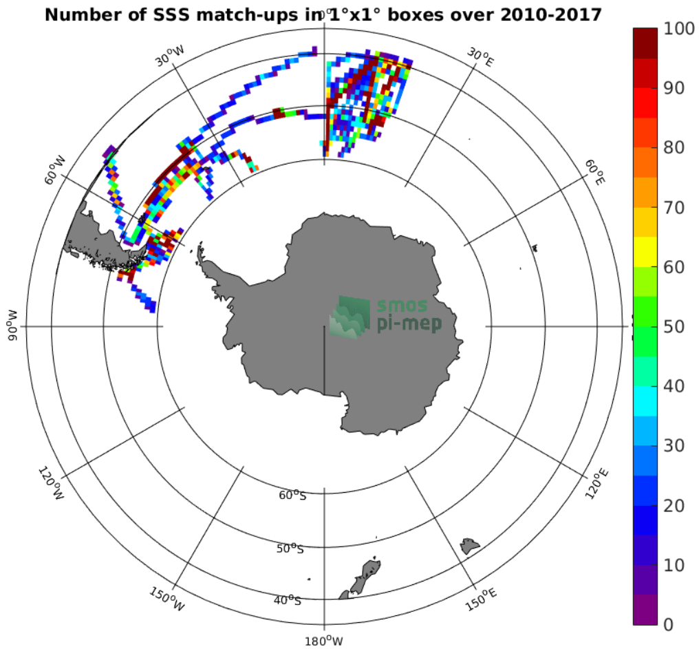
Figure 4: Number of SSS match-ups between TSG-POLARSTERN SSS and the SMOS-L3-CATDS-IFREMER-CECOS-V2-MONTHLY-0.25DEG SSS product for the Roaring Forties and Furious Fifties Pi-MEP region over 1^\circ \times 1^\circ boxes and for the full satellite product period.
