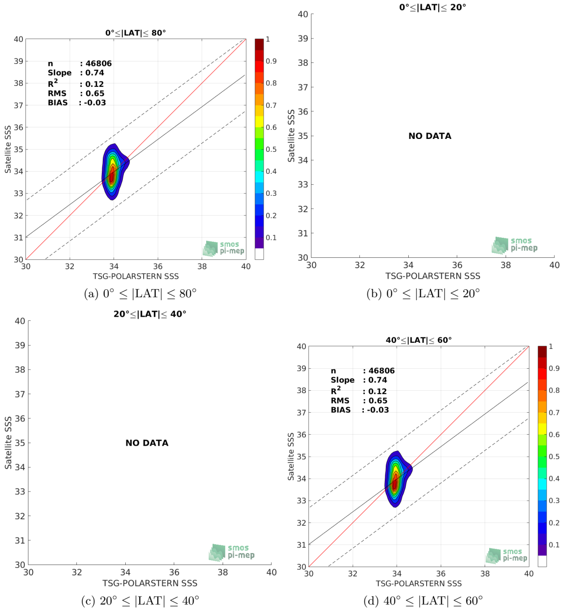
Figure 9: Contour maps of the concentration of SMOS-L3-CATDS-IFREMER-CECOS-V2-MONTHLY-0.25DEG SSS (y-axis) versus TSG-POLARSTERN SSS (x-axis) at match-up pairs for different latitude bands. For each plot, the red line shows x=y . The black thin and dashed lines indicate a linear fit through the data cloud and the \pm 95\% confidence levels, respectively. The number match-up pairs n , the slope and R^2 coefficient of the linear fit, the root mean square (RMS) and the mean bias between satellite and in situ data are indicated for each latitude band in each plots.
