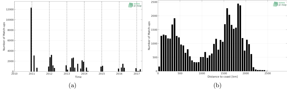
Figure 1: Number of match-ups between TSG-POLARSTERN and SMOS-L3-CATDS-IFREMER-CECOS-V2-MONTHLY-0.25DEG SSS as a function of time (a) and as function of the distance to coast (b) over the Roaring Forties and Furious Fifties Pi-MEP region and for the full satellite product period.
