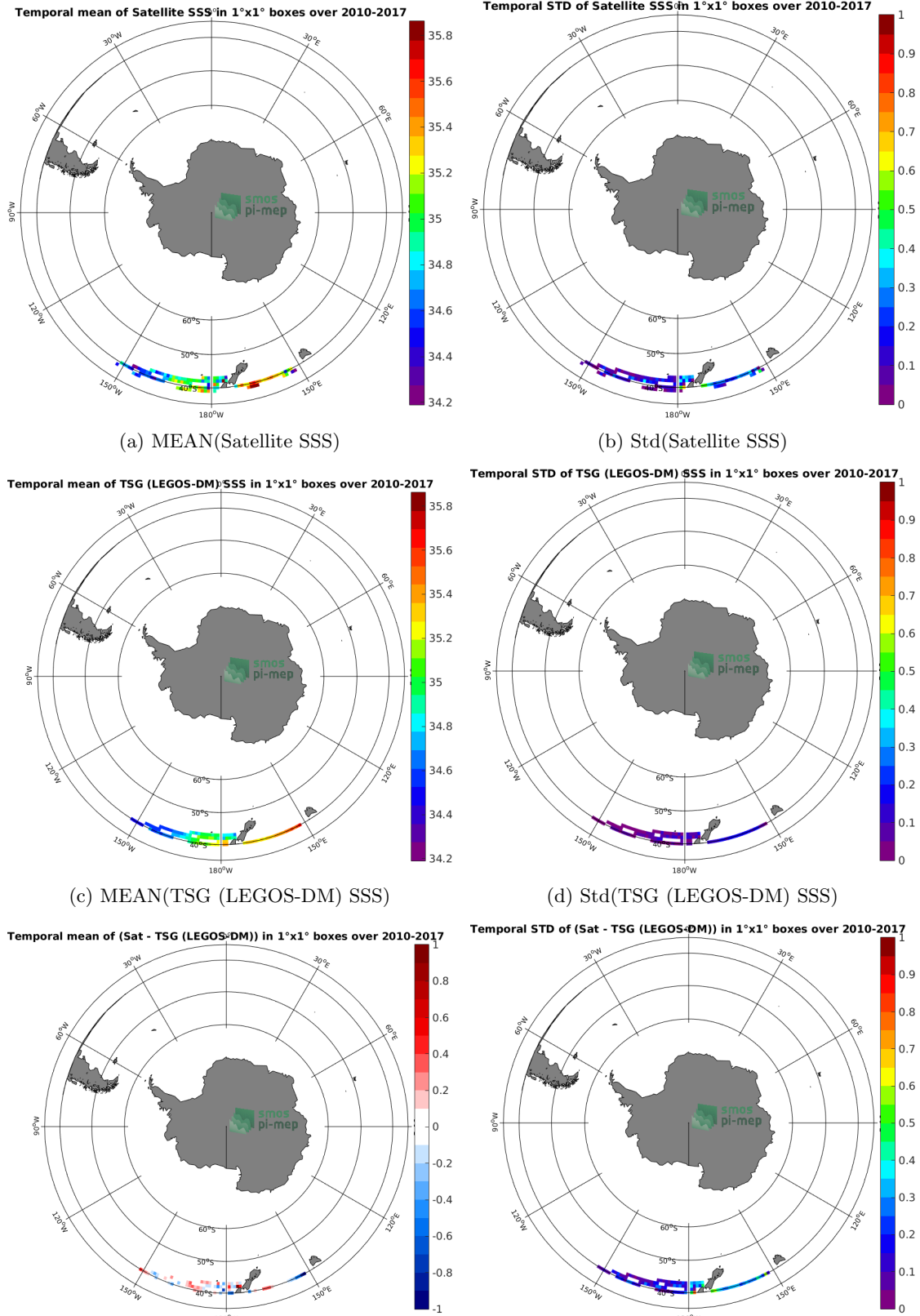
Figure 6: Temporal mean (left) and Std (right) of SSS from SMOS SSS L3 v2 - Monthly - 0.25 Deg (CATDS-CECOS-IFREMER) (top), TSG (LEGOS-DM) (middle), and of \Delta SSS (Satellite - TSG (LEGOS-DM)). Only match-up pairs are used to generate these maps.
