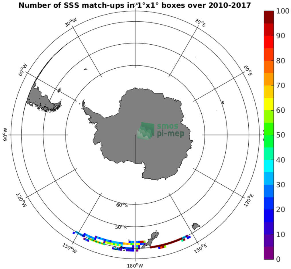
Figure 4: Number of SSS match-ups between TSG (LEGOS-DM) SSS and the SMOS SSS L3 v2 - Monthly - 0.25 Deg (CATDS-CECOS-IFREMER) SSS product for the Roaring Forties and Furious Fifties Pi-MEP region over 1°x1° boxes and for the full satellite product period.
