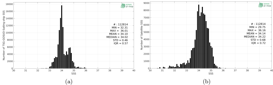
Figure 2: Histograms of SSS from TSG-GOSUD-Sailing-ship (a) and SMOS L3 v2 - Monthly - 0.25 Deg (CATDS-CECOS-IFREMER) (b) considering all match-up pairs per bins of 0.1 over the Roaring Forties and Furious Fifties Pi-MEP region and for the full satellite product period.
