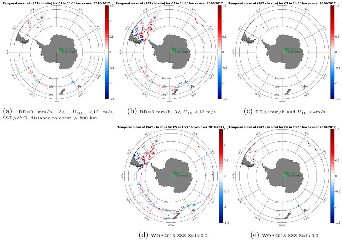
Figure 12: Temporal mean gridded over spatial boxes of size 1°x1° of \Delta SSS (SMOS L3 v2 - Monthly - 0.25 Deg (CATDS-CECOS-IFREMER) - TSG-GOSUD-Sailing-ship) for 5 different subdatasets corresponding to: RR=0 mm/h, 3 < U_{10} < 12 m/s, SST > 5°C, distance to coast > 800 km (a), RR=0 mm/h, 3 < U_{10} < 12 m/s (b), RR > 1mm/h and U_{10} < 4 m/s (c), WOA2013 SSS Std < 0.2 (d), WOA2013 SSS Std > 0.2 (e).
