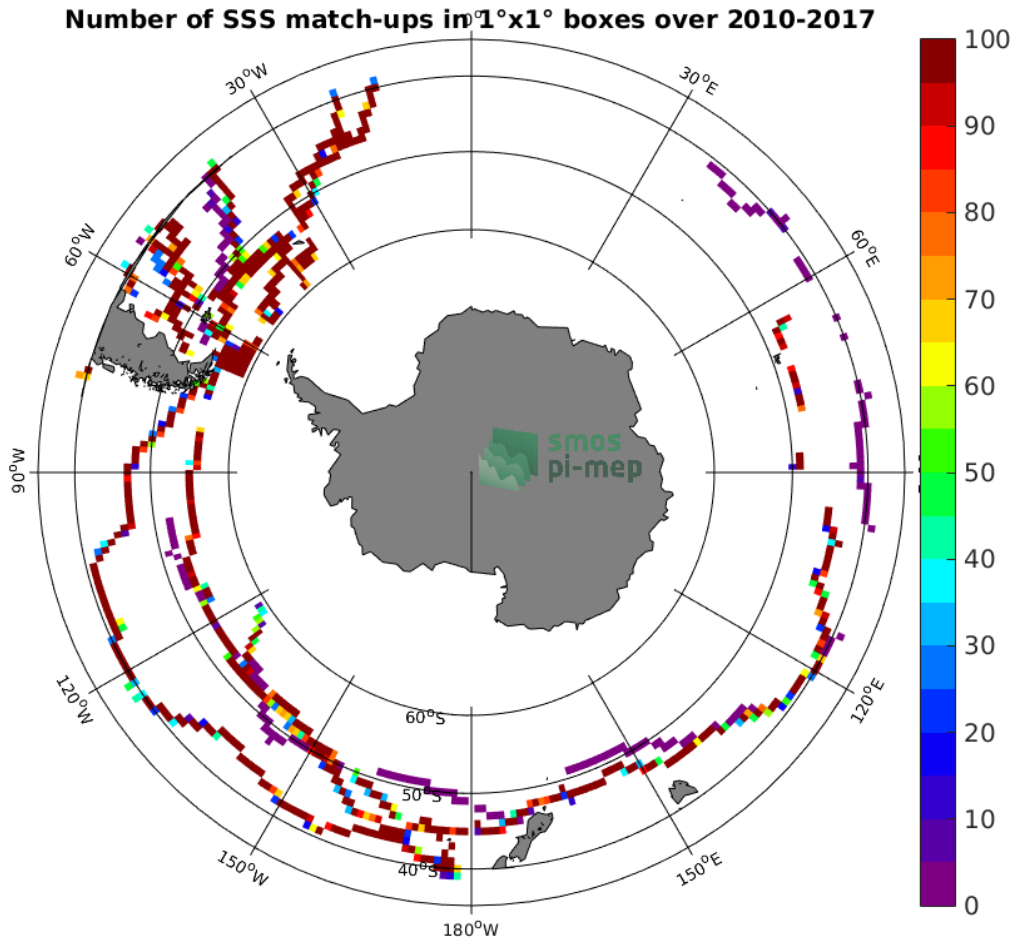
Figure 4: Number of SSS match-ups between TSG-GOSUD-Sailing-ship SSS and the SMOS L3 v2 - Monthly - 0.25 Deg (CATDS-CECOS-IFREMER) SSS product for the Roaring Forties and Furious Fifties Pi-MEP region over 1°x1° boxes and for the full satellite product period.
