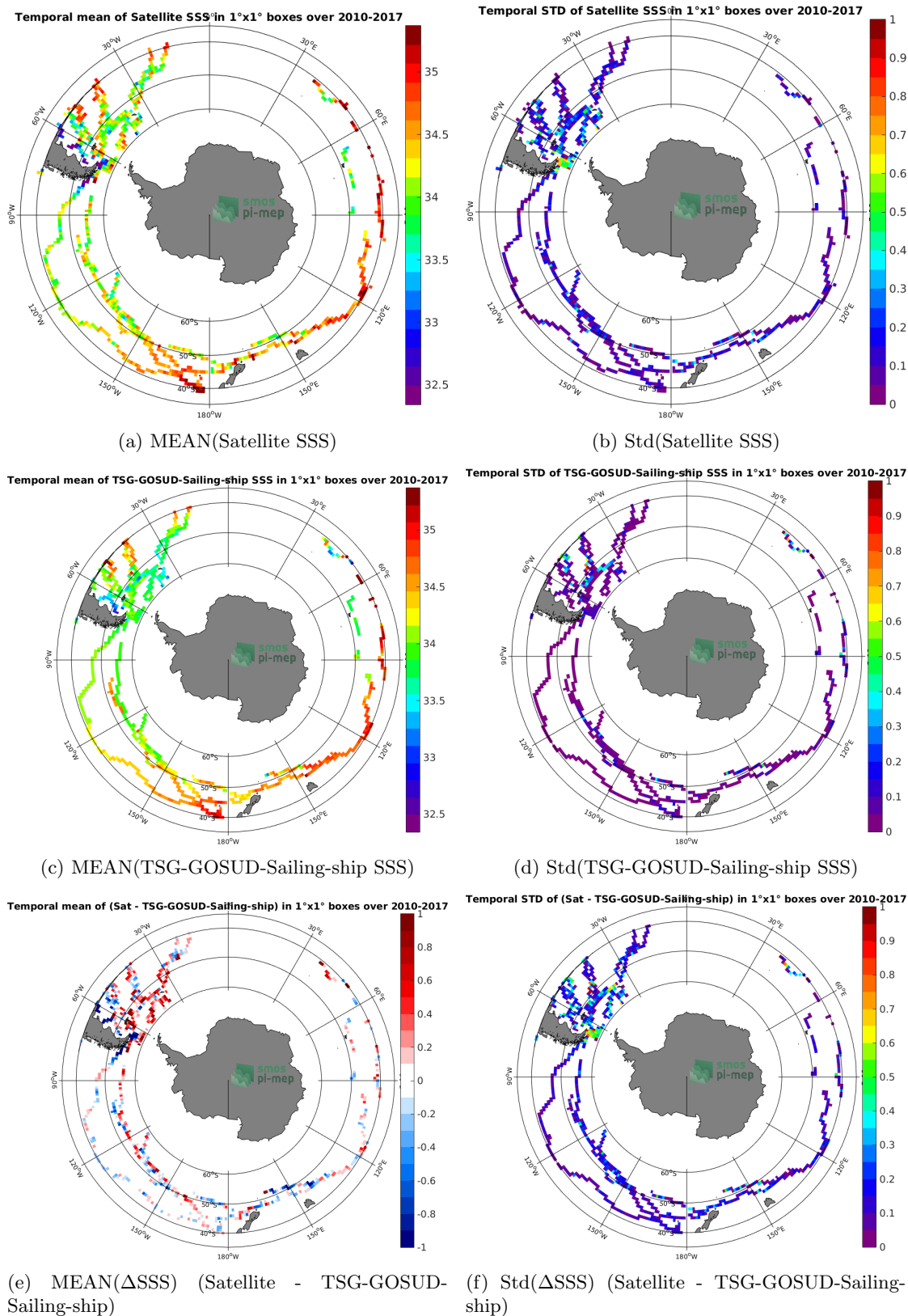
Figure 6: Temporal mean (left) and Std (right) of SSS from SMOS L3 v2 - Monthly - 0.25 Deg (CATDS-CECOS-IFREMER) (top), TSG-GOSUD-Sailing-ship (middle), and of \Delta SSS (Satellite - TSG-GOSUD-Sailing-ship). Only match-up pairs are used to generate these maps.
