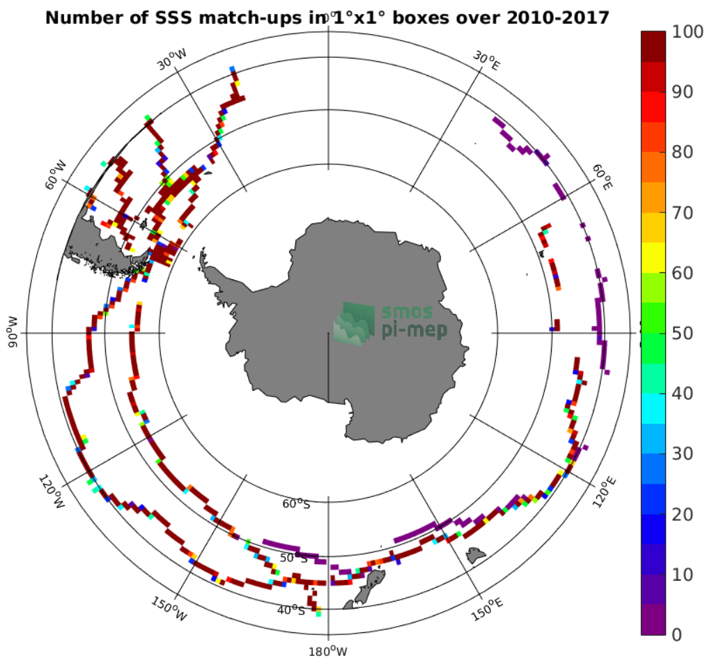
Figure 4: Number of SSS match-ups between TSG-GOSUD-Sailing-ship SSS and the SMOS-L3-CATDS-IFREMER-CECOS-V2-MONTHLY-0.25DEG SSS product for the Roaring Forties and Furious Fifties Pi-MEP region over 1°x1° boxes and for the full satellite product period.
