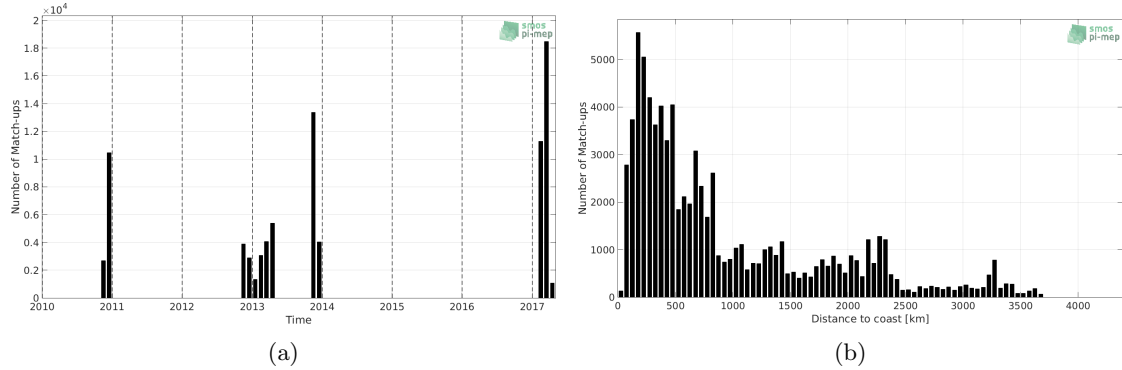
Figure 1: Number of match-ups between TSG-GOSUD-Sailing-ship and SMOS-L3-CATDS-IFREMER-CECOS-V2-MONTHLY-0.25DEG SSS as a function of time (a) and as function of the distance to coast (b) over the Roaring Forties and Furious Fifties Pi-MEP region and for the full satellite product period.
