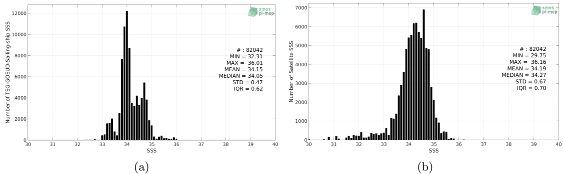
Figure 2: Histograms of SSS from TSG-GOSUD-Sailing-ship (a) and SMOS-L3-CATDS-IFREMER-CECOS-V2-MONTHLY-0.25DEG (b) considering all match-up pairs per bins of 0.1 over the Roaring Forties and Furious Fifties Pi-MEP region and for the full satellite product period.
