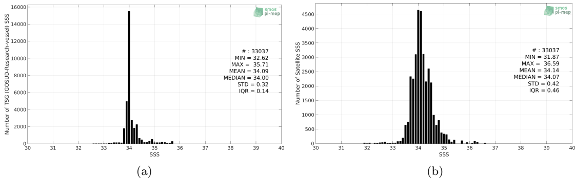
Figure 2: Histograms of SSS from TSG (GOSUD-Research-vessel) (a) and SMOS SSS L3 v2 - Monthly - 0.25 Deg (CATDS-CECOS-IFREMER) (b) considering all match-up pairs per bins of 0.1 over the Roaring Forties and Furious Fifties Pi-MEP region and for the full satellite product period.
