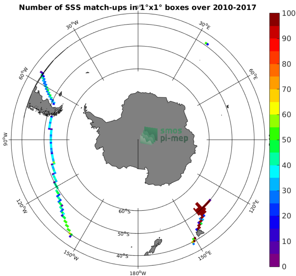
Figure 4: Number of SSS match-ups between TSG (GOSUD-Research-vessel) SSS and the SMOS SSS L3 v2 - Monthly - 0.25 Deg (CATDS-CECOS-IFREMER) SSS product for the Roaring Forties and Furious Fifties Pi-MEP region over 1^\circ \times 1^\circ boxes and for the full satellite product period.
