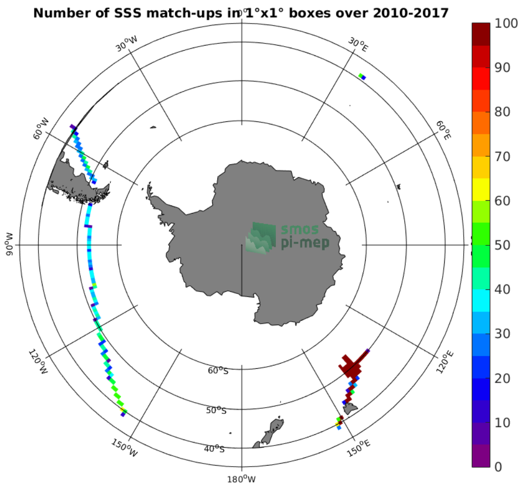
Figure 4: Number of SSS match-ups between TSG-GOSUD-Research-vessel SSS and the SMOS L3 v2 - Monthly - 0.25 Deg (CATDS-CECOS-IFREMER) SSS product for the Roaring Forties and Furious Fifties Pi-MEP region over 1°x1° boxes and for the full satellite product period.
