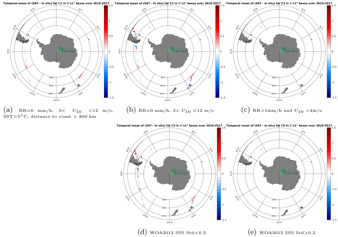
Figure 12: Temporal mean gridded over spatial boxes of size 1°x1° of \Delta SSS (SMOS L3 v2 - Monthly - 0.25 Deg (CATDS-CECOS-IFREMER) - TSG-GOSUD-Research-vessel) for 5 different subdatasets corresponding to:RR=0 mm/h, 3 < U_{10} < 12 m/s, SST>5°C, distance to coast > 800 km (a), RR=0 mm/h, 3 < U_{10} < 12 m/s (b), RR>1mm/h and U_{10} < 4 m/s (c), WOA2013 SSS Std<0.2 (d), WOA2013 SSS Std>0.2 (e).
