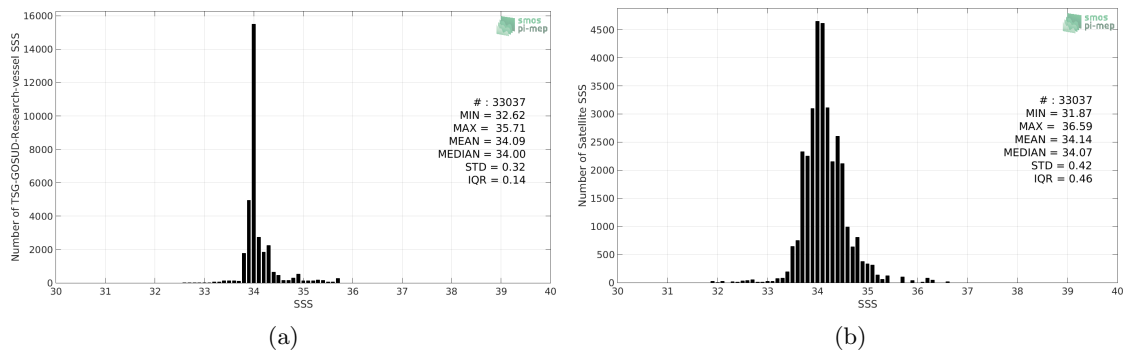
Figure 2: Histograms of SSS from TSG-GOSUD-Research-vessel (a) and SMOS L3 v2 - Monthly - 0.25 Deg (CATDS-CECOS-IFREMER) (b) considering all match-up pairs per bins of 0.1 over the Roaring Forties and Furious Fifties Pi-MEP region and for the full satellite product period.
