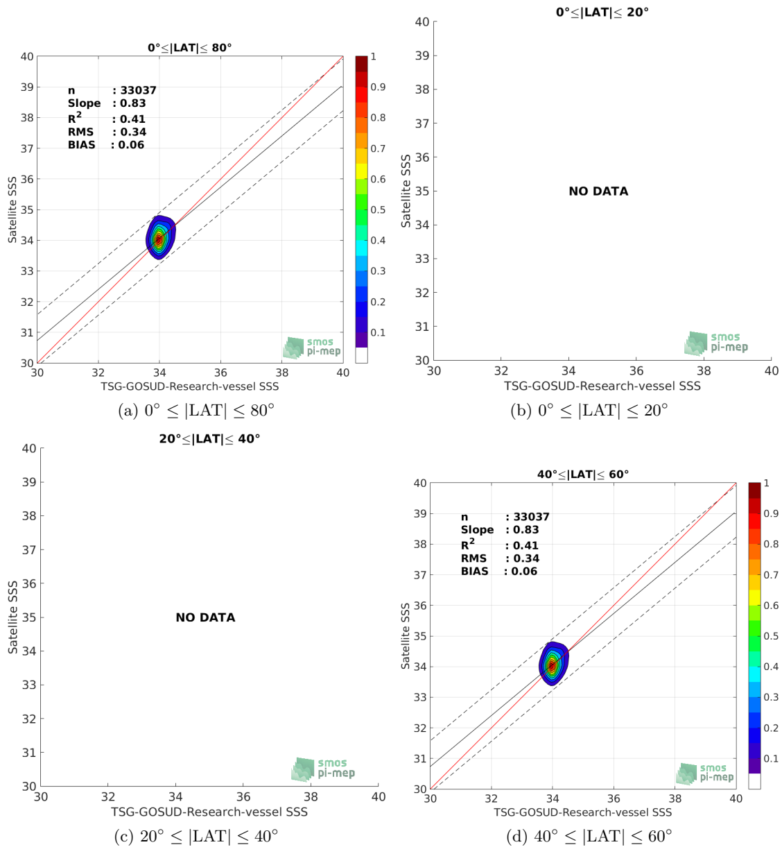
Figure 9: Contour maps of the concentration of SMOS L3 v2 - Monthly - 0.25 Deg (CATDS-CECOS-IFREMER) SSS (y-axis) versus TSG-GOSUD-Research-vessel SSS (x-axis) at match-up pairs for different latitude bands. For each plot, the red line shows x=y . The black thin and dashed lines indicate a linear fit through the data cloud and the \pm 95\% confidence levels, respectively. The number match-up pairs n , the slope and R^2 coefficient of the linear fit, the root mean square (RMS) and the mean bias between satellite and in situ data are indicated for each latitude band in each plots.
