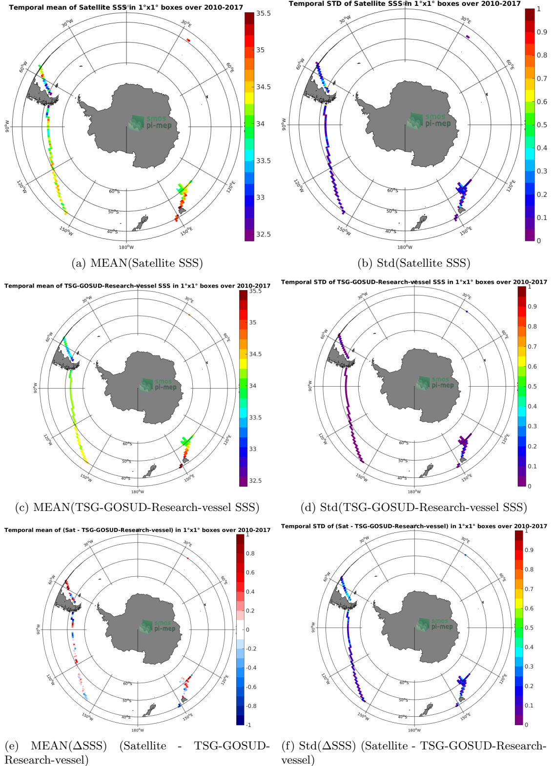
Figure 6: Temporal mean (left) and Std (right) of SSS from SMOS L3 v2 - Monthly - 0.25 Deg (CATDS-CECOS-IFREMER) (top), TSG-GOSUD-Research-vessel (middle), and of \Delta SSS (Satellite - TSG-GOSUD-Research-vessel). Only match-up pairs are used to generate these maps.
