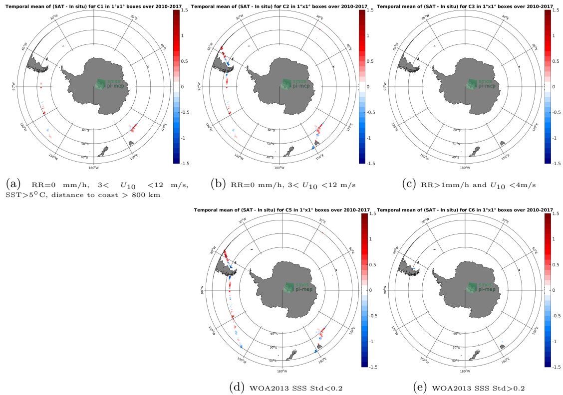
Figure 12: Temporal mean gridded over spatial boxes of size 1^\circ \times 1^\circ of \Delta SSS (SMOS-L3-CATDS-IFREMER-CECOS-V2-MONTHLY-0.25DEG - TSG-GOSUD-Research-vessel) for 5 different subdatasets corresponding to:RR=0 mm/h, 3 < U_{10} < 12 m/s, SST >5^\circ C, distance to coast > 800 km (a), RR=0 mm/h, 3 < U_{10} < 12 m/s (b), RR >1 mm/h and U_{10} < 4 m/s (c), WOA2013 SSS Std <0.2 (d), WOA2013 SSS Std >0.2 (e).
