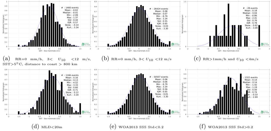
Figure 13: Normalized histogram of \Delta\text{SSS} (SMOS-L3-CATDS-IFREMER-CECOS-V2-MONTHLY-0.25DEG - Sea mammals) for 6 different subdatasets corresponding to: RR=0 mm/h, 3 < U_{10} < 12 m/s, SST>5°C, distance to coast > 800 km (a), RR=0 mm/h, 3 < U_{10} < 12 m/s (b), RR>1mm/h and U_{10} < 4 m/s (c), MLD<20m (d), WOA2013 SSS Std<0.2 (e), WOA2013 SSS Std>0.2 (f).
