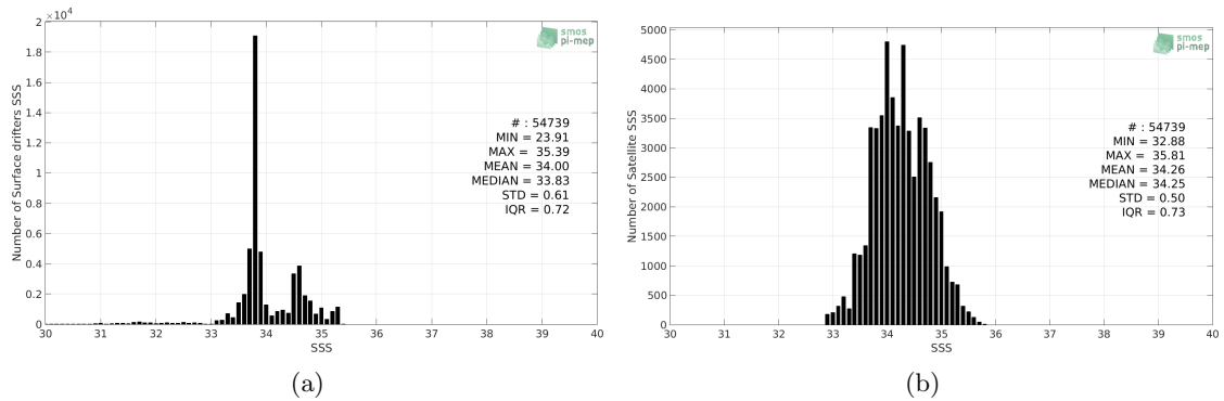
Figure 2: Histograms of SSS from Surface drifters (a) and SMOS SSS L3 v2 - Monthly - 0.25 Deg (CATDS-CECOS-IFREMER) (b) considering all match-up pairs per bins of 0.1 over the Roaring Forties and Furious Fifties Pi-MEP region and for the full satellite product period.
