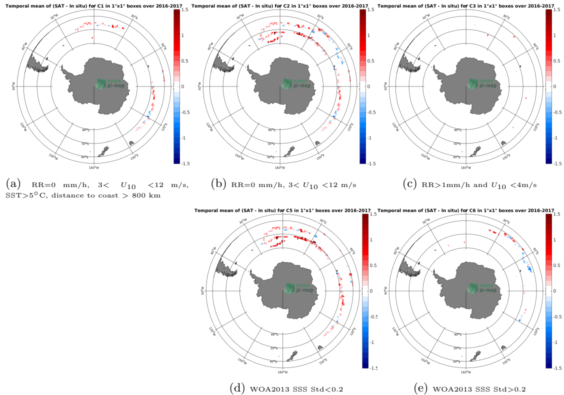
Figure 11: Temporal mean gridded over spatial boxes of size 1^{\circ}\times 1^{\circ} of \Delta\text{SSS} (SMOS SSS L3 v2 - Monthly - 0.25 Deg (CATDS-CECOS-IFREMER) - Surface drifters) for 5 different subdatasets corresponding to:RR=0 mm/h, 3 < U_{10} < 12 m/s, SST >5^{\circ}\text{C} , distance to coast > 800 km (a), RR=0 mm/h, 3 < U_{10} < 12 m/s (b), RR >1 mm/h and U_{10} < 4 m/s (c), WOA2013 SSS Std <0.2 (d), WOA2013 SSS Std >0.2 (e).
