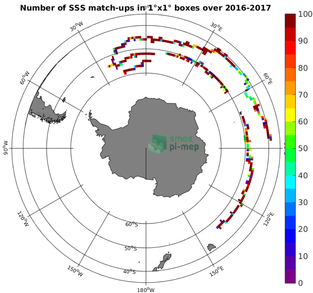
Figure 3: Number of SSS match-ups between Surface drifters SSS and the SMOS SSS L3 v2 - Monthly - 0.25 Deg (CATDS-CECOS-IFREMER) SSS product for the Roaring Forties and Furious Fifties Pi-MEP region over 1°x1° boxes and for the full satellite product period.
