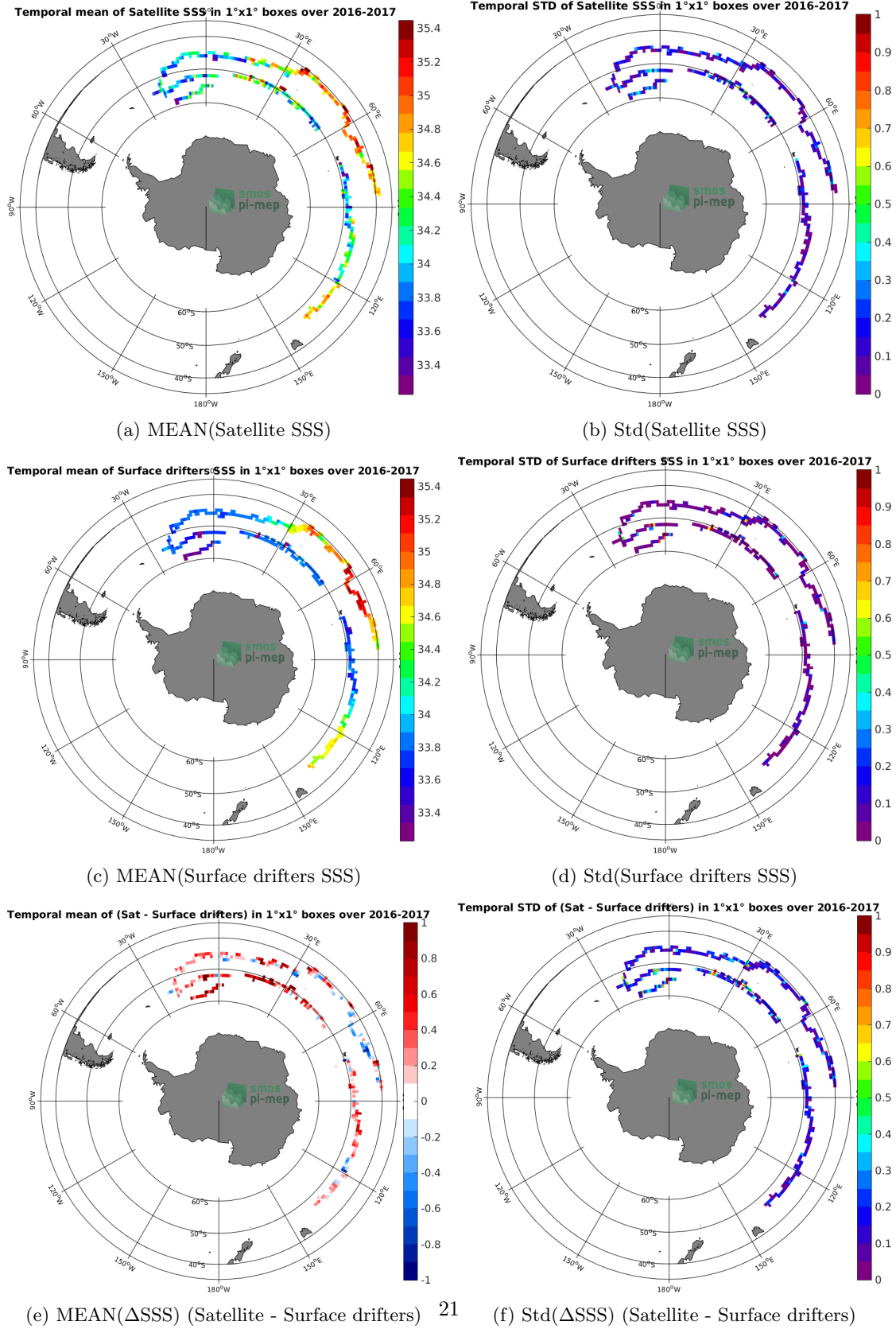
Figure 5: Temporal mean (left) and Std (right) of SSS from SMOS SSS L3 v2 - Monthly - 0.25 Deg (CATDS-CECOS-IFREMER) (top), Surface drifters (middle), and of \Delta SSS (Satellite - Surface drifters). Only match-up pairs are used to generate these maps.
