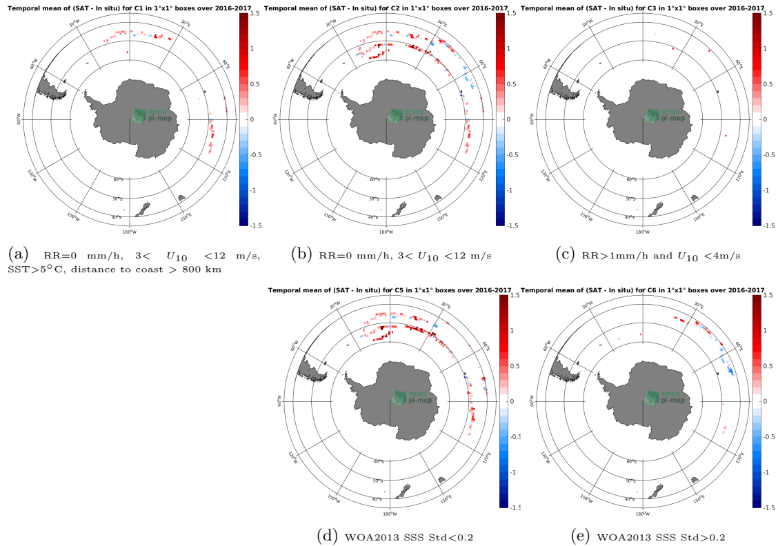
Figure 11: Temporal mean gridded over spatial boxes of size 1^{\circ}\times 1^{\circ} of \Delta\text{SSS} (SMOS L3 v2 - Monthly - 0.25 Deg (CATDS-CECOS-IFREMER) - Surface drifters) for 5 different subdatasets corresponding to:RR=0 mm/h, 3 < U_{10} < 12 m/s, SST >5^{\circ}\text{C} , distance to coast > 800 km (a), RR=0 mm/h, 3 < U_{10} < 12 m/s (b), RR >1 mm/h and U_{10} < 4 m/s (c), WOA2013 SSS Std <0.2 (d), WOA2013 SSS Std >0.2 (e).
