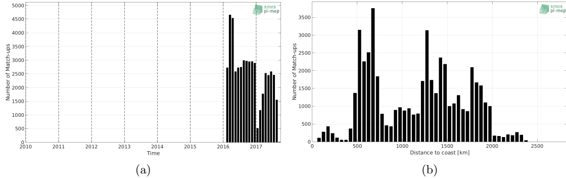
Figure 1: Number of match-ups between Surface drifters and SMOS L3 v2 - Monthly - 0.25 Deg (CATDS-CECOS-IFREMER) SSS as a function of time (a) and as function of the distance to coast (b) over the Roaring Forties and Furious Fifties Pi-MEP region and for the full satellite product period.
