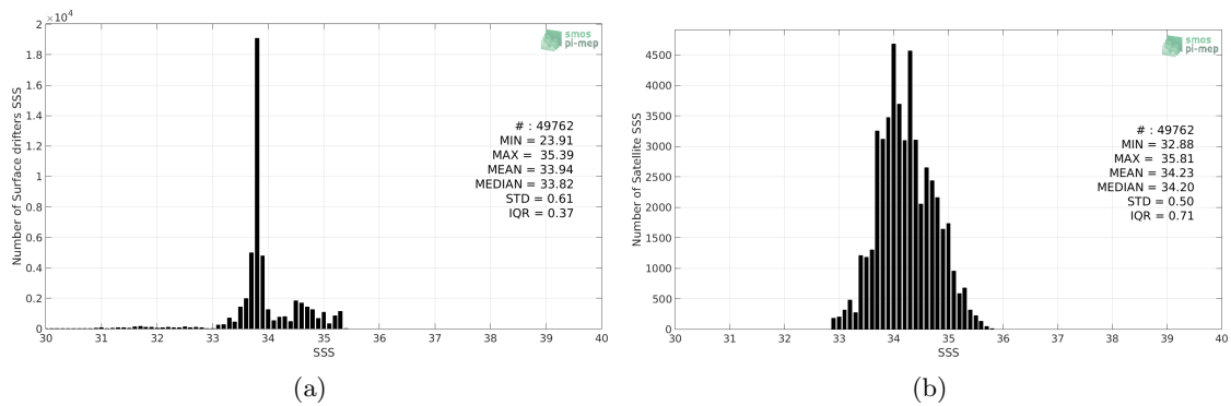
Figure 2: Histograms of SSS from Surface drifters (a) and SMOS L3 v2 - Monthly - 0.25 Deg (CATDS-CECOS-IFREMER) (b) considering all match-up pairs per bins of 0.1 over the Roaring Forties and Furious Fifties Pi-MEP region and for the full satellite product period.
