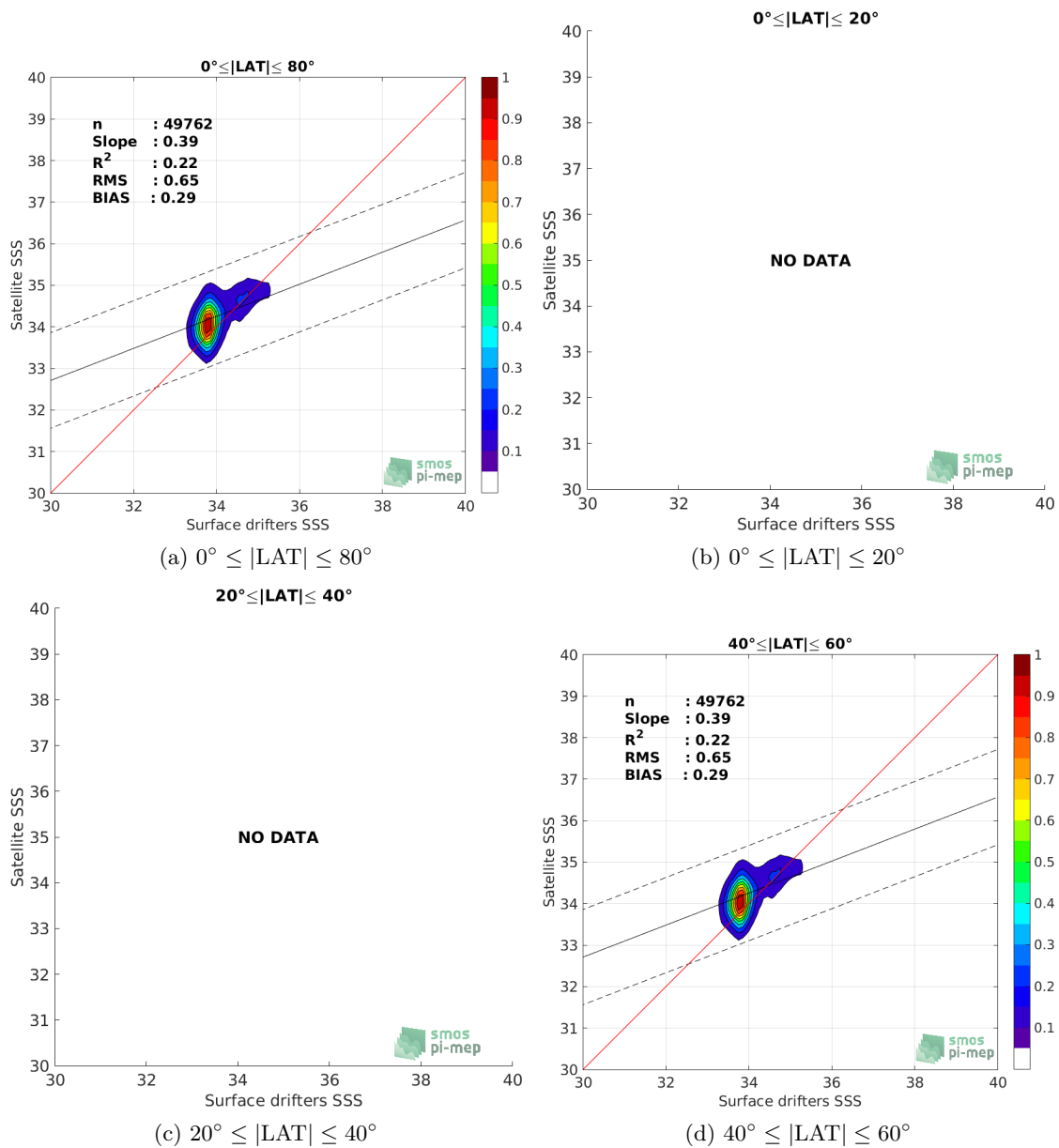
Figure 8: Contour maps of the concentration of SMOS L3 v2 - Monthly - 0.25 Deg (CATDS-CECOS-IFREMER) SSS (y-axis) versus Surface drifters SSS (x-axis) at match-up pairs for different latitude bands. For each plot, the red line shows x=y . The black thin and dashed lines indicate a linear fit through the data cloud and the \pm 95\% confidence levels, respectively. The number match-up pairs n , the slope and R^2 coefficient of the linear fit, the root mean square (RMS) and the mean bias between satellite and in situ data are indicated for each latitude band in each plots.
