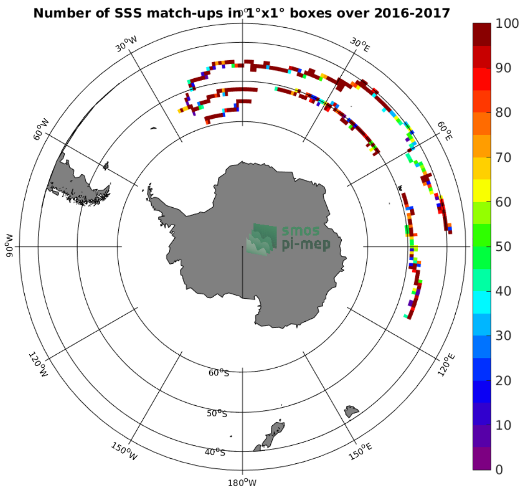
Figure 3: Number of SSS match-ups between Surface drifters SSS and the SMOS L3 v2 - Monthly - 0.25 Deg (CATDS-CECOS-IFREMER) SSS product for the Roaring Forties and Furious Fifties Pi-MEP region over 1^\circ \times 1^\circ boxes and for the full satellite product period.
