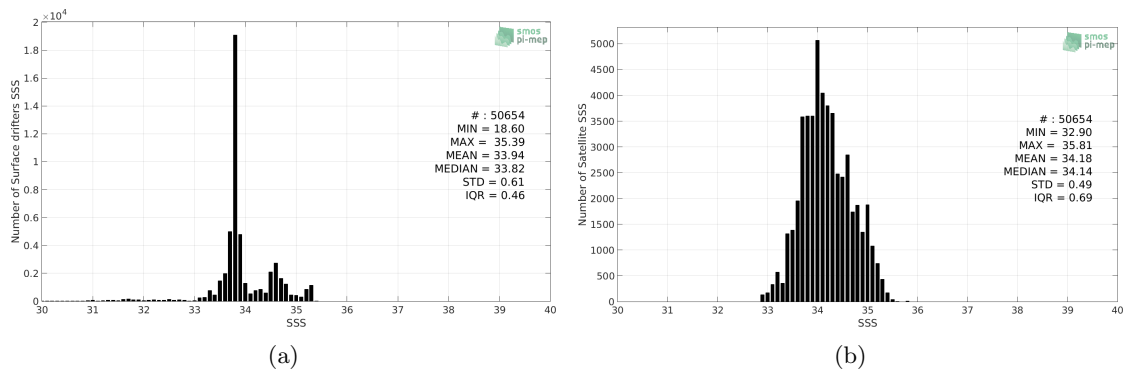
Figure 2: Histograms of SSS from Surface drifters (a) and SMOS-L3-CATDS-IFREMER-CECOS-V2-MONTHLY-0.25DEG (b) considering all match-up pairs per bins of 0.1 over the Roaring Forties and Furious Fifties Pi-MEP region and for the full satellite product period.
