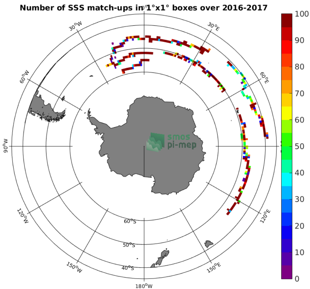
Figure 3: Number of SSS match-ups between Surface drifters SSS and the SMOS-L3-CATDS-IFREMER-CECOS-V2-MONTHLY-0.25DEG SSS product for the Roaring Forties and Furious Fifties Pi-MEP region over 1°x1° boxes and for the full satellite product period.
