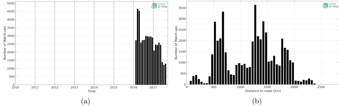
Figure 1: Number of match-ups between Surface drifters and SMOS-L3-CATDS-IFREMER-CECOS-V2-MONTHLY-0.25DEG SSS as a function of time (a) and as function of the distance to coast (b) over the Roaring Forties and Furious Fifties Pi-MEP region and for the full satellite product period.
