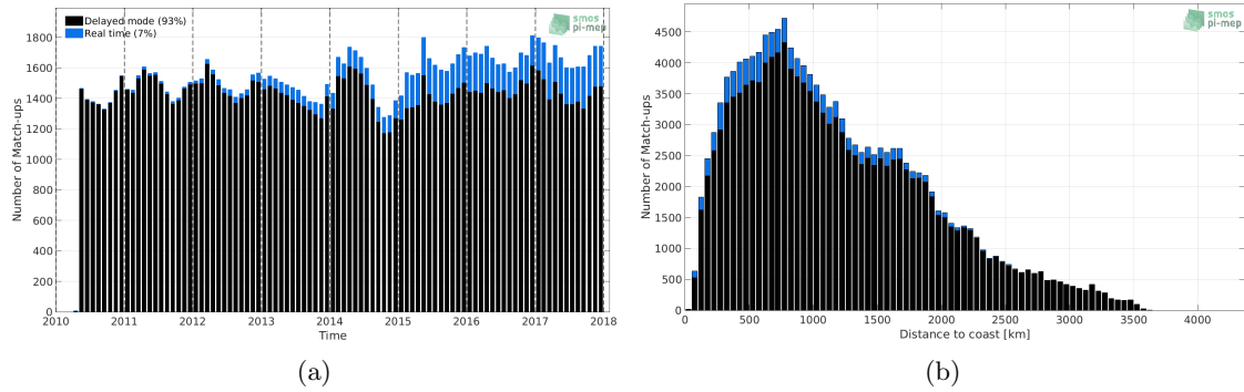
Figure 1: Number of match-ups between Argo and SMOS SSS L3 v2 - Monthly - 0.25 Deg (CATDS-CECOS-IFREMER) SSS as a function of time (a) and as function of the distance to coast (b) over the Roaring Forties and Furious Fifties Pi-MEP region and for the full satellite product period.
