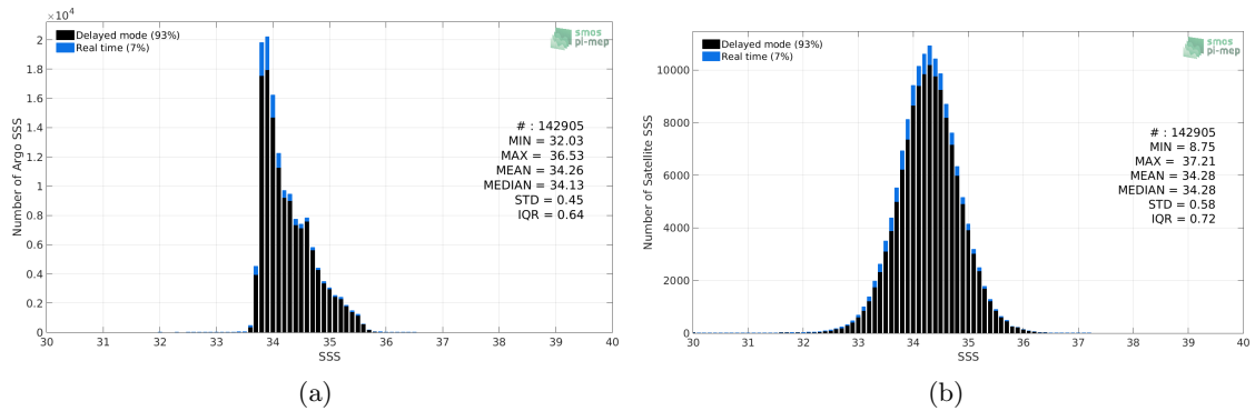
Figure 2: Histograms of SSS from Argo (a) and SMOS SSS L3 v2 - Monthly - 0.25 Deg (CATDS-CECOS-IFREMER) (b) considering all match-up pairs per bins of 0.1 over the Roaring Forties and Furious Fifties Pi-MEP region and for the full satellite product period.
