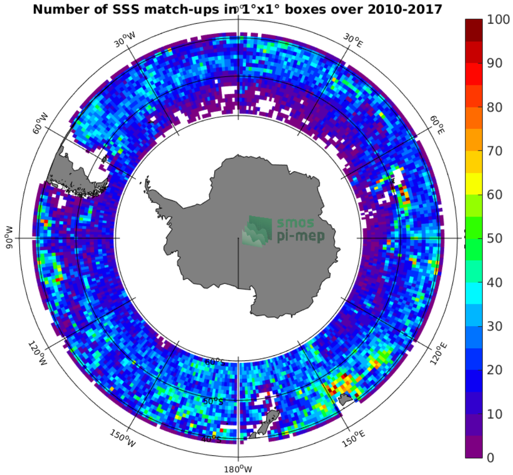
Figure 4: Number of SSS match-ups between Argo SSS and the SMOS SSS L3 v2 - Monthly - 0.25 Deg (CATDS-CECOS-IFREMER) SSS product for the Roaring Forties and Furious Fifties Pi-MEP region over 1°x1° boxes and for the full satellite product period.
