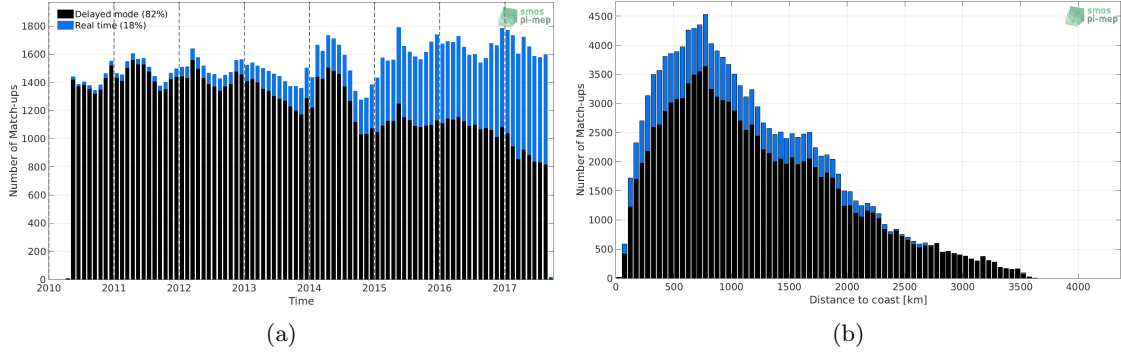
Figure 1: Number of match-ups between Argo and SMOS-L3-CATDS-IFREMER-CECOS-V2-MONTHLY-0.25DEG SSS as a function of time (a) and as function of the distance to coast (b) over the Roaring Forties and Furious Fifties Pi-MEP region and for the full satellite product period.
