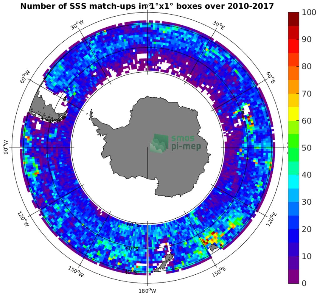
Figure 4: Number of SSS match-ups between Argo SSS and the SMOS-L3-CATDS-IFREMER-CECOS-V2-MONTHLY-0.25DEG SSS product for the Roaring Forties and Furious Fifties Pi-MEP region over 1°x1° boxes and for the full satellite product period.
