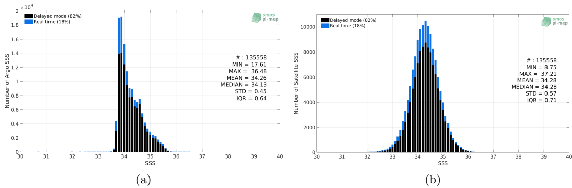
Figure 2: Histograms of SSS from Argo (a) and SMOS-L3-CATDS-IFREMER-CECOS-V2-MONTHLY-0.25DEG (b) considering all match-up pairs per bins of 0.1 over the Roaring Forties and Furious Fifties Pi-MEP region and for the full satellite product period.
