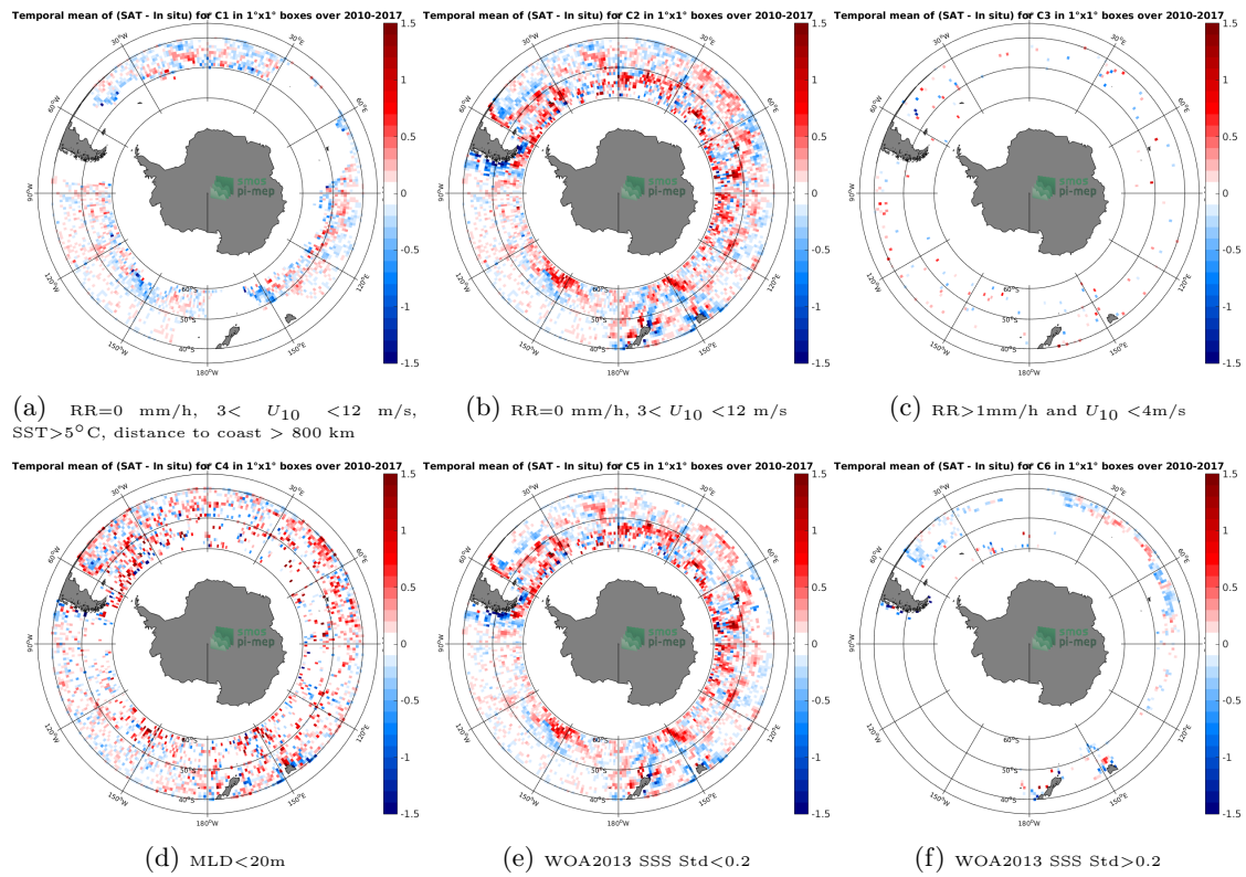
Figure 12: Temporal mean gridded over spatial boxes of size 1^\circ \times 1^\circ of \Delta SSS (SMOS-L3-CATDS-IFREMER-CECOS-V2-MONTHLY-0.25DEG - Argo) for 6 different subdatasets corresponding to:RR=0 mm/h, 3 < U_{10} < 12 m/s, SST >5^\circ C, distance to coast > 800 km (a), RR=0 mm/h, 3 < U_{10} < 12 m/s (b), RR >1 mm/h and U_{10} < 4 m/s (c),MLD <20 m (d),WOA2013 SSS Std <0.2 (e),WOA2013 SSS Std >0.2 (f).
