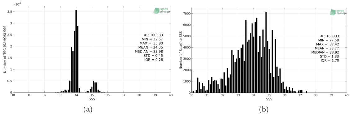
Figure 2: Histograms of SSS from TSG (SAMOS) (a) and SMOS SSS L3 v2 - Daily - 0.5 Deg (CATDS-CECOS-IFREMER) (b) considering all match-up pairs per bins of 0.1 over the Roaring Forties and Furious Fifties Pi-MEP region and for the full satellite product period.
