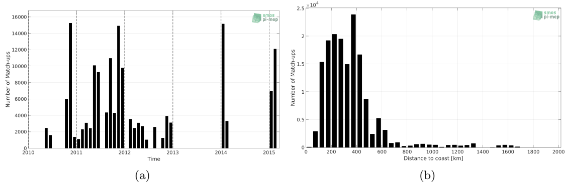
Figure 1: Number of match-ups between TSG (SAMOS) and SMOS SSS L3 v2 - Daily - 0.5 Deg (CATDS-CECOS-IFREMER) SSS as a function of time (a) and as function of the distance to coast (b) over the Roaring Forties and Furious Fifties Pi-MEP region and for the full satellite product period.
