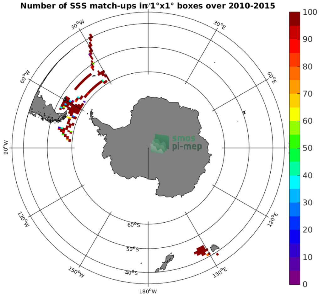
Figure 4: Number of SSS match-ups between TSG (SAMOS) SSS and the SMOS SSS L3 v2 - Daily - 0.5 Deg (CATDS-CECOS-IFREMER) SSS product for the Roaring Forties and Furious Fifties Pi-MEP region over 1°x1° boxes and for the full satellite product period.
